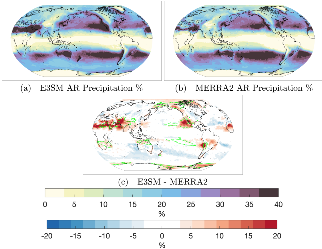
Figure 6. The fraction of annual precipitation attributed to ARs for each grid cell for (a) E3SM and (b) MERRA2. The difference (E3SM minus MERRA2) is shown in (c). The colorbar on the top (bottom) corresponds to the absolute (difference) percentages. Contour lines in (c) indicate the 1.5 % positive AR frequency biases from Fig. 1c.
