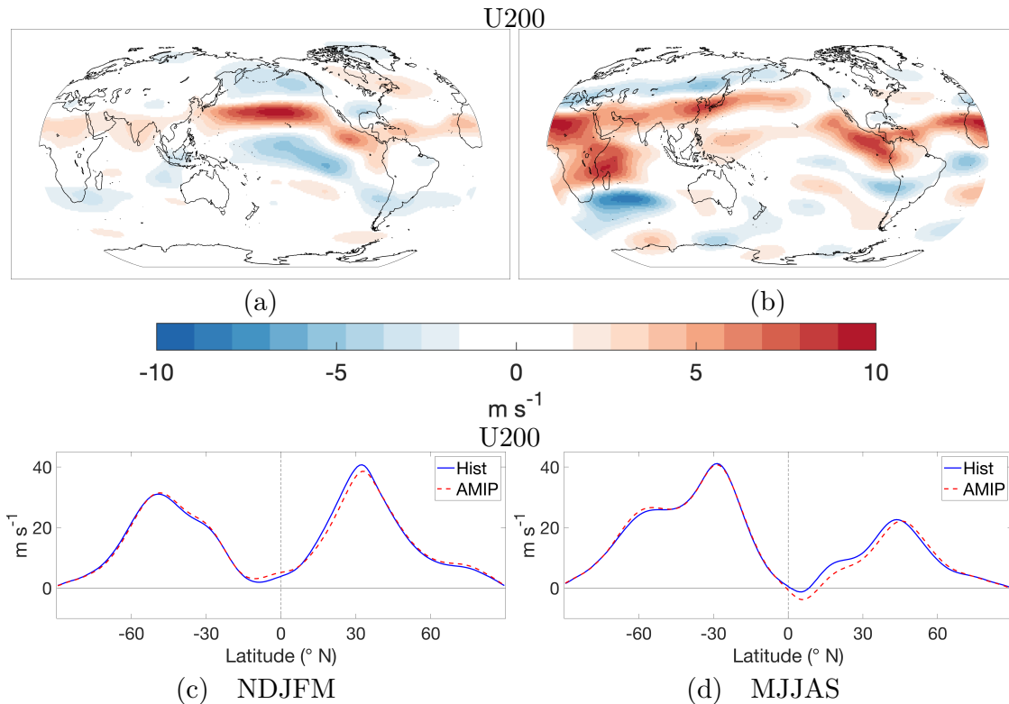
Figure 9. Seasonal differences between E3SM fully-coupled and AMIP: zonal wind at 200 hPa (top row) and zonal means over the Pacific and Atlantic basins (100-360° E) of zonal wind at 200 hPa (bottom row).
