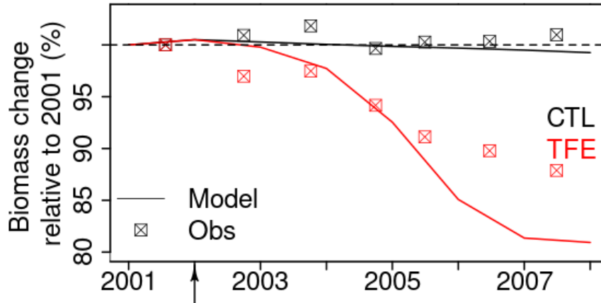
1070 Figure 9 Tree biomass change simulated by model after mortality being triggered. The squares in the plot denote the observation. Biomass change relative to 2001 is calculated by dividing biomass during 2002-2008 by biomass in 2001.
