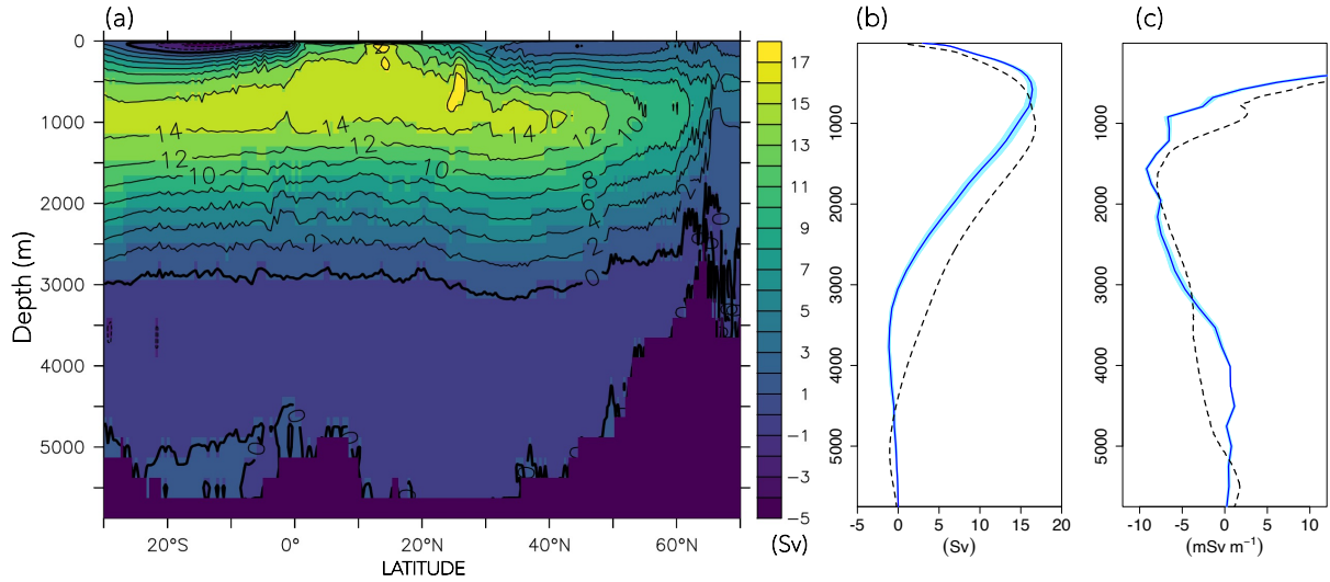
Figure 5. Atlantic meridional overturning stream function climatology over 2004–2014 of the Hist simulations. (a) Latitude–depth structure, (b) vertical profile at 26.5° N, and (c) z derivative of AMOC at 26.5° N. Blue lines and the shaded areas are modelled results, and dashed black lines are observational values from the RAPID array (McCarthy et al., 2015).
