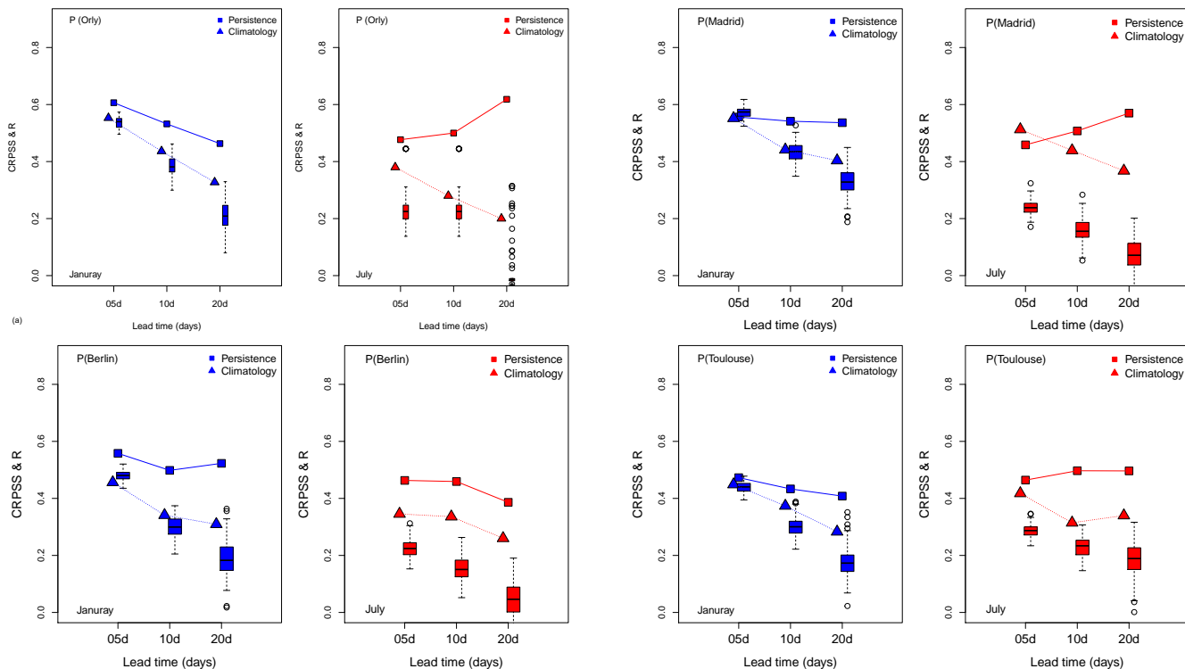
Figure 4. Skill scores for the precipitation of Orly, Madrid, Berlin and Toulouse for lead times of 5, 10, 20 days for January (blue) and July (red) for analogs computed from reanalyses of (a) NCEP and (b) ERA5. Squares indicate CRPSS where the Persistence is the baseline, triangles indicates CRPSS where the climatology is the reference, and boxplots indicates the probability distribution of correlation between observation and the median of 100 simulations for all days. The boxplot upper whisker is: \min\{1.5(q_{75} - q_{50}) + q_{50}, \max(CRPS)\} . The boxplot lower whisker is: \max\{q_{50} - 1.5(q_{75} - q_{50}), \min(CRPS)\} .
