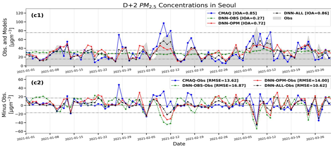
365 Figure 7. Time series of PM 2.5 concentrations from observations and predictions using the CMAQ, DNN-OBS, DNN-OPM and DNN-ALL. 7 (a1) to (c1) depict the time series of predictions and observations and (a2) to (c2) depict the differences between the predictions and observations (predictions minus observations). In 7 (a1) to (c1), each of the dashed lines represents values of 15.5 \mu\text{g}\text{m}^{-3} , 35.5 \mu\text{g}\text{m}^{-3} , 75.5 \mu\text{g}\text{m}^{-3} , and average value of observation (27 \mu\text{g}\text{m}^{-3} ). In 7 (a2) to (c2), the dashed lines represent the standard deviation of observation PM 2.5 as negative and positive.
