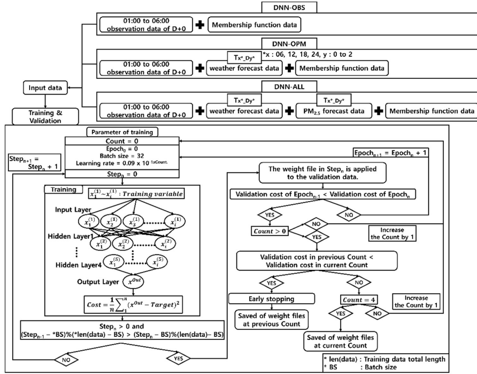
220 Figure 4. Structure of DNN model training process.
