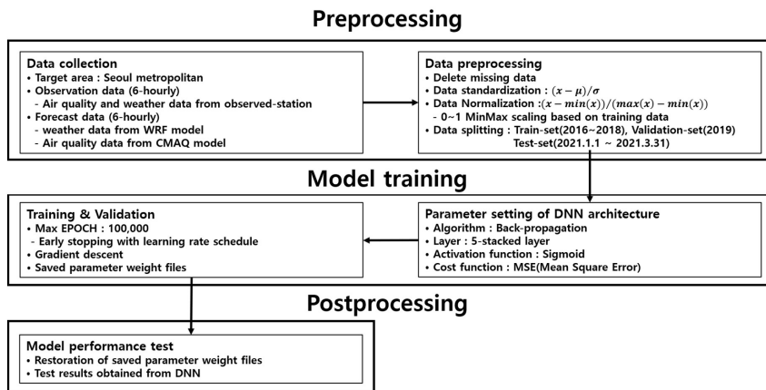
Figure 1. Flowchart of the PM 2.5 forecasting system based on the DNN algorithm.
