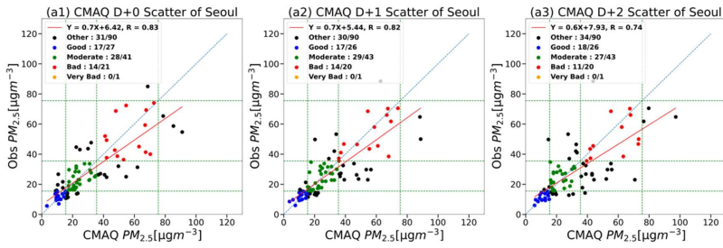
(a) Scatter plot of the CMAQ model for D+0 to D+2
