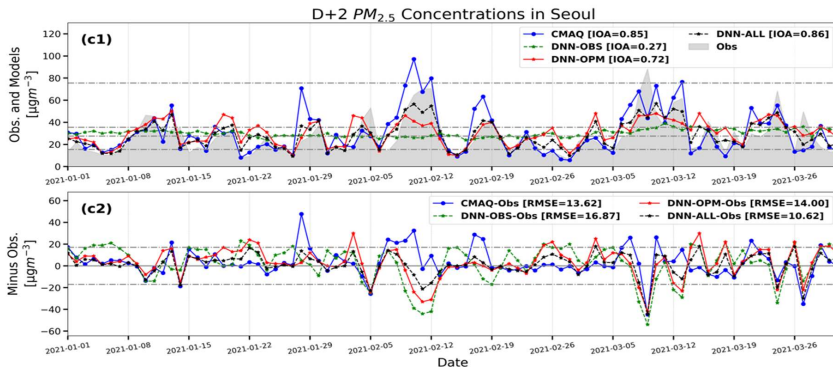
Figure 7. Time series of PM_{2.5} concentrations from observations and predictions using the CMAQ, DNN-OBS, DNN-OPM and DNN-ALL. 7 (a1) to (c1) depict the time series of predictions and observations and (a2) to (c2) depict the differences between the predictions and observations (predictions minus observations). In 7 (a1) to (c1), each of the dashed lines represents values of 15.5 \mu g m^{-3} , 35.5 \mu g m^{-3} , 75.5 \mu g m^{-3} , and average value of observation ( 27 \mu g m^{-3} ). In 7 (a2) to (c2), the dashed lines represent the standard deviation of observation PM_{2.5} as negative and positive.
