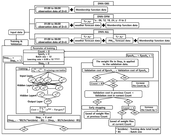
Figure 4. Structure of DNN model training process.
