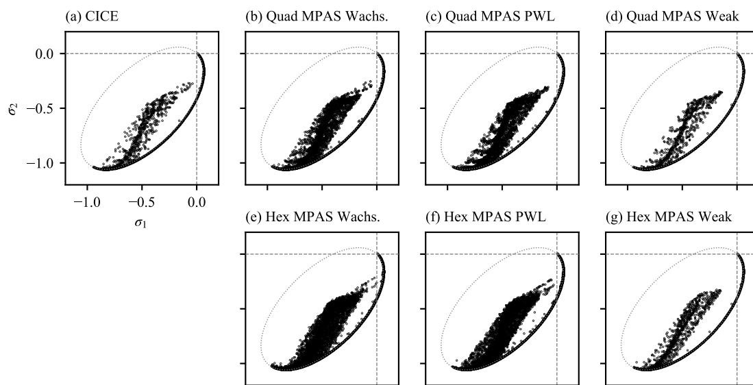
Figure 14. Principal stress components for the square domain test case and (dotted) the EVP yield curve. (a): CICE. (b-d): MPAS-Seaice on a quadrilateral mesh and using the Wachspress variational, PWL variational and weak schemes respectively. (e-g): MPAS-Seaice on a hexagonal mesh and using the Wachspress variational, PWL variational and weak schemes respectively.
