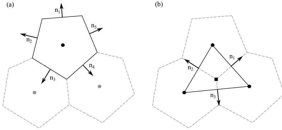
Figure 3. Contour integration lines used by the weak stress divergence operator scheme. (a): Strain rate at cell centers ( circle ) are calculated from line integrals around primary mesh cells ( solid line ). (b): Stress divergence at cell vertices ( square ) are calculated from line integrals around the dual mesh cells ( solid line ). Directions of normal vectors used in the integrals are shown for both figures.
