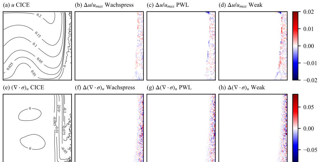
Figure 12. (a): u velocity component of CICE for the square domain test case using a quadrilateral mesh. (b,c,d): Difference ( \Delta u / u_{max} ) between the u component of MPAS-Seaice and CICE in the square domain test case for the MPAS-Seaice Wachspres variational, PWL variational and weak schemes respectively and using a quadrilateral mesh. (e-h): As (a-d) but for the u component of the divergence of internal ice stress.
