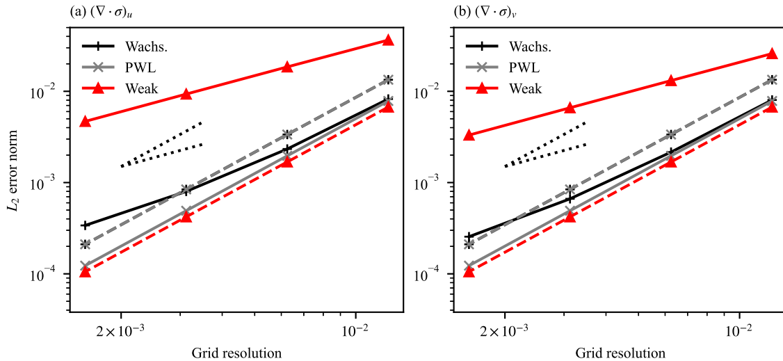
Figure 6. Scaling of L_2 error norm against grid resolution for the model calculation of the (a) u , and (b) v components of stress divergence from an analytical strain rate tensor field for a planar test case with a regular mesh. Grid resolution is the mean distance between cell centers. Solid lines denote hexagonal cell meshes, whereas dashed lines signify square cell meshes. Ideal first and second-order scaling gradients are also shown as dotted lines.
