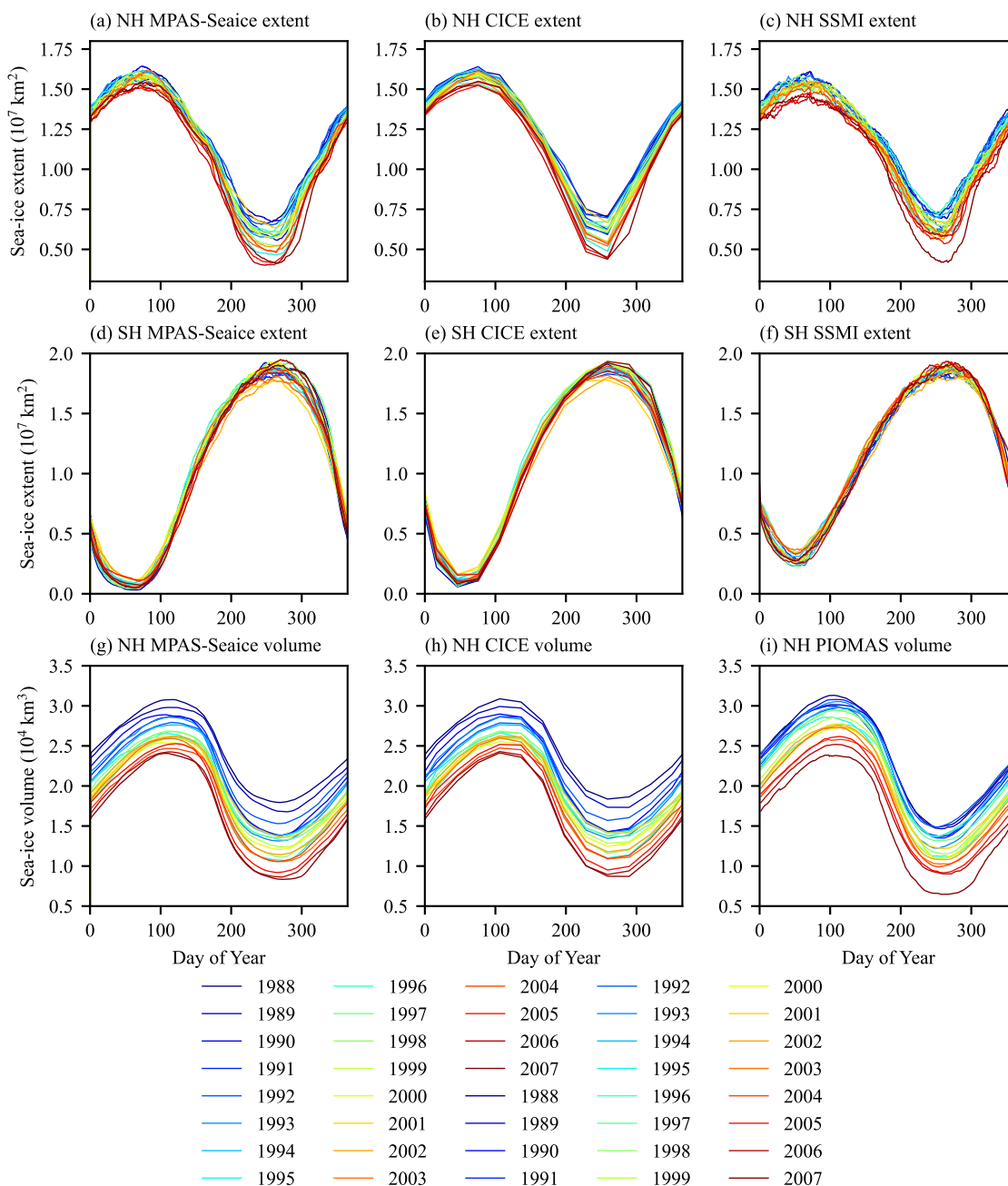
Figure 18. Sea-ice extent (area with ice concentration greater than 15%) by year for the Northern (a-c) and Southern (d-f) Hemispheres, for MPAS-Sealice (a,d), CICE (b,e) and SSMI satellite observations (c,f). Northern Hemisphere total sea-ice volume by year for (g) MPAS-Sealice, (h) CICE, and (i) PIOMAS.
