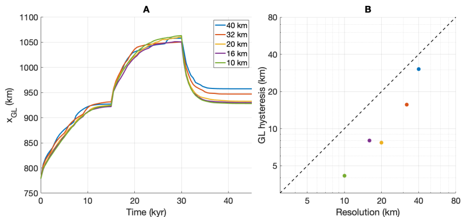
Figure 7. panel A: Grounding-line position over time in the MISIP experiment at different resolutions. The first 25 kyr show the initialisation phase. Panel B: grounding-line hysteresis (defined as the difference in grounding-line positions between t = 15 kyr and t = 45 kyr) versus model resolution.
