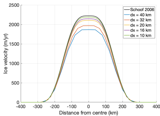
Figure 3: Cross-slope transect of the downslope velocity in the Schoof (2006) ice-stream experiment at different resolutions.
