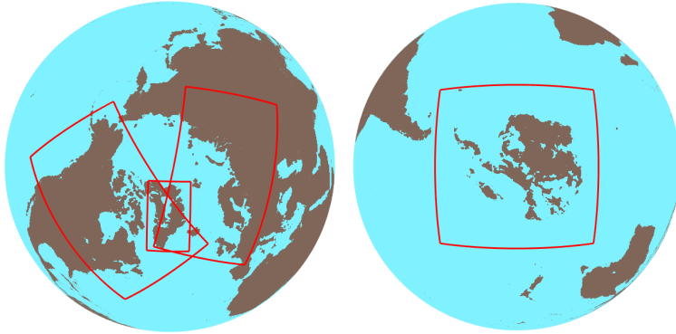
Figure 1: The four model regions of IMA-ICE. No ice is shown; brown (blue) indicates bedrock above (below) present-day sea level.
