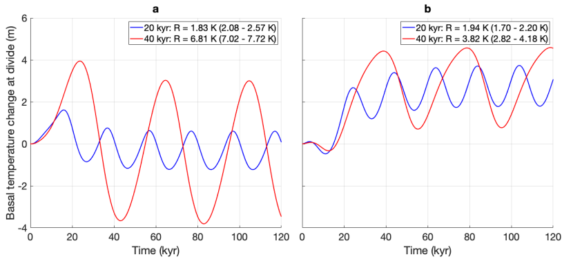
5 Figure 5: Ice temperature at the base of the ice divide, relative to the pressure melting point, over time for the “glacial cycle” experiments from the first EISMINT intercomparison exercise, with a moving margin (panel a) and a fixed margin (panel b). The legends list the simulated glacial-interglacial difference R for the last cycle, with the range of numbers reported by Huybrechts et al. (1996) listed between brackets for comparison.
