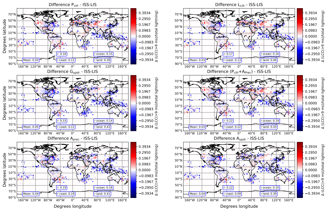
Figure 10. Difference between the observed and the simulated ratio of LCC(>9 ms)-lightning to total lightning density March, April and May using different lightning parameterizations. Positive values indicate that the model overestimates the ratio. The calculated global, land and ocean spatial correlation coefficients r are included.
