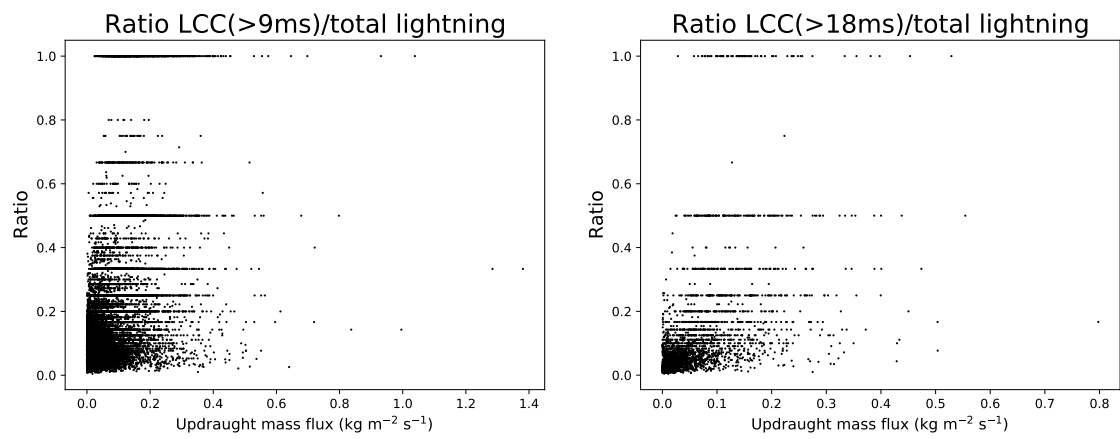
Figure 2. Ratios of (left panel) LCC(>9 ms)- and (right panel) LCC(>18 ms)-lightning to total lightning flashes versus the updraught mass flux extracted from ERA5 1-hourly averaged 2.75^\circ \times 2.75^\circ grid cells for lightning reported by ISS-LIS globally between March 2017 and March 2018.
