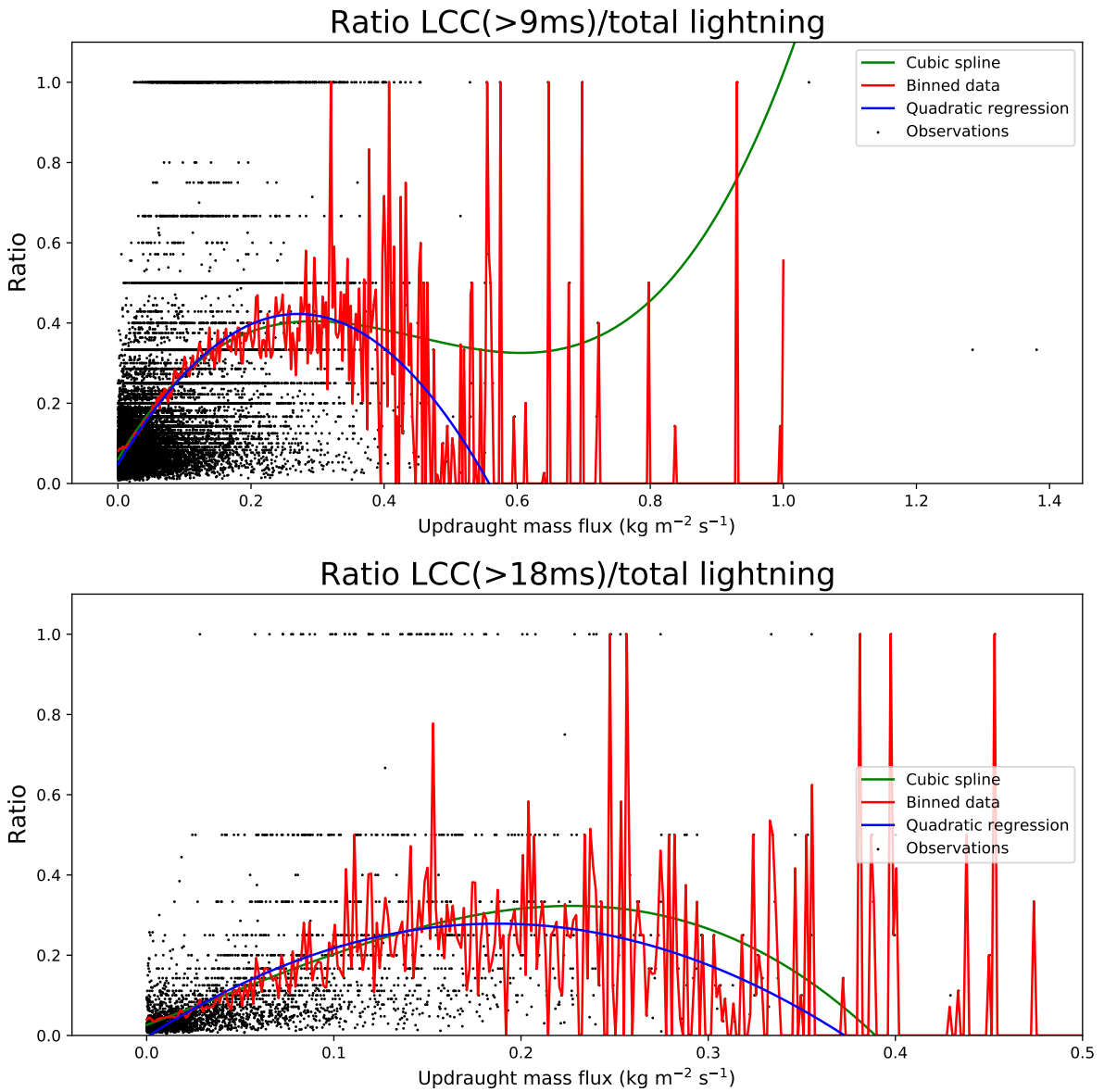
Figure 3. Ratios of (upper panel) LCC(>9 ms)- and (lower panel) LCC(>18 ms)-lightning to total lightning flashes versus the updraught mass flux as in Fig. 2. We have added a cubic smoothing spline (green line), a quadratic fitting (blue line) and a binning (red line) to the data as described in the text.
