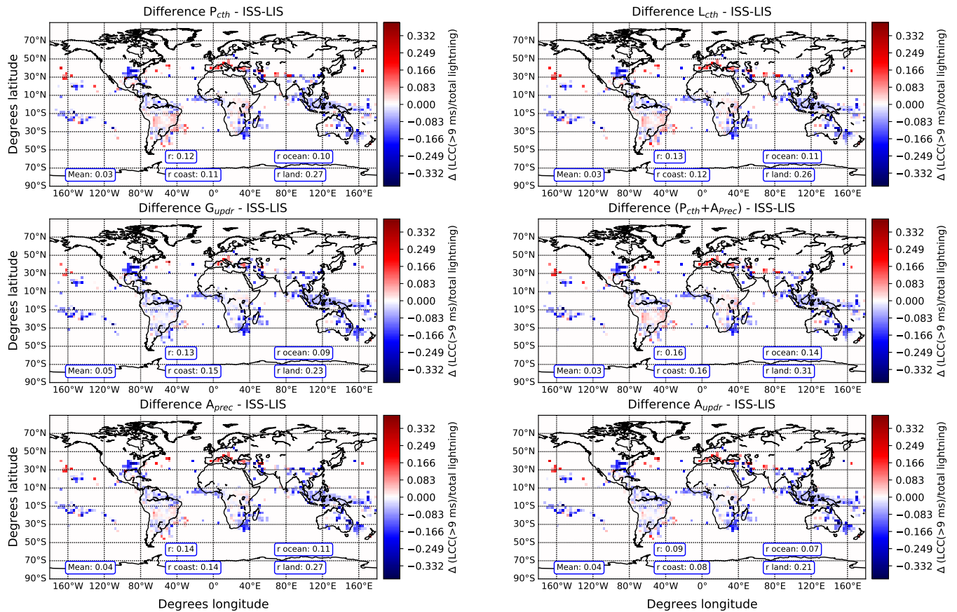
Figure 9. Difference between the observed and the simulated ratio of LCC(>9 ms)-lightning to total lightning density December, January and February using different lightning parameterizations. Positive values indicate that the model overestimates the ratio. The calculated global, land and ocean spatial correlation coefficients r are included.
