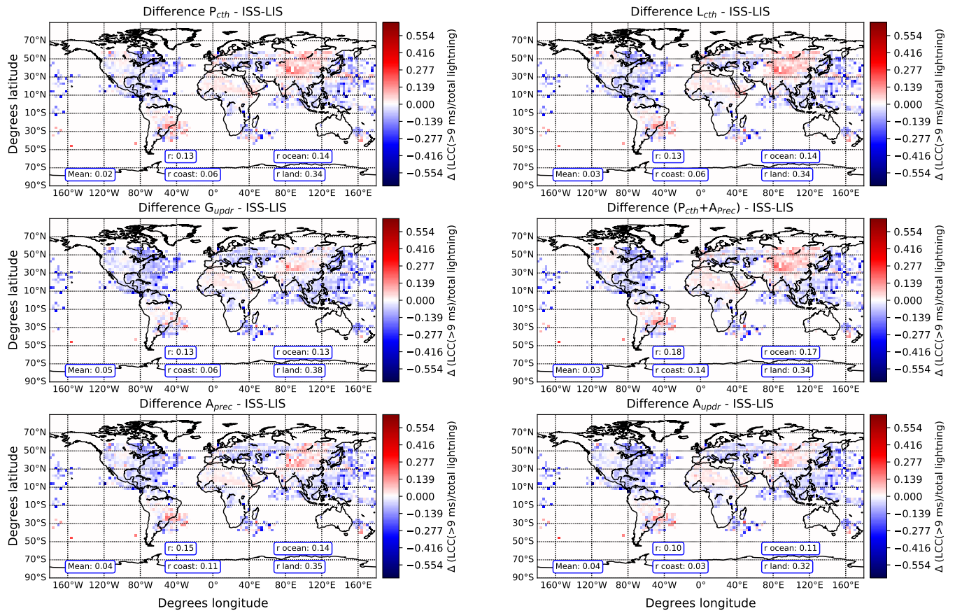
Figure 11. Difference between the observed and the simulated ratio of LCC(>9 ms)-lightning to total lightning density June, July and August using different lightning parameterizations. Positive values indicate that the model overestimates the ratio. The calculated global, land and ocean spatial correlation coefficients r are included.
