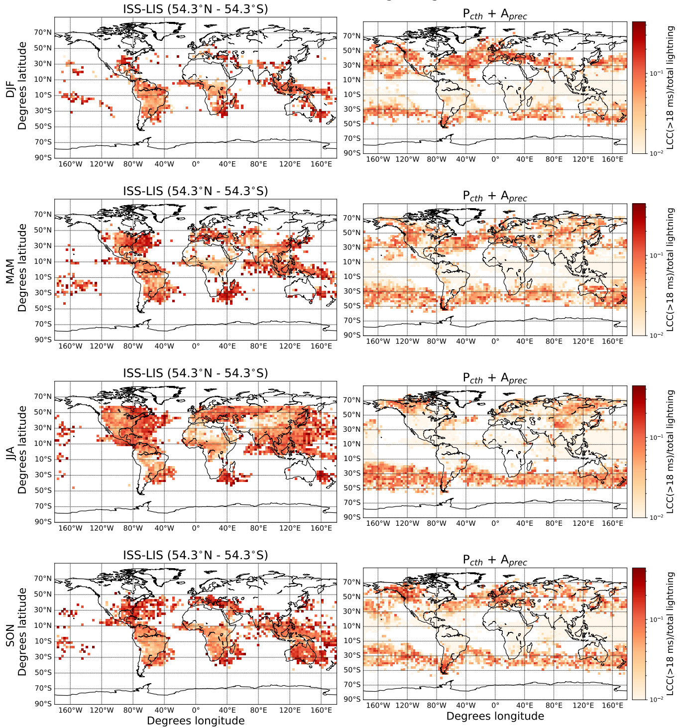
Figure 8. Seasonal observed (left panels) and simulated (right of panels) ratio of LCC(>18 ms)-lightning to total lightning using P_{cth} + A_{prec} lightning parameterization. The maximum value of the colorbar is 0.33.
