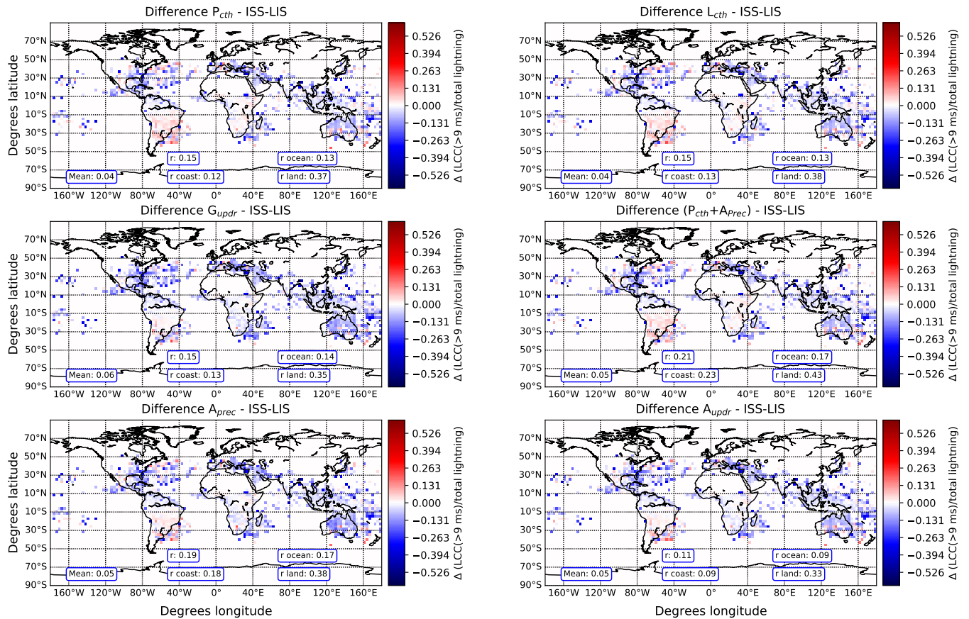
Figure 12. Difference between the observed and the simulated ratio of LCC(>9 ms)-lightning to total lightning density September, October and November using different lightning parameterizations. Positive values indicate that the model overestimates the ratio. The calculated global, land and ocean spatial correlation coefficients r are included.
