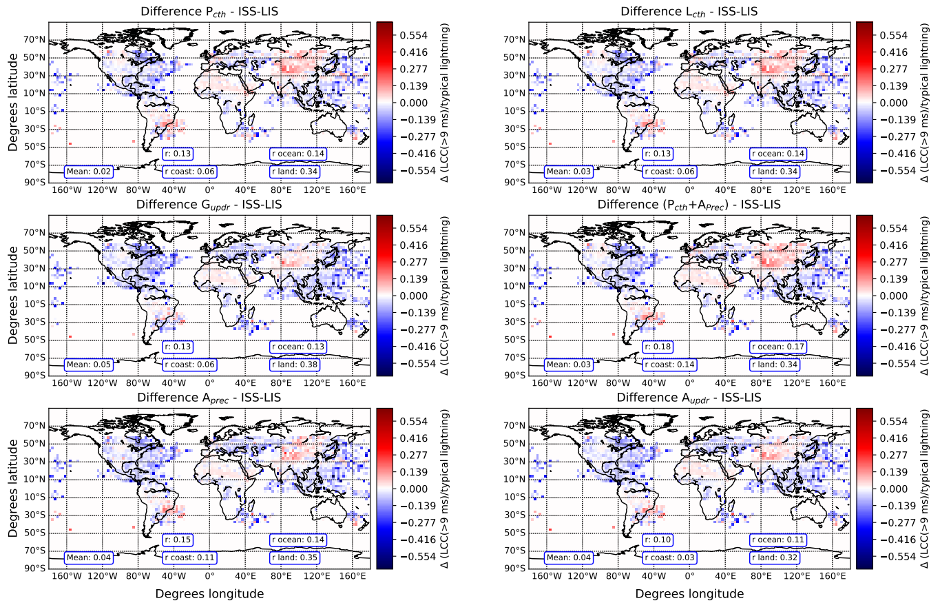
Figure 11. Difference between the observed and the simulated ratio of LCC(>9 ms)-lightning to typical total lightning density June, July and August using different lightning parameterizations. Positive values indicate that the model overestimates the ratio. The calculated global, land and ocean spatial correlation coefficients r are included.
