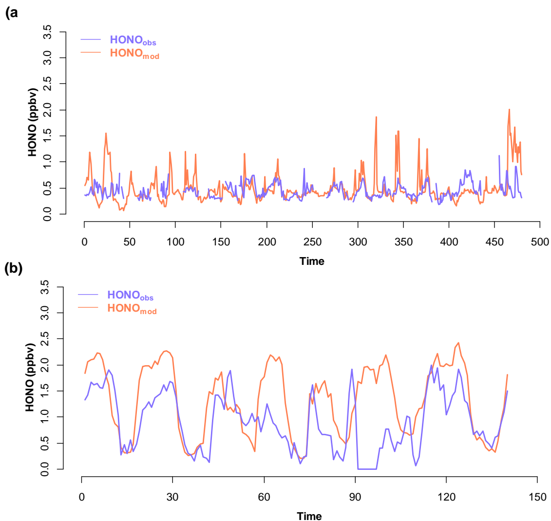
386 387 Figure 8. Comparison between the measured ( HONO_{obs} ) and calculated ( HONO_{mod} ) HONO 388 mixing ratios in Seoul during (a) June 2018 and (b) April 2019. The blue and red lines indicate 389 the measured and calculated HONO mixing ratio, respectively. The x axis indicates the hour 390 from the beginning of the experiment, which is (a) 00:00 on 1 st June 2018 and (b) 00:00 on 12 th 391 April 2019.
