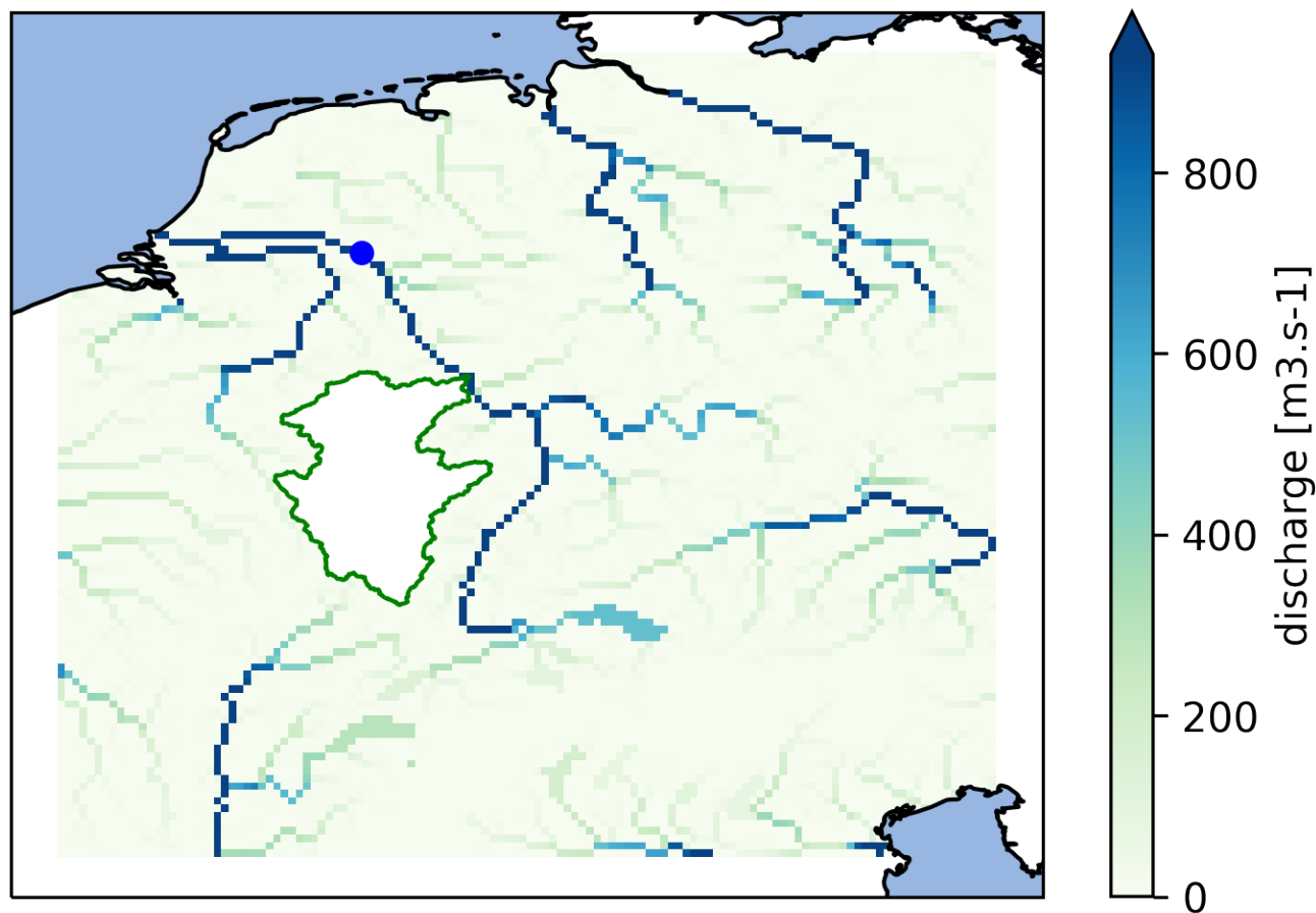
Figure 9. Calculated discharge in the Rhine basin at the end of the model run using the PCR-GlobWB 2.0 model for the Rhine coupled with the MARRMoT model for the Moselle subcatchment. The Moselle subcatchment has been cut-out of the PCR-GlobWB 2.0 model (by altering its 'landmask' setting). The MARRMoT model calculates the discharge for the Moselle and each timestep this is added to the 'channel storage' parameter of PCR-GlobWB 2.0 at the location where the Moselle flows into the Rhine (at Koblenz). The blue dot on the map indicates the location of the observation station at Lobith, which is used for the hydrographs shown in Figure 11.
