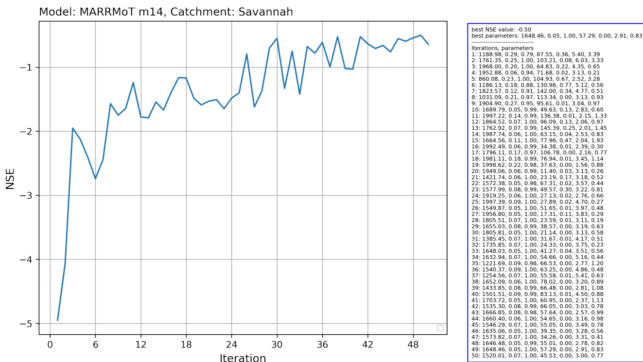
Figure 15. Output of the running the Covariance Matrix Adaptation Evolution Strategy (CMA-ES) calibration scheme from the CMA-ES/pycma software package on the MARRMoT m14 model (an implementation of TOPMODEL) for the Savannah basin.
