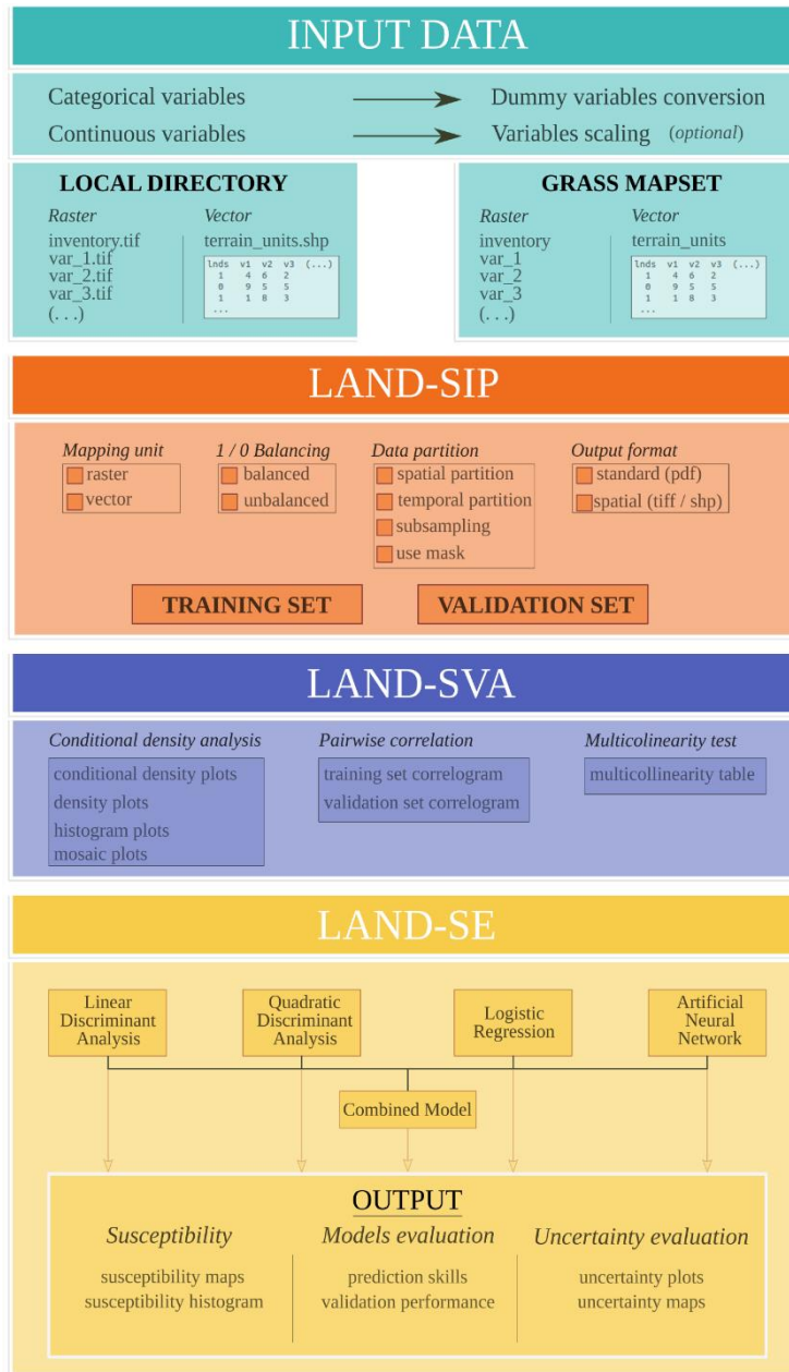
Figure 1: Logical schema of LAND-SUITE software.
