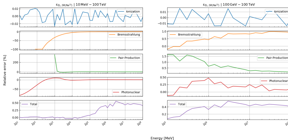
1005 Figure E5: Relative error of our energy loss calculations compared to the tabulated values from Groom et al. (2001) for standard rock ( ^{22}_{11}\text{Na} ) in the energy ranges: (left) 10 MeV – 100 TeV, (right) 100 GeV – 100 TeV.
