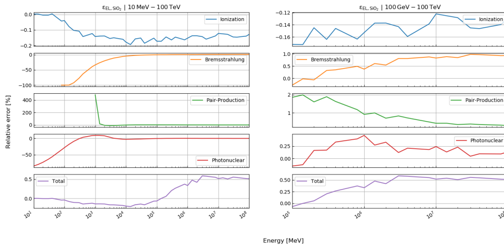
Figure E11: Relative error of our energy loss calculations compared to the tabulated values from Groom et al. (2001) for silicon dioxide (quartz) in the energy ranges: (left) 10 MeV – 100 TeV, (right) 100 GeV – 100 TeV.
