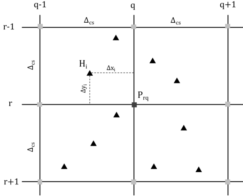
Figure 5: Two-dimensional stencil, used to summarise the bilinear interpolation of interface positions within cones ( H_i , \blacktriangle ) to a fixed grid ( P_{rq} , \blacksquare ) with a user-defined cell size \Delta_{cs} . Every interface position within a \pm\Delta_{cs} interval contributes to the grid height P_{rq} .
