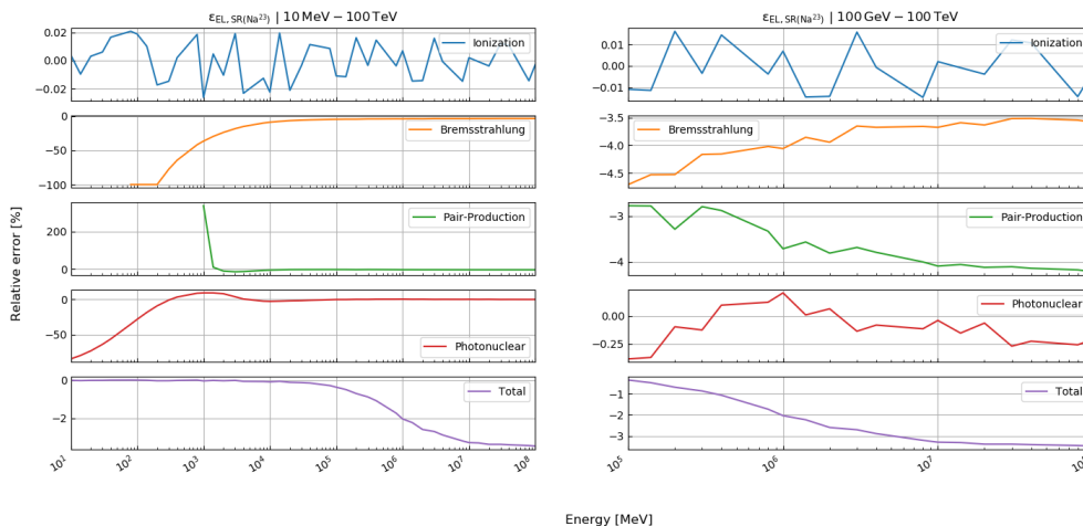
1000 Figure E4: Relative error of our energy loss calculations compared to the tabulated values from Groom et al. (2001) for standard rock ( ^{23}_{11}\text{Na} ) in the energy ranges: (left) 10 MeV – 100 TeV, (right) 100 GeV – 100 TeV.
