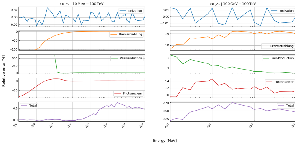
Figure E7: Relative error of our energy loss calculations compared to the tabulated values from Groom et al. (2001) for calcium in the energy ranges: (left) 10 MeV – 100 TeV, (right) 100 GeV – 100 TeV.
