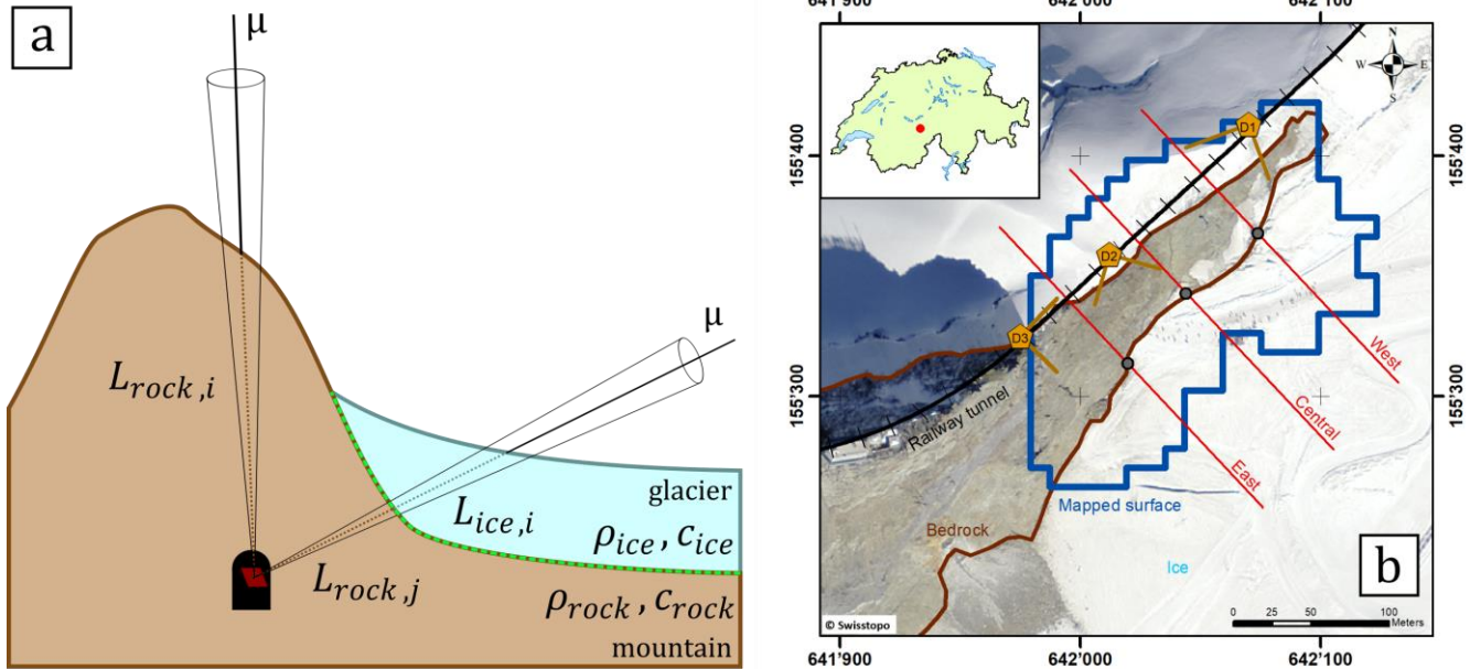
65 Figure 1: a) Schematic side view of the experiment from Nishiyama et al. (2017). A muon detector (red) is placed in a tunnel or 66 cavity and records muons from the cosmic ray flux that penetrate the material (ice & rock) from different directions. Muons that are detected along cones yield information on the amount and density of matter between the topographic surface and the detector. Based on this the interface between ice and rock (dashed green line) can be reconstructed. b) Modified Fig. 1 from Nishiyama et al. (2017); Overview of the study region in the central Swiss Alps. Detectors are indicated by yellow pentagrams (D1, D2, D3; 70 including their viewfield) within the railway tunnel (black line). The imaged area is outlined in blue and the region that we know from the digital elevation model to contain only rock is marked in brown. We verified (see Sect. 4) the reconstruction in this study with the one from Nishiyama et al. (2017) along three cross-sections (East, Central, West; red lines). Basemap: Orthophotomosaic Swissimage, © Federal Office of Topography swisstopo.
