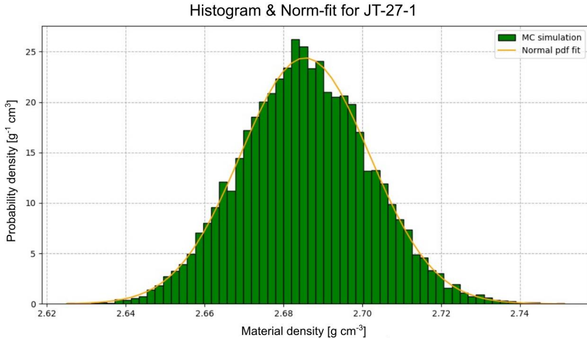
795 Figure B1: Example output of “subsample_analysis.py” for a bulk density measurement of subsample JT-27-1 (see supplementary information for data). Green bars represent the histogram of 10’000 Monte Carlo simulation draws. The orange curve indicates the fitted normal probability density function.
