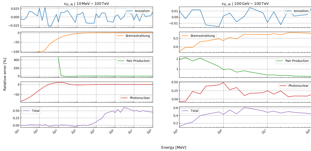
Figure E6: Relative error of our energy loss calculations compared to the tabulated values from Groom et al. (2001) for aluminium in the energy ranges: (left) 10 MeV – 100 TeV, (right) 100 GeV – 100 TeV.
