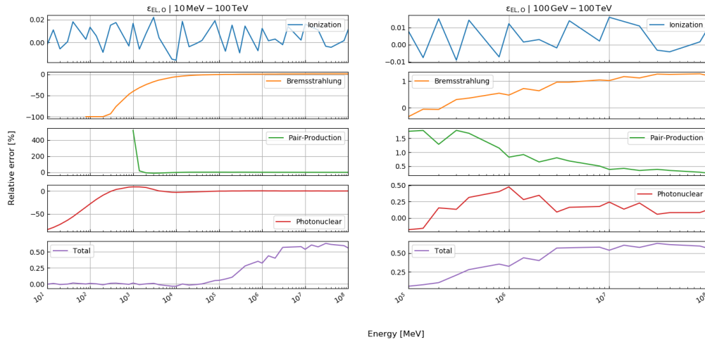
Figure E9: Relative error of our energy loss calculations compared to the tabulated values from Groom et al. (2001) for oxygen in the energy ranges: (left) 10 MeV – 100 TeV, (right) 100 GeV – 100 TeV.
