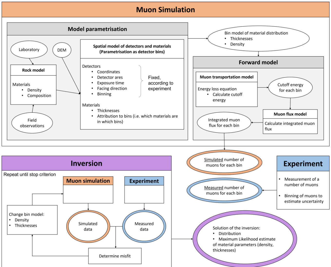
185 Figure 2: A schematic flowchart showing the different involved models in a muon tomographic experiment. The muon simulation 190 consists of a model for rocks, detectors, the cosmic ray flux and a particle physical model on how muons lose energy upon travelling through rocks. These models allow for a synthetic data set to be computed. The systematic comparison between synthetic data and actual measured data and the subsequent change of the model parameters to find the set of parameters that reproduce the measured data best is an (often iterative) optimisation problem. This procedure is termed “inversion” (usually) by geophysicists.
