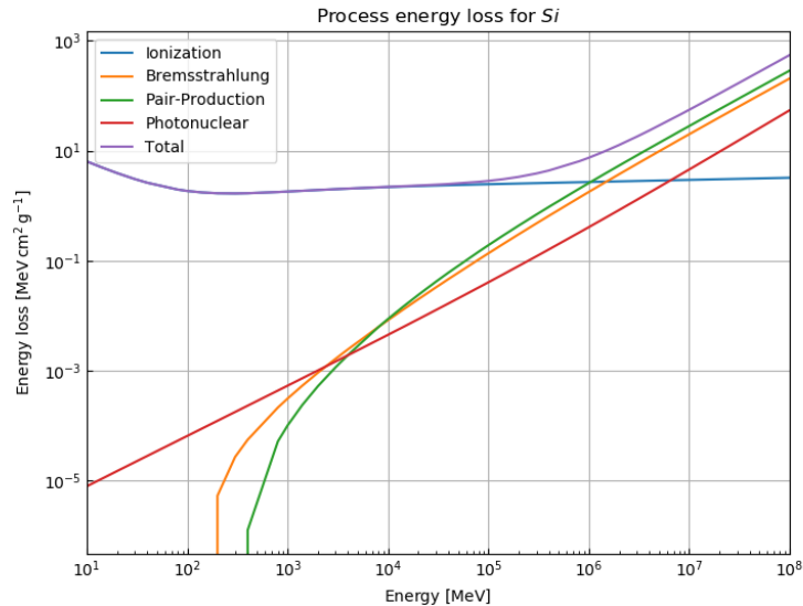
950 Figure E1: Log-log plot of the stopping power of the different energy loss processes for silicon. At \sim 10 \text{ GeV} the radiative processes (i.e. bremsstrahlung, pair-production and photonuclear interactions) reach around 1 % of the total stopping power. At a few hundred GeV (at the so called “critical energy”) the radiative processes start to become dominant over the ionisation losses.
