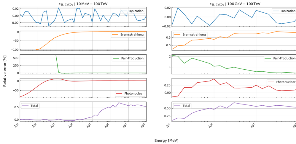
Figure E10: Relative error of our energy loss calculations compared to the tabulated values from Groom et al. (2001) for calcium carbonate (calcite) in the energy ranges: (left) 10 MeV – 100 TeV, (right) 100 GeV – 100 TeV.
