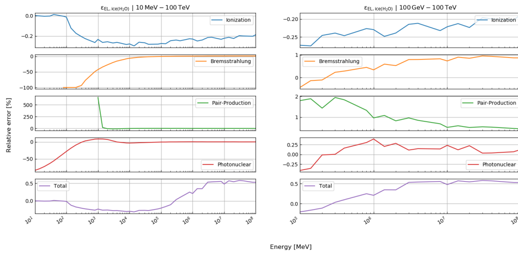
Figure E12: Relative error of our energy loss calculations compared to the tabulated values from Groom et al. (2001) for ice in the energy ranges: (left) 10 MeV – 100 TeV, (right) 100 GeV – 100 TeV.
