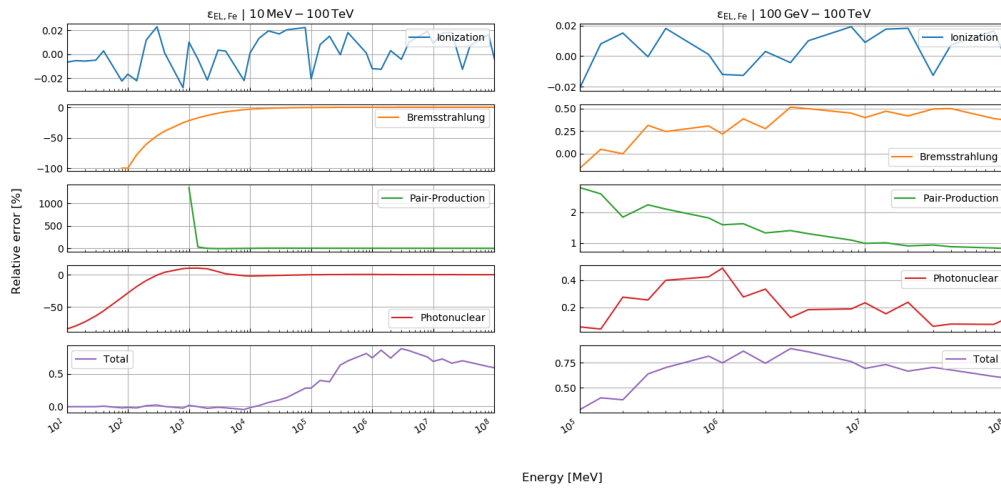
1015 Figure E8: Relative error of our energy loss calculations compared to the tabulated values from Groom et al. (2001) for iron in the energy ranges: (left) 10 MeV – 100 TeV, (right) 100 GeV – 100 TeV.
