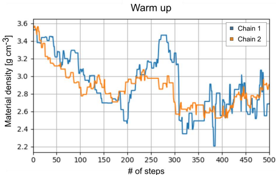
Figure 4: Example of a trace plot (2 independent chains; blue and orange) of a MH run with 500 draws. This plot shows the parameter value (here material density) vs. # of steps of a collection of cones in which we (Nishiyama et al., 2017) knew that only rock is present. This is a calculation that is included in the code base. The warm-up phase of this MH algorithm takes roughly 150 simulations indicated by the subsequent oscillation around a parameter value of \sim 2.7 - 2.8 \text{ g cm}^{-3} .
