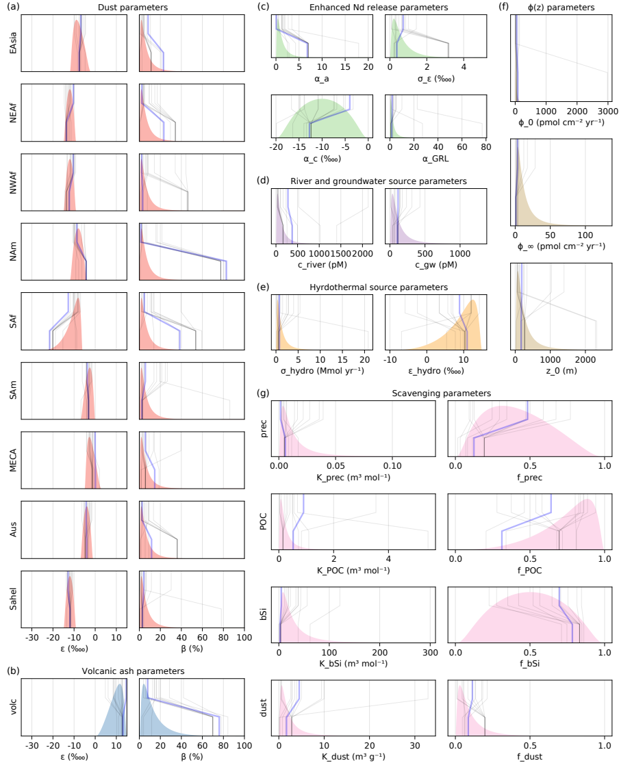
Figure B1. Parameter prior distributions (color-filled densities), and initial and optimized parameter values for a dozen of optimization runs (vertical black-lines). Each line starts by showing the initial parameter value at the top and is connected to the final optimized value at the bottom. The thicker blue line represents the optimization run that was used as our “best” estimate. (a) Dust \epsilon_{Nd} values ( \epsilon_r ) and solubility solubilities ( \beta_r ) for each region of origin r . (b) Volcanic ash \epsilon_{Nd} value ( \epsilon_{volc} ) and solubility ( \beta_{volc} ). (c) Enhanced Nd release parameters, \alpha curve parameters (curvature \alpha_a and center \alpha_c ), Greenland enhancement ( \alpha_{GRL} ), and global standard deviation of per-grid-cell in situ sedimentary \epsilon_{Nd} ( \sigma_\epsilon ). (d) Rivers and groundwater Nd concentrations ( c_{river} and c_{gw} ). (e) Global Hydrothermal-hydrothermal source magnitude ( \sigma_{hydro} ) and \epsilon_{Nd} ( \epsilon_{hydro} ). (f) Sedimentary flux parameters ( \phi_0 , \phi_\infty , and z_0 ) (g) Reversible scavenging reaction equilibrium constants, K_X , and fractions returned to water when reaching seafloor, f_X , for each particle type X . See also Table 2.
