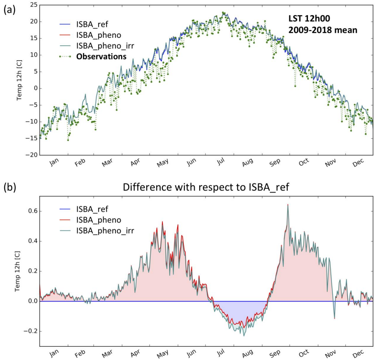
985 Figure 8 – Seasonal variation of surface temperature daily values at 12:00 local time (degree C) in the most densely irrigated part of Nebraska (Fig. 2e) from 2009 to 2018 (a) as derived from the reference simulation ISBA_ref (blue line), ISBA_pheno (red line), ISBA_pheno_irr (cyan) and the CGLS product (green dotted line). The surface temperature differences at 12:00 local time (b) of ISBA_pheno_irr and ISBA_pheno simulations with respect to the ISBA-ref simulations are shown.
