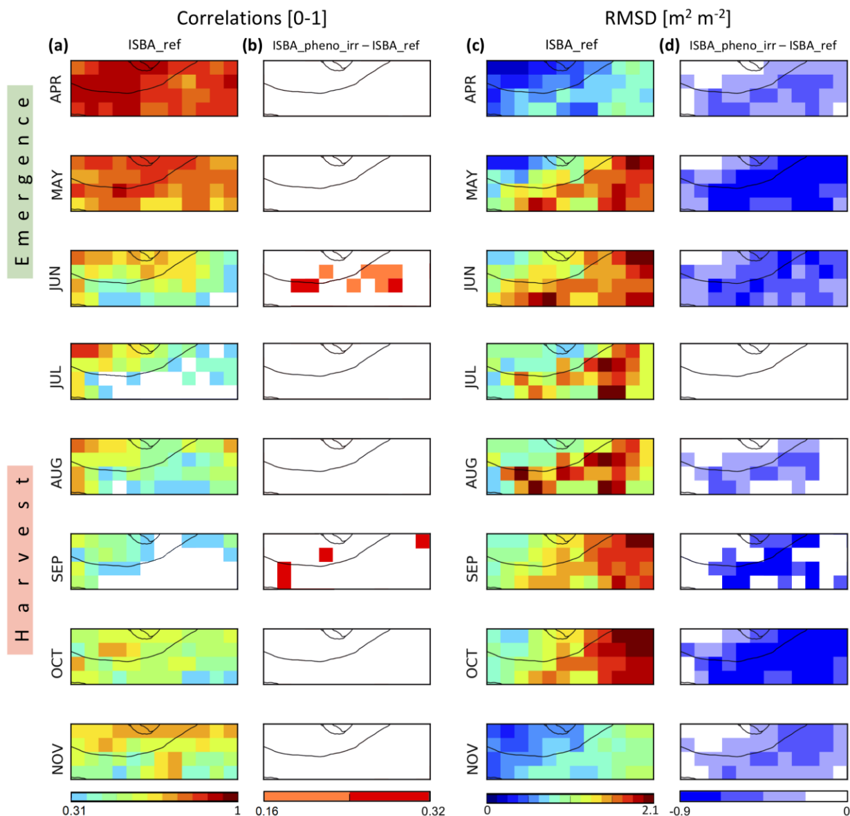
975 Figure 7 – Comparison of simulated LAI with CGLS LAI observations in the most densely irrigated part of Nebraska (Fig. 2e) from 1999 to 2018 during the vegetation growing and senescence time period from April to November. Monthly temporal correlation (a, b) and RMSD (c, d) maps are shown for the reference simulation without a representation of irrigation ISBA_ref (a, c). The added value of the ISBA_pheno_irr simulation with respect to ISBA-ref is 980 shown through score difference maps (b, d). White is used to mask non-significant correlation and score difference values.
