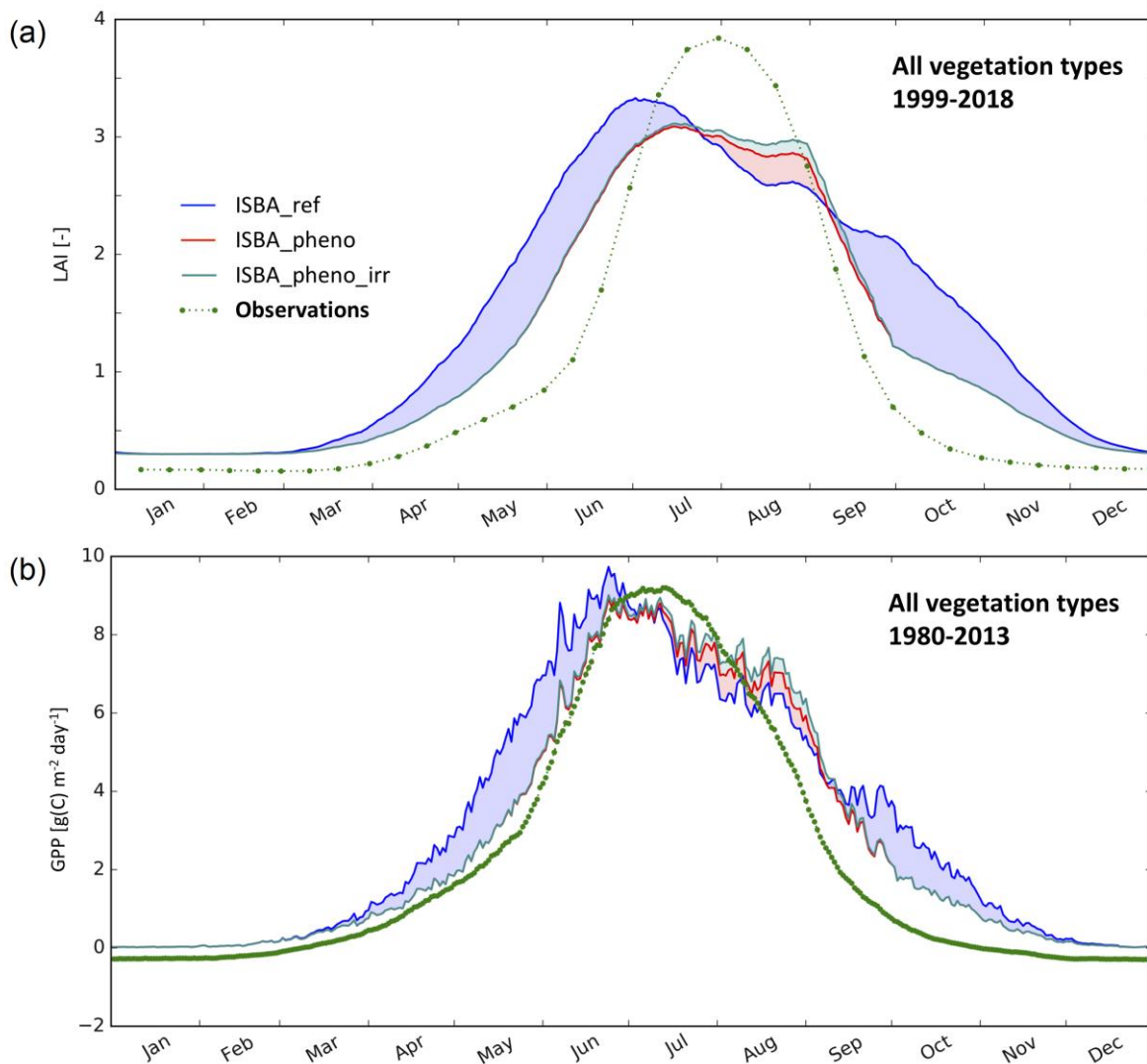
960 Figure 5 – Simulated vs. observed LAI and GPP of all vegetation types, in the most densely irrigated part of Nebraska (Fig. 2e): (a) seasonal variation of mean LAI (m²m⁻²) from 1999 to 2018, (b) seasonal variation of mean GPP (gC m⁻² d⁻¹) 1980 to 2013. ISBA_ref, ISBA_pheno, ISBA_pheno_irr simulations are represented by blue, red, and cyan lines, and satellite-derived observations by green dots.
