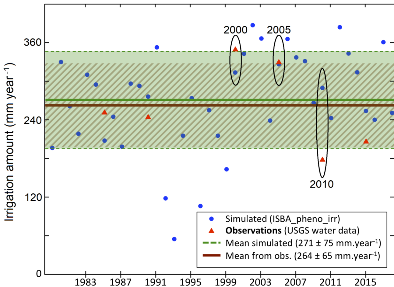
945 Figure 3 – Yearly cumulated irrigation amounts simulated by the model for the studied area in Nebraska from 1979 to 2018 (blue dots). The six USGS observations from 1985 to 2018 are shown (red triangles). The mean and standard deviation of the yearly values are shown for the model (green solid and dashed lines, respectively), and for the USGS data (brown lines). The 2000 and 2005 dry years are indicated, together with the 2010 wet year.
