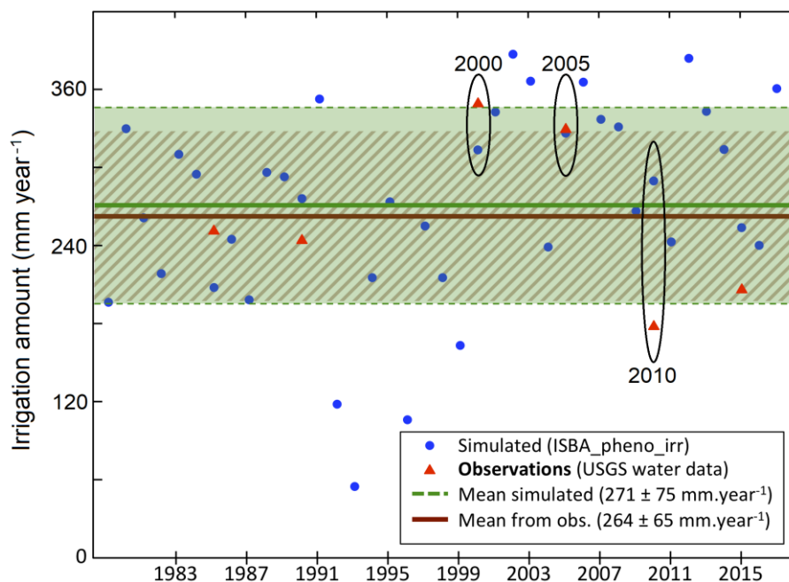
Figure 3 – Yearly cumulated irrigation amounts simulated by the model for the studied area in Nebraska from 1979 to 2018 (blue dots). The six USGS observations from 1985 to 2015 58 are shown (red triangles). The mean and standard deviation of the yearly values are shown for the model (green solid and dashed lines, respectively), and for the USGS data (brown lines). The 2000 and 2005 dry years are indicated, together with the 2010 wet year.
