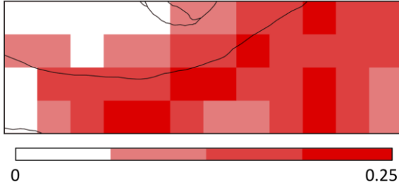
(a) LAI Correlation: ISBA_pheno_irr – ISBA_ref
