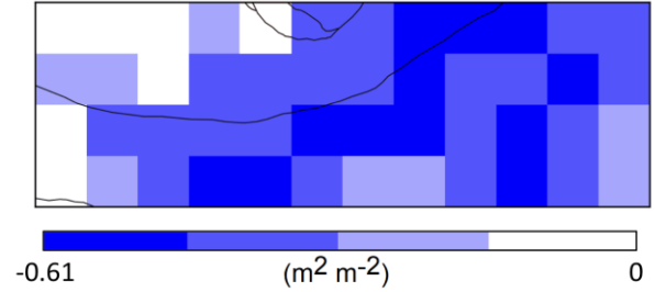
(b) LAI RMSD: ISBA_pheno_irr – ISBA_ref
