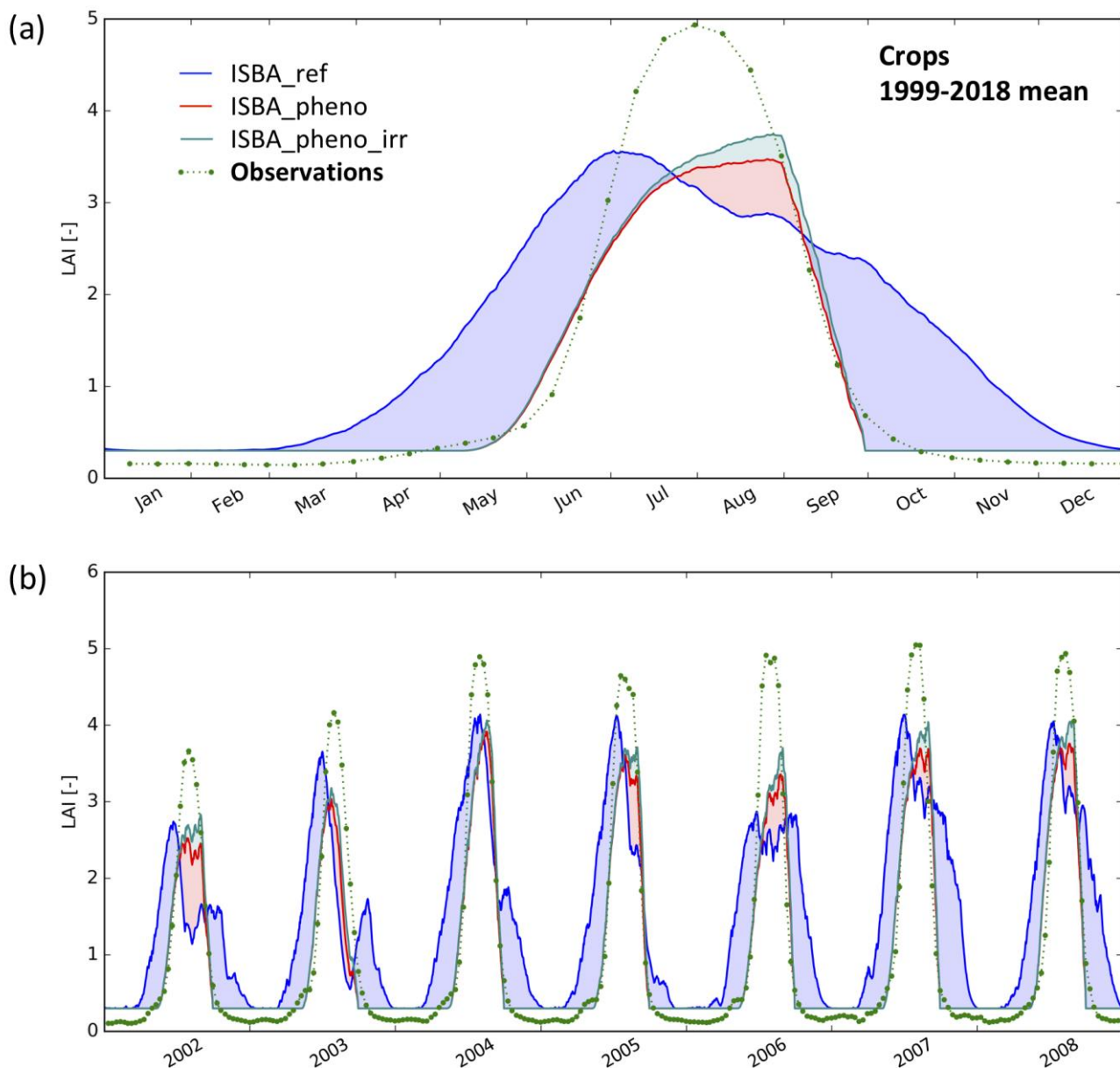
975 Figure 4 – LAI ( \text{m}^2 \text{m}^{-2} ) of irrigated crops (C3 or C4) in the most densely irrigated part of Nebraska (Fig. 2e): (a) seasonal variation for the time period from 1999 to 2018, (b) daily time series from 2002 to 2008. Simulated LAI is shown for the irrigated fraction, from the reference simulation (ISBA_ref, blue line), and from the simulations with only agricultural practices and with agricultural practices and irrigation (ISBA_pheno, red line, and ISBA_pheno_irr, cyan line, respectively). Satellite-derived LAI observations (green dots) are for areas where the fraction of C3 or C4 irrigated crops is larger than 50 %.
