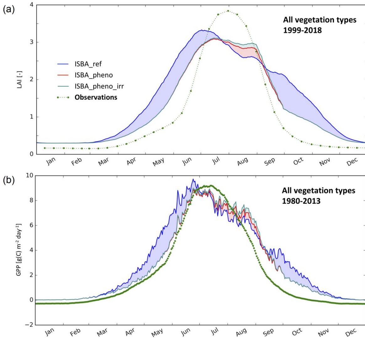
Figure 56 – Simulated vs. observed LAI and GPP ( \text{m}^2\text{m}^{-2} ) of all vegetation types, in the most densely irrigated part of Nebraska (Fig. 12e): from 1999 to 2018: (a) seasonal variation of mean LAI ( \text{m}^2\text{m}^{-2} ) from 1999 to 2018, (b) seasonal variation of mean GPP ( \text{gC m}^{-2}\text{d}^{-1} ) 1980 to 2013. of ISBA_ref (blue line), ISBA_pheno (red line), ISBA_pheno_irr (cyan) simulations and of satellite-derived observations are represented by blue, red, and cyan lines, and satellite-derived observations by (green dots), (b) temporal correlation and (c) RMSD score difference maps showing the added value of the ISBA_pheno_irr with respect to ISBA_ref. Positive value for correlation (Fig. 6b) means that the result of ISBA_pheno_irr is better, and for RMSD (Fig. 6c) negative value means that result of ISBA_pheno_irr is better.
