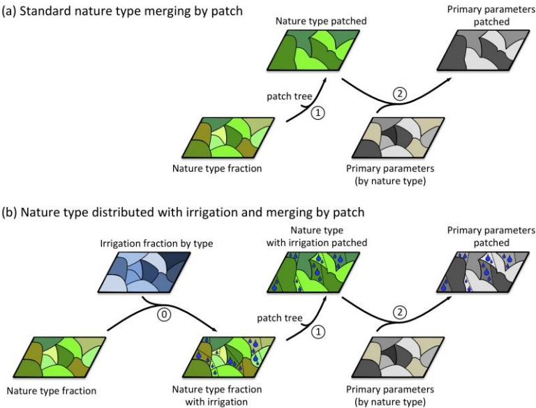
Figure 3 — Diagram of the processing steps to obtain the ISBA model primary parameters from the nature types: (a) with the original method and (b) with the new method developed for irrigation. The different steps consist of: (0) cross-referencing the maps of vegetation cover (nature types) and irrigation fractional coverage (addition of irrigated nature type classes where irrigation is possible), (1) merging nature type classes following path aggregation rules (see Fig. S1.1), and (2) computing primary parameter values following the patch faction map.
