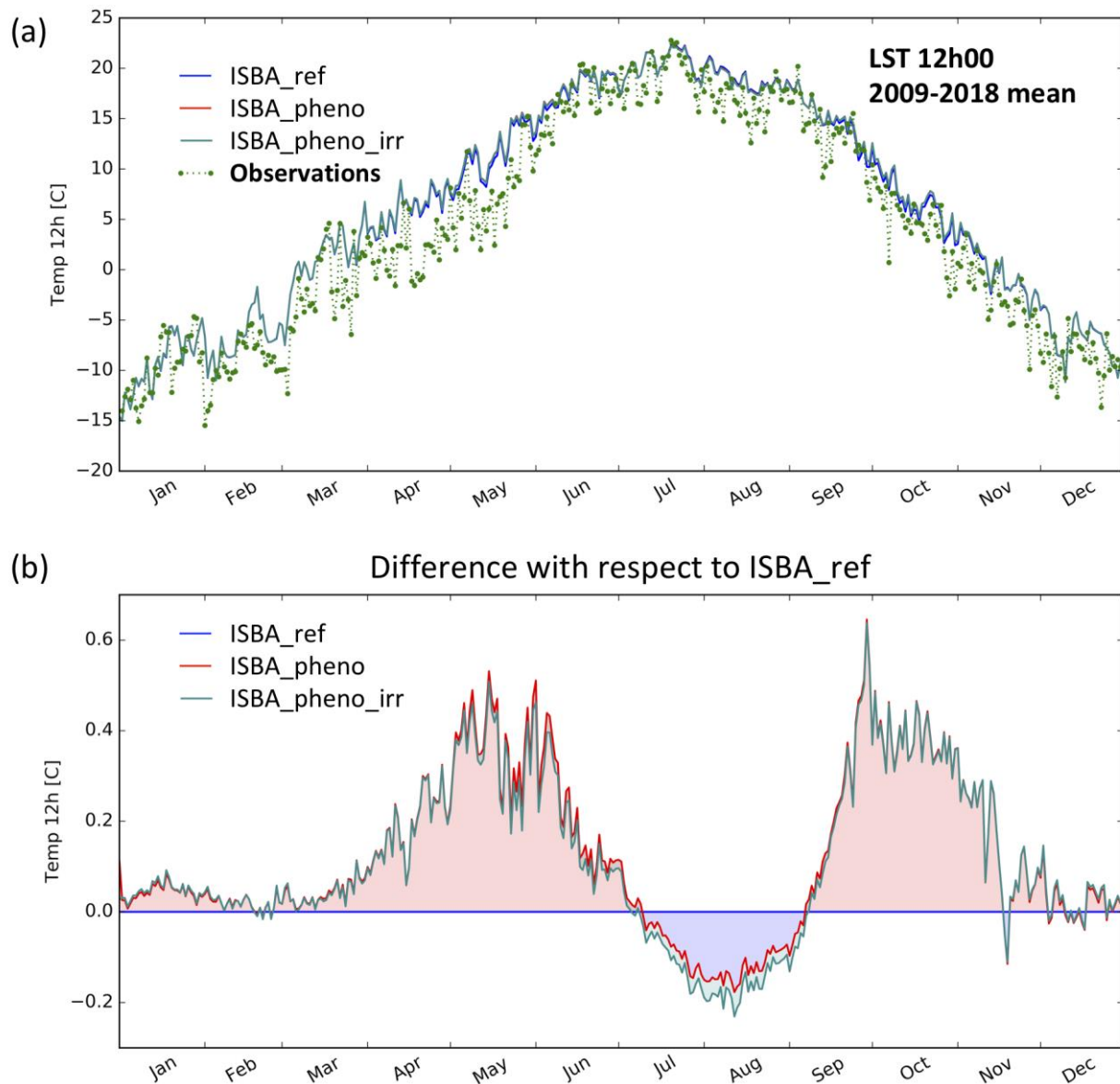
Figure 811 – Seasonal variation of surface temperature daily values at 12:00 local time (degree C) in the most densely irrigated part of Nebraska (Fig. 21e) from 2009 to 2018 (a) as derived from the reference simulation ISBA_ref (blue line), ISBA_pheno (red line), ISBA_pheno_irr (cyan) and the CGLS product (green dotted line). The surface temperature differences at 12:00 local time (b) of ISBA_pheno_irr and ISBA_pheno simulations with respect to the ISBA-ref simulations are shown.
