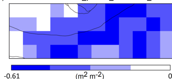
(b) LAI RMSD: ISBA_pheno_irr – ISBA_ref
