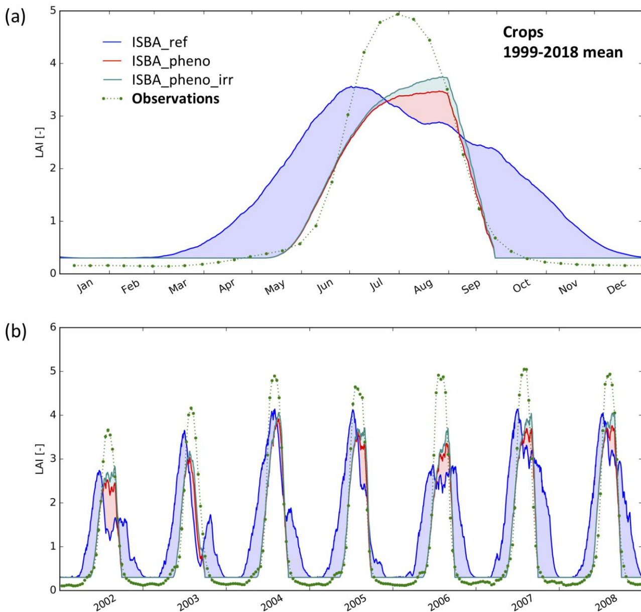
Figure 45 – LAI ( \text{m}^2 \text{m}^{-2} ) of irrigated crops (C3 or C4) in the most densely irrigated part of Nebraska (Fig. 21e): (a) seasonal variation for the time period from 1999 to 2018, (b) daily time series from 2002 to 2008. Simulated LAI is shown for the irrigated fraction, from the reference simulation (ISBA_ref, blue line), and from the simulations with only agricultural practices and with agricultural practices and irrigation (ISBA_pheno, red line, and ISBA_pheno_irr, cyan line, respectively). Satellite-derived LAI observations (green dots) are for areas where the fraction of C3 or C4 irrigated crops is larger than 50 %.
