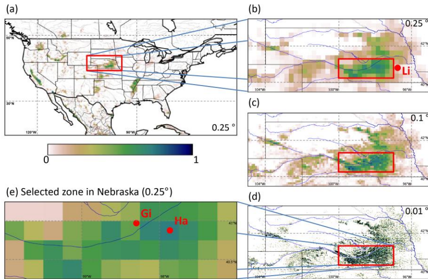
Figure 1--Irrigation fractional coverage derived from Meier et al. (2018) over (a) the Continental United State (CONUS), (b, c, d, e) Nebraska: at (b) 0.25^{\circ}\times0.25^{\circ} , (c) 0.1^{\circ}\times0.1^{\circ} , (d) 0.01^{\circ}\times0.01^{\circ} spatial resolutions, and (e) over the selected zone in southern Nebraska considered in this study ( 100-97^{\circ}\text{W} , 40.25-41.25^{\circ}\text{N} ). The red boxes show the location of the different zooms. The “Li”, “Gi” and “Ha” red dots correspond to the Lincoln weather station, Grand Island weather station, and Hampton irrigated area, respectively.
