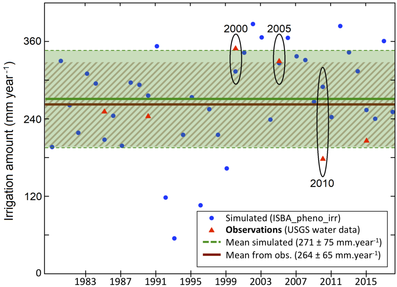
Figure 43 – Yearly cumulated irrigation amounts simulated by the model for the studied area in Nebraska from 1979 to 2018 (blue line dots). The six USGS observations from 1985 to 2018 are shown (red triangles). The mean and standard deviation of the yearly values are shown for the model (green solid and dashed lines, respectively), and for the USGS water data from 1985 to 2019 (brown lines). The 2000 and 2005 dry years are indicated, together with the 2010 wet year.
