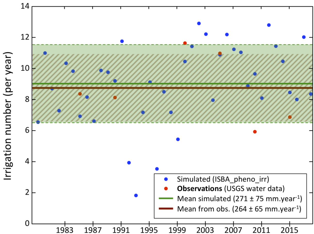
Figure 3-4 – Yearly cumulated number of irrigation events simulated by the model for the studied area in Nebraska from 1979 to 2018 (blue line). The mean and standard deviation of the yearly values are shown for the model (green solid and dashed lines, respectively), and for the USGS water data from 1985 to 2019 (brown lines).
