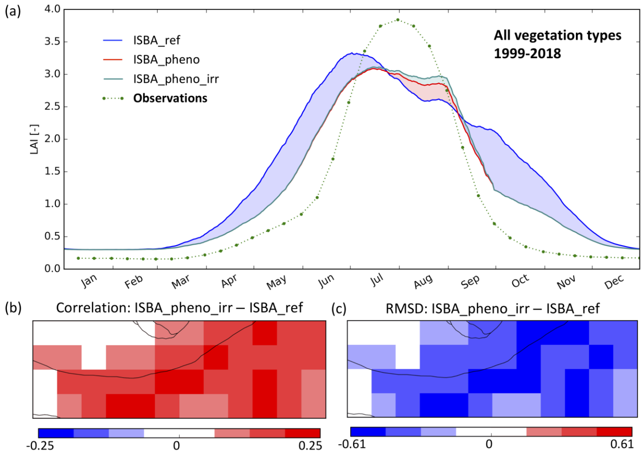
Figure 5-6 – Simulated vs. observed LAI ( \text{m}^2\text{m}^{-2} ) of all vegetation types, in the most densely irrigated part of Nebraska (Fig. 1e) from 1999 to 2018: (a) seasonal variation of mean LAI of ISBA_ref (blue line), ISBA_pheno (red line), ISBA_pheno_irr (cyan) simulations and of satellite-derived observations (green dots), (b) temporal correlation and (c) RMSD score difference maps showing the added value of the ISBA_pheno_irr with respect to ISBA-ref.
