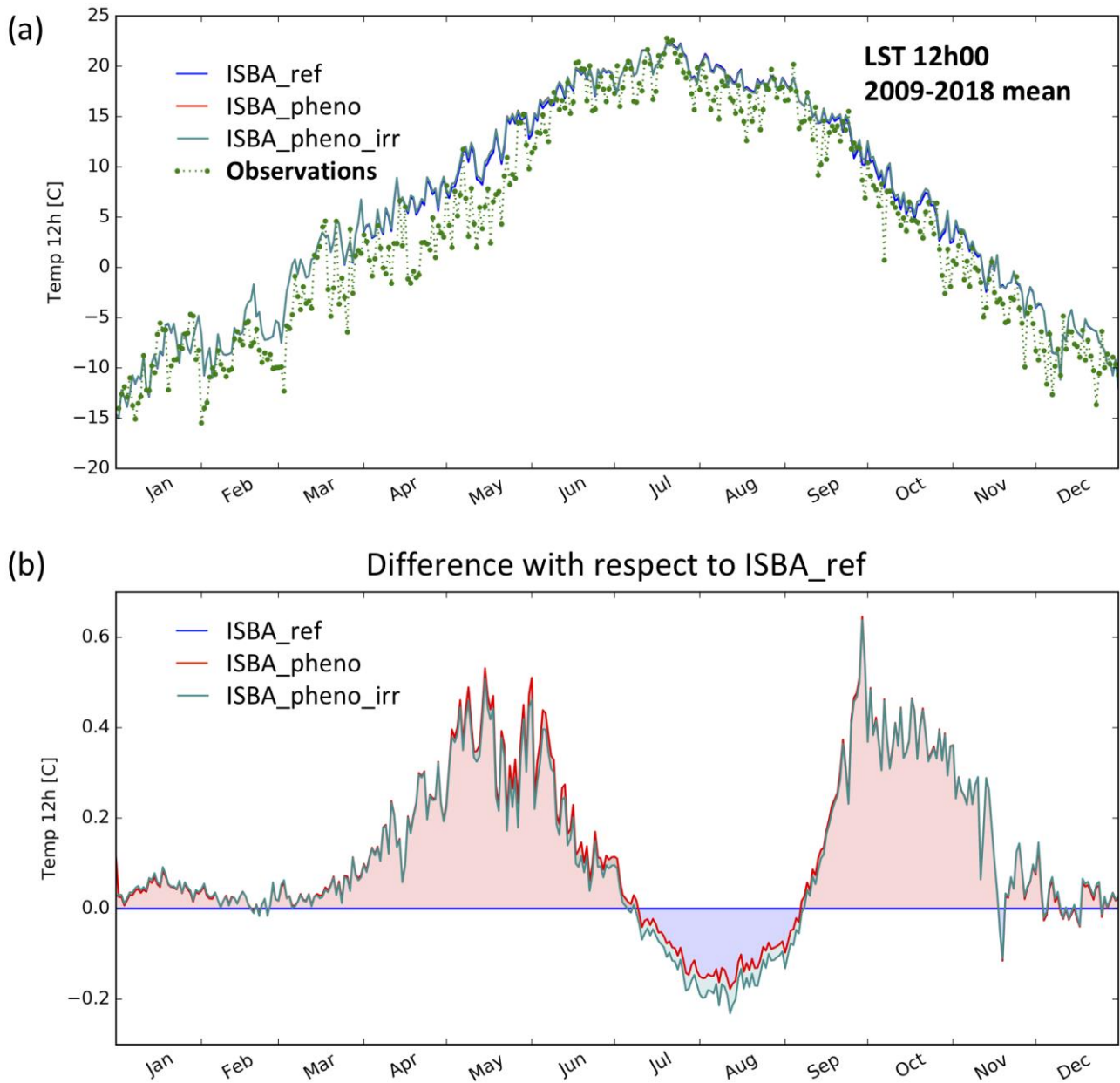
Figure 10-11 – Seasonal variation of surface temperature daily values at 12:00 local time (degree C) from 2009 to 2018 (a) as derived from the reference simulation ISBA_ref (blue line), ISBA_pheno (red line), ISBA_pheno_irr (cyan) and the CGLS product (green dotted line). The surface temperature differences at 12:00 local time (b) of ISBA_pheno_irr and ISBA_pheno simulations with respect to the ISBA-ref simulations are shown.
