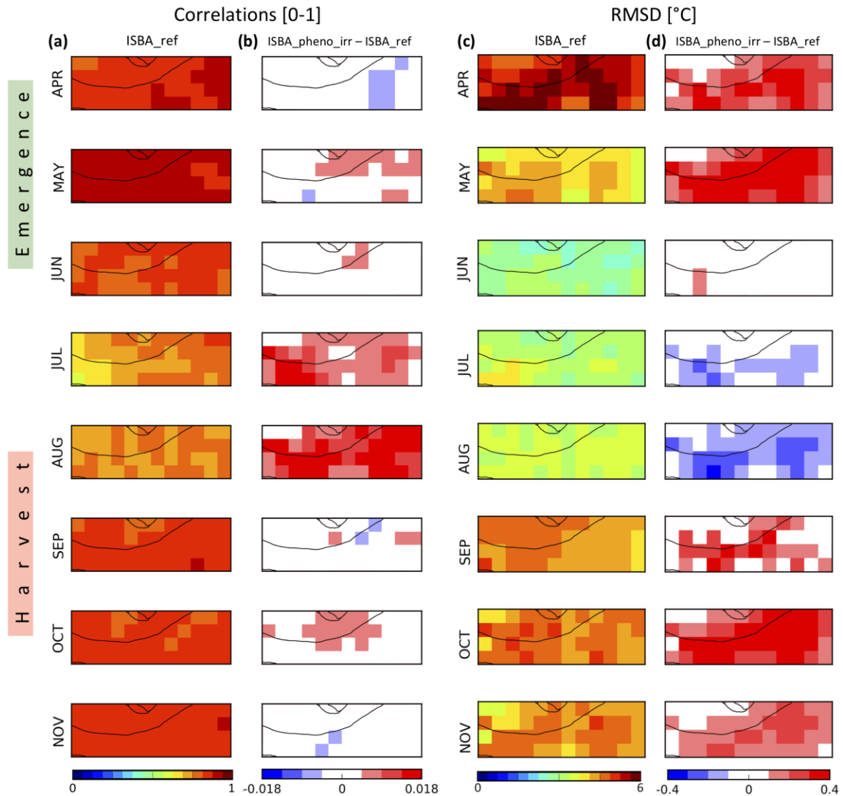
Figure 11-12 – Comparison of simulated surface temperature daily values at 12:00 local time with CGLS observations from 2009 to 2018 during the vegetation growing and senescence time period from April to November. Monthly temporal correlation (a, b) and RMSD (c, d) maps are shown for the reference simulation without a representation of irrigation ISBA_ref (a, c). The added value of the ISBA_pheno_irr simulation with respect to ISBA-ref is shown through score difference maps (b, d).
