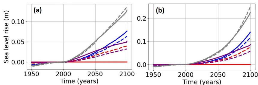
295 Figure 2: Projected changes up to 2100 (relative to 1986-2005) of dominating barystatic SLR contributions scaled to the IBI domain using their spatial fingerprints for (a) SSP1-2.6 scenario (b) SSP5-8.5 scenario. The SL contributions evaluated here are: the Antarctic ice-sheet contribution (blue), the Greenland ice-sheet contribution (red), the glaciers contribution (purple), and their sum (grey). The dashed lines represent the initial CNRM-CM6-1-HR contributions and the solid lines the contributions based on Oppenheimer et al., 2019 for the Antarctic ice sheet and on Hock et al., 2019 for glaciers.
