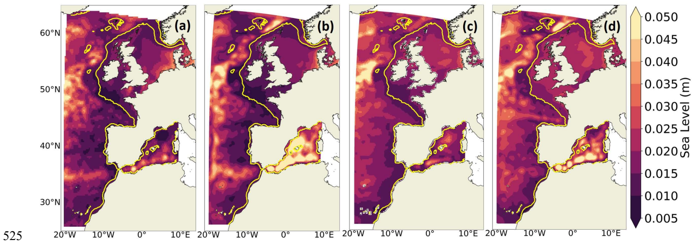
525 Figure 7: SL interannual variability over the 1993-2014 period in (a) altimetry (b) IBI-ERAi (c) CNRM-CM6-1-HR and (d) IBI-CCS_corr. The interannual variability is computed as the standard deviation of the detrended annual mean SL. Note that all panels here do not include the inverse barometer effect on sea level. The shelf break (defined by the 200 m isobath is indicated in yellow).
