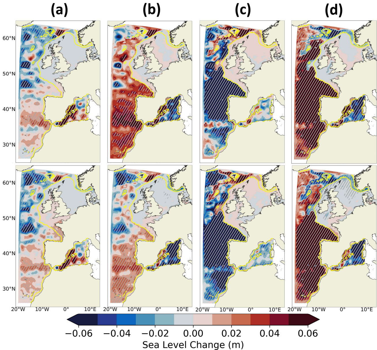
715 Figure 15: Differences of projected changes (2081-2100 vs 1986-2005) between IBI-CCS_corr and IBI-CCS_raw simulations for the DSL (first column), the steric (second column), thermosteric (third column) and halosteric (last column) SL components under the SSP5-8.5 (upper row) and SSP1-2.6 (lower row) scenarios. The steric, thermosteric and halosteric SL components have been computed between 0-2000 m depth. A student test has been performed with a confidence interval of 95% and the significant differences between the two simulations have been marked with white dots. The shelf break (defined by the 200 m isobath is indicated in yellow).
