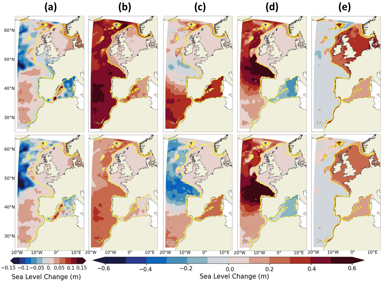
640 Figure 12: Projected changes (2081-2100 vs 1986-2005) under the SSP5-8.5 (upper row) and SSP1-2.6 (lower row) scenarios in the IBI-CCS_corr simulation for the (a) DSL, (b) steric, (c) thermosteric (d) halosteric and (e) manometric SL components. The steric, thermosteric and halosteric SL components have been computed between 0-2000m depth. Note that the DSL mean over the IBI zone is 0. Note that the projected changes of the inverse barometer effect are not incorporated in the projected changes of manometric sea level (e). Moreover, as the changes are computed 0-2000m, the steric + manometric sea level changes are not equal to the DSL changes here. The shelf break (defined by the 200 m isobath is indicated in yellow).
