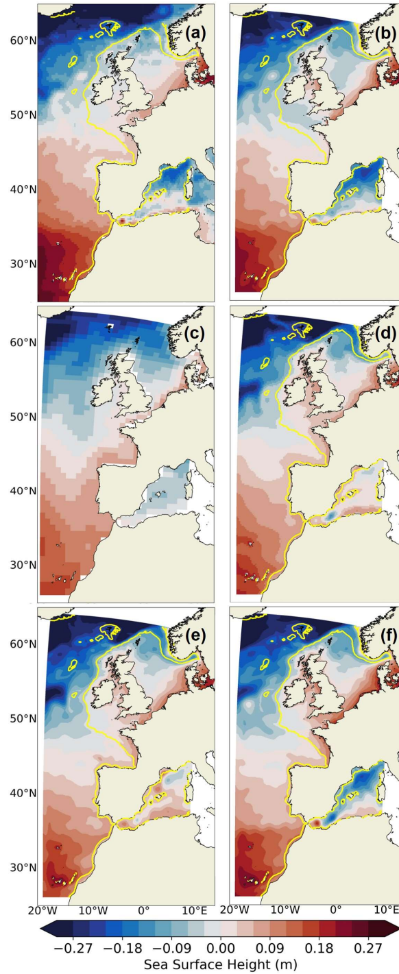
495 Figure 6: Mean sea surface height over the 1993-2014 period in (a) MDT CNES-CLS-18 (b) IBI-ERAi (c) CNRM-CM6-1 (d) CNRM-CM6-1-HR (e) IBI-CCS_raw and (f) IBI-CCS_corr. Note that all panels here do not include the inverse barometer effect on sea level. The shelf break (defined by the 200 m isobath is indicated in yellow).
