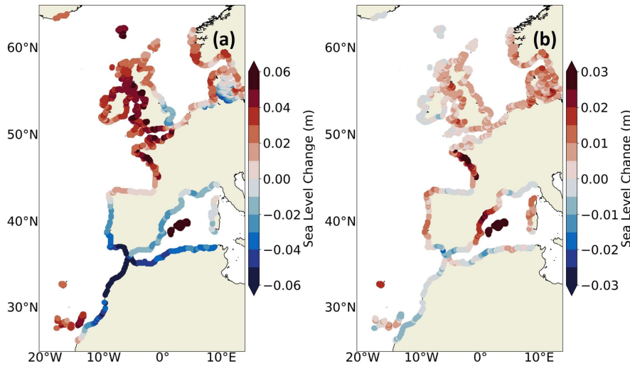
765 Figure 17: (a) Projected changes of the non-tidal residual 99 th percentile for the SSP5-8.5 scenario between 2081-2100 and 1986-2005 period in IBI-CCS_corr. (b) Differences with projected changes in IBI-CCS_raw.
