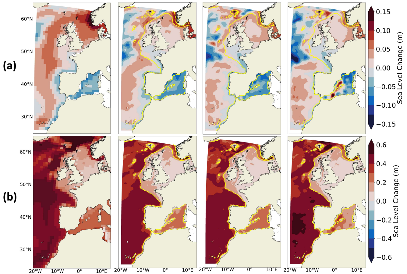
665 Figure 13: Projected changes (2081-2100 vs 1986-2005) in (a) DSL and (b) steric SL over 0-2000 m depth under the SSP5-8.5 scenario in CNRM-CM6-1 (first column), CNRM-CM6-1-HR (second column), IBI-CCS_raw (third column) and IBI-CCS_corr (last column) simulations. Note that the DSL mean over the IBI zone is 0 in the RCMs and thus, to compare the DSL between the GCMs and RCMs, the mean DSL over the IBI domain is removed from the GCMs. The shelf break (defined by the 200 m isobath is indicated in yellow).
