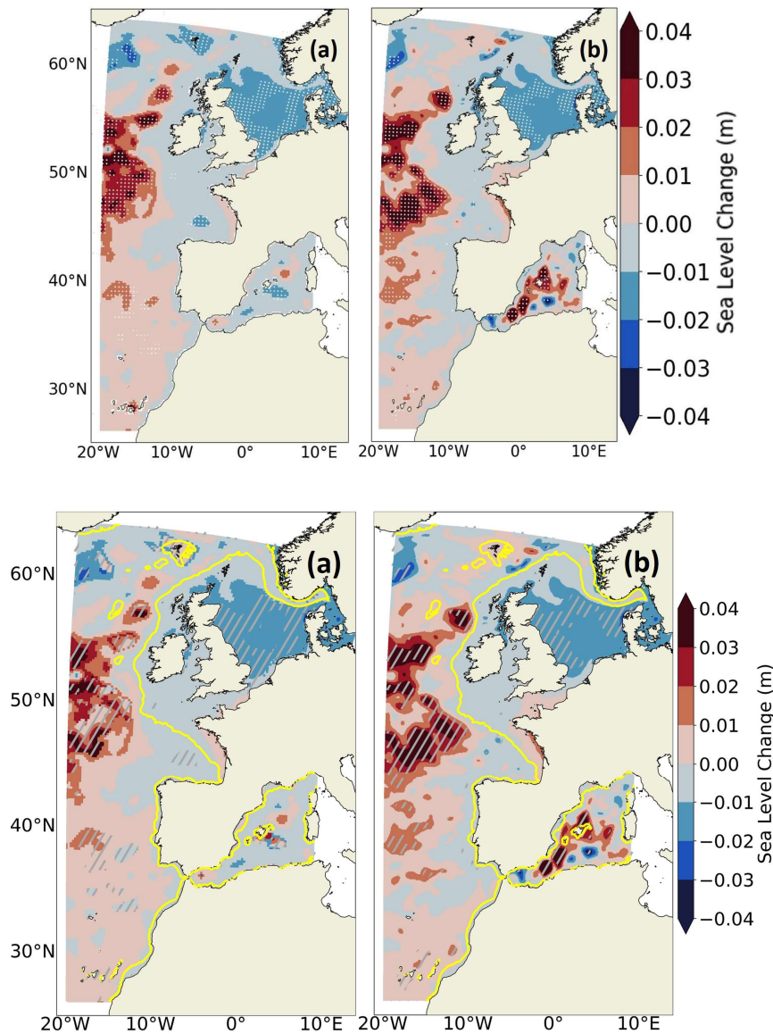
800 Figure 16: Projected changes (2081-2100 vs 1986-2005) of SL interannual variability under the SSP5-8.5 scenario for the (a) GCM CNRM-CM6-1-HR and (b) IBI-CCS_corr. The interannual variability is computed as the standard deviation of the detrended annual mean SL. A Fisher test has been performed with a confidence interval of 90% and the significant differences between the two simulations have been marked with white dots. The shelf break (defined by the 200 m isobath) is indicated in yellow.
