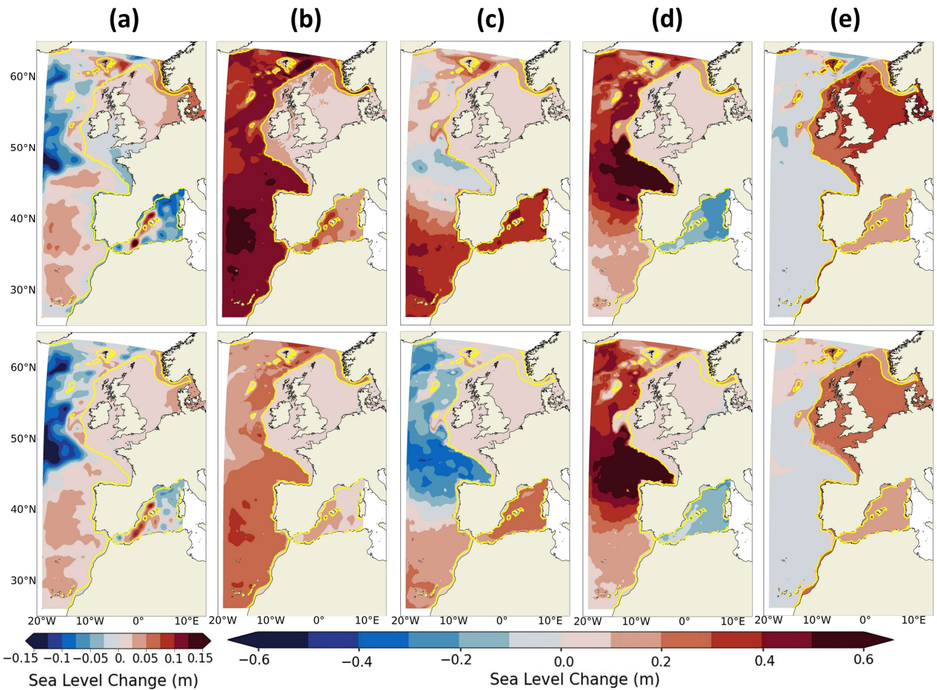
690 Figure 12: Projected changes (2081-2100 vs 1986-2005) under the SSP5-8.5 (upper row) and SSP1-2.6 (lower row) scenarios in the IBI-CCS_corr simulation for the (a) DSL, (b) steric, (c) thermosteric (d) halosteric and (e) manometric SL components. The steric, thermosteric and halosteric SL components have been computed between 0-2000m depth. Note that the DSL mean over the IBI zone is 0. Note that the projected changes of the inverse barometer effect are not incorporated in the projected changes of manometric sea level (e). Moreover, as the changes are computed 0-2000m, the steric + manometric sea level changes are not equal to the DSL changes here. The shelf break (defined by the 200 m isobath is indicated in yellow). 695
