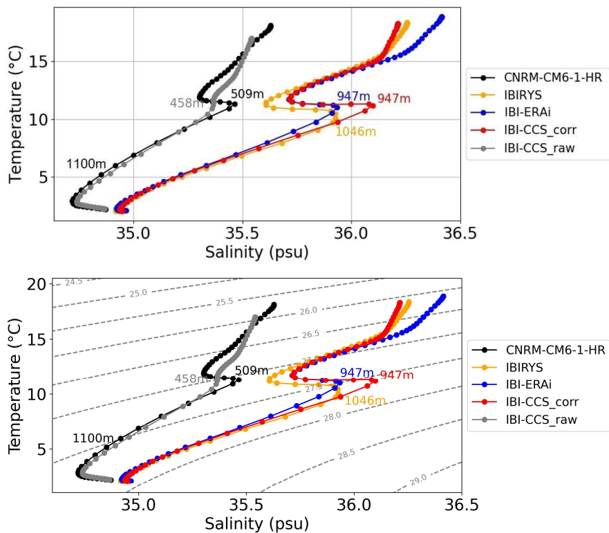
Figure 5: TS diagram performed at the star location of Fig. 1 over the 1993-2014 period for the CNRM-CM6-1-HR, IBIRYS, IBI-ERAi, IBI-CCS_corr, IBI-CCS_raw simulations.
