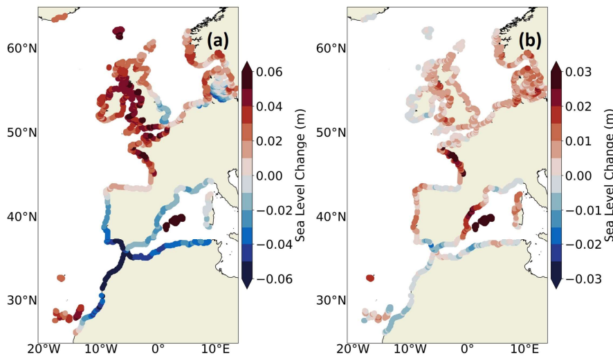
825 Figure 17: (a) Projected changes of the non-tidal residual 99 th percentile for the SSP5-8.5 scenario between 2081-2100 and 1986-2005 period in IBI-CCS_corr. (b) Differences with projected changes in IBI-CCS_raw.
