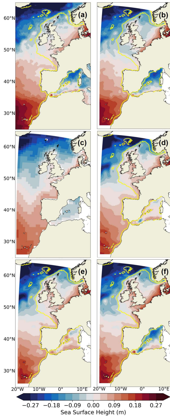
535 Figure 6: Mean sea surface height over the 1993-2014 period in (a) MDT CNES-CLS-18 (b) IBI-ERAi (c) CNRM-CM6-1 (d) CNRM-CM6-1-HR (e) IBI-CCS_raw and (f) IBI-CCS_corr. Note that all panels here do not include the inverse barometer effect on sea level. The shelf break (defined by the 200 m isobath is indicated in yellow).
