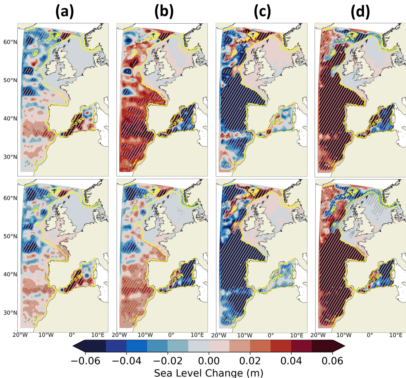
Figure 15: Differences of projected changes (2081-2100 vs 1986-2005) between IBI-CCS_corr and IBI-CCS_raw simulations for the DSL (first column), the steric (second column), thermosteric (third column) and halosteric (last column) SL components under the SSP5-8.5 (upper row) and SSP1-2.6 (lower row) scenarios. The steric, thermosteric and halosteric SL components have been computed between 0-2000 m depth. A student test has been performed with a confidence interval of 95% and the significant differences between the two simulations have been marked with white dots. The shelf break (defined by the 200 m isobath is indicated in yellow).
