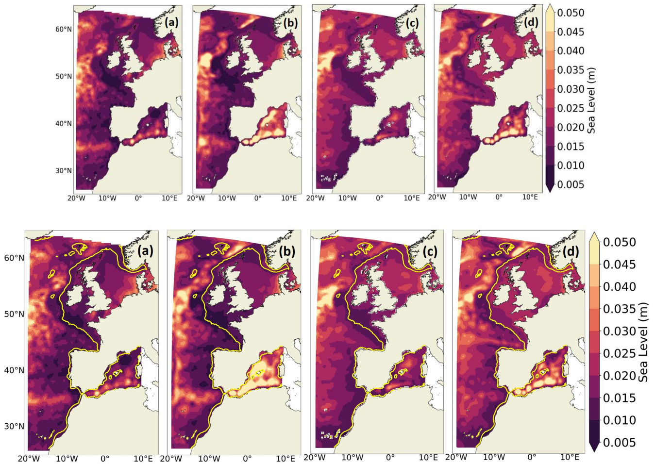
570 Figure 7: SL interannual variability over the 1993-2014 period in (a) altimetry (b) IBI-ERAi (c) CNRM-CM6-1-HR and (d) IBI-CCS_corr. The interannual variability is computed as the standard deviation of the detrended annual mean SL. Note that all panels here do not include the inverse barometer effect on sea level. The shelf break (defined by the 200 m isobath is indicated in yellow).
