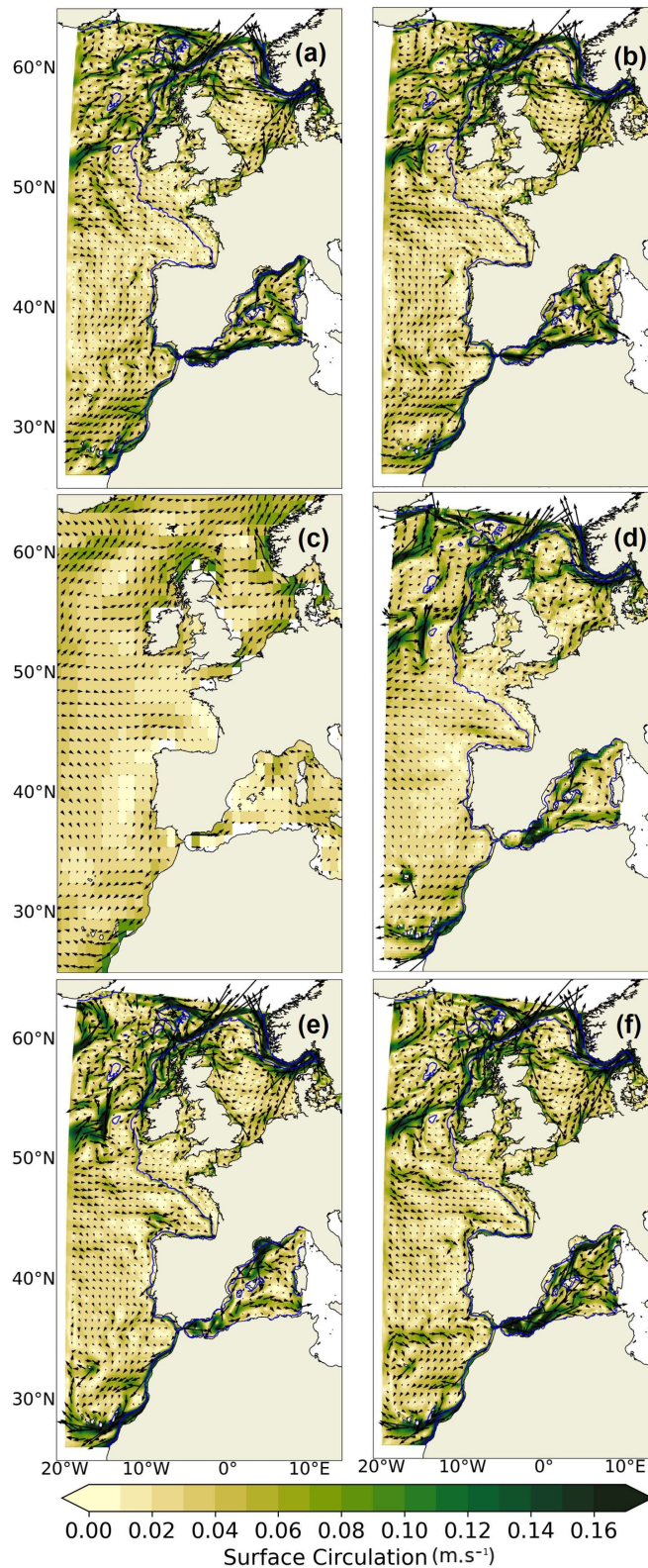
455 Figure 4: Surface circulation (in \text{m.s}^{-1} ) over the 1993-2014 period in (a) IBIRYS (b) IBI-ERAi (c) CNRM-CM6-1 (d) CNRM-CM6-1-HR (e) IBI-CCS_raw and (f) IBI-CCS_corr simulations. The shelf break (defined by the 200 m isobath is indicated in blue).
