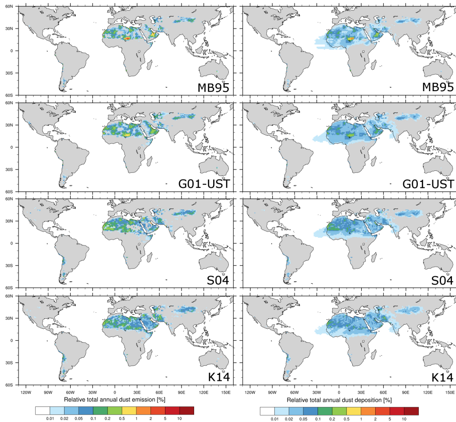
Figure A1. Percent contribution of dust emission (left column) and deposition (right column) to their respective global and annual totals for the four experiments described in Section 4.1.
