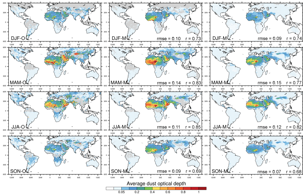
Figure 5. Seasonally averaged MODIS Deep Blue DOD (left), MONARCH all-sky \text{DOD}_{\text{coarse}} at satellite overpass times co-located with MODIS DOD (middle), and clear-sky \text{DOD}_{\text{coarse}} at approximate satellite overpass times derived from three-hourly model output from MONARCH (right). The model results were obtained for \text{DOD}_{\text{coarse}} averaged across the four model experiments. The seasonal averages were calculated with respect to the number of valid values per grid cell in the respective products. Area-weighted root-mean-square-error (rmse) and uncentered Pearson product-moment coefficient of linear correlation (r) between model and observations are indicated in the respective panels.
