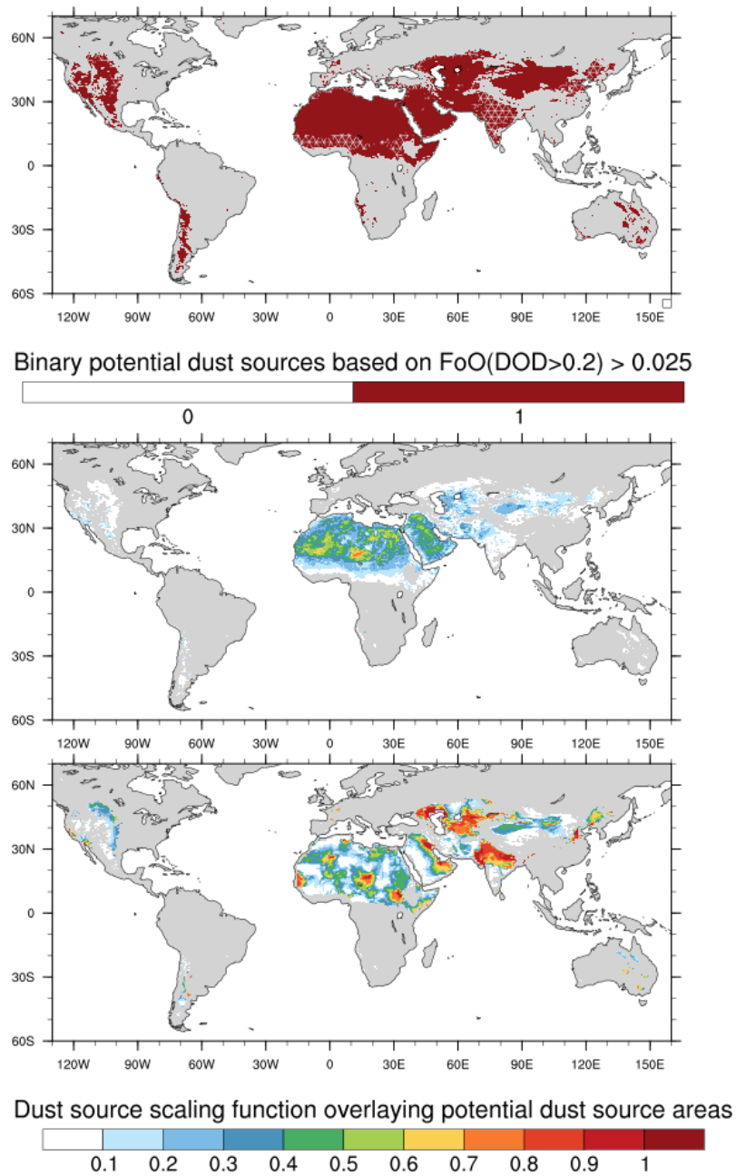
Figure 3. (Top) Binary potential dust source areas defined based on \text{FoO}(\text{DOD} > 0.2) > 0.025 ; light line patterns indicate anthropogenic dust sources using the method from Ginoux et al. (2012) considering cropland and pasture based on Klein Goldewijk et al. (2017); (Center) binary dust source overlaid with \text{FoO}(\text{DOD} > 0.2) ; (Bottom) binary dust sources overlaid with the topographic source scaling function from Ginoux et al. (2001) without vegetation mask.
