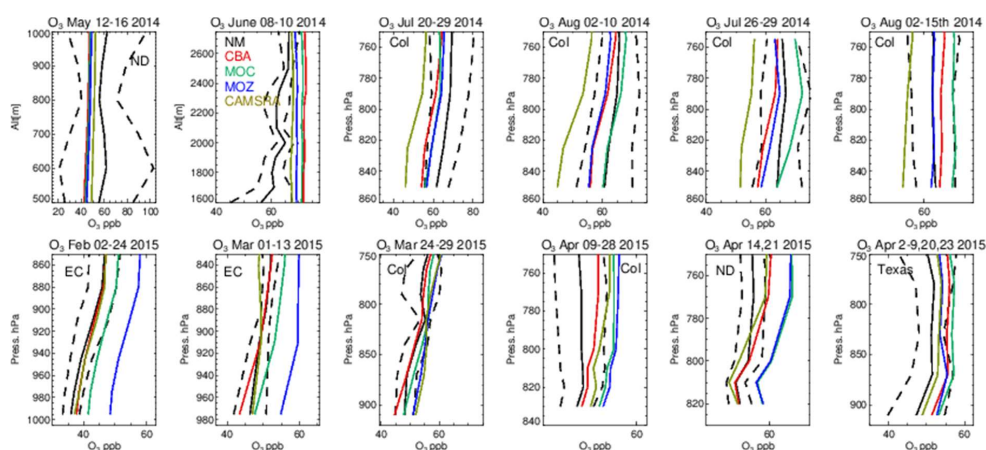
Figure 6: Comparisons of lower tropospheric O 3 profiles for 2014/2015 against composites of aircraft measurements for the regional domains shown in Figure 1. The 1- \sigma standard deviation of the mean for the observational values are shown as the dashed line. Campaigns shown (top left to bottom right) are TOPDOWN, DISCOVER-AQ, FRAPPE, WINTER and SONGNEX.
