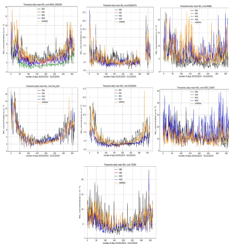
665 Figure 12. As for Fig. 5 except for surface \text{NO}_2 .
