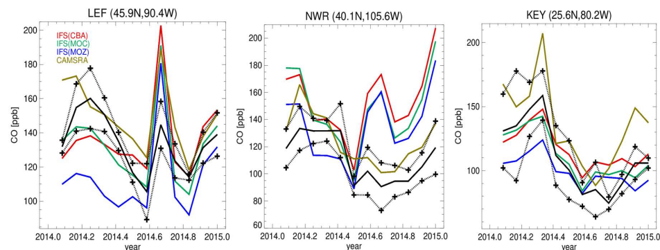
Figure 8: Comparisons of monthly mean surface CO mixing ratios at three separate surface measurement sites across the US. The observational monthly means with the variability are shown in black.
