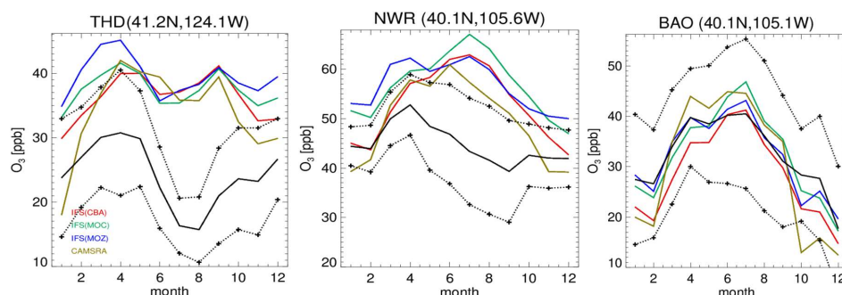
Figure 4: Comparisons of surface O_3 measurements for 2014 for the three GFDL stations situated in the US, namely: Trinidad Head (THD), Niwot Ridge (NWR) and Boulder (BAO). The color key to the various ensemble members is given in the left panel. The observational means and the corresponding 1- \sigma variability are shown as the black solid and dashed lines, respectively.
