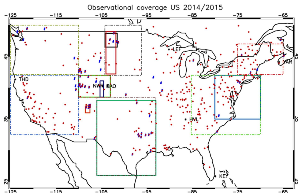
Figure 1: The location of surface measurement stations and areas sampled during the numerous aircraft campaigns Ke to air-shed: — ND (May 2014), — NM (June 2014), — Col (July/Aug 2014), — Col (July/Aug 2014; Mar/Apr 2015), — VN (Feb/March 2015) and — Texas (Apr 2015). The areas outlined by the dashed-dot borders are associated with the regions for which the AirNow observations are analysed, with the reader being referred to Table 10. The individual stations for the AirNow network are shown as the red dots ( O_3 ) and blue dots ( NO_2 ) for rural stations only, where for clarity we omit the suburban/urban stations.
