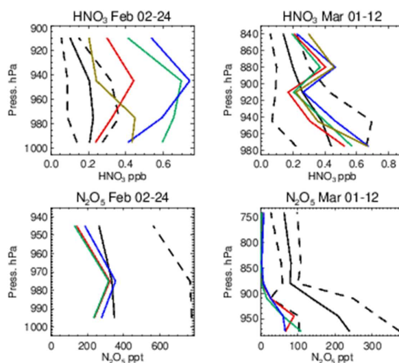
750 Figure 15. Comparisons of N 2 O 5 and HNO 3 for the WINTER campaign using nighttime flights. The black line represents the observational mean value with the associated standard deviation being shown as the dashed line.
