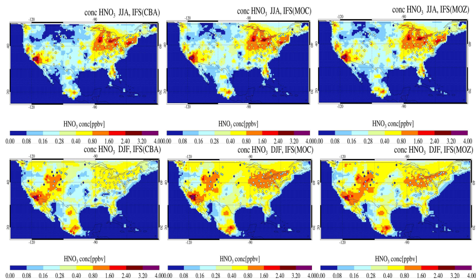
Figure 17. The Seasonal mean distribution of surface mixing ratios for gas phase \text{HNO}_3 across the US for (top) JJA and (bottom) DJF against seasonal composites of observations taken from the CASTNET network. The observational mean values and locations of the measurement stations are given as the diamonds located in each panel.
