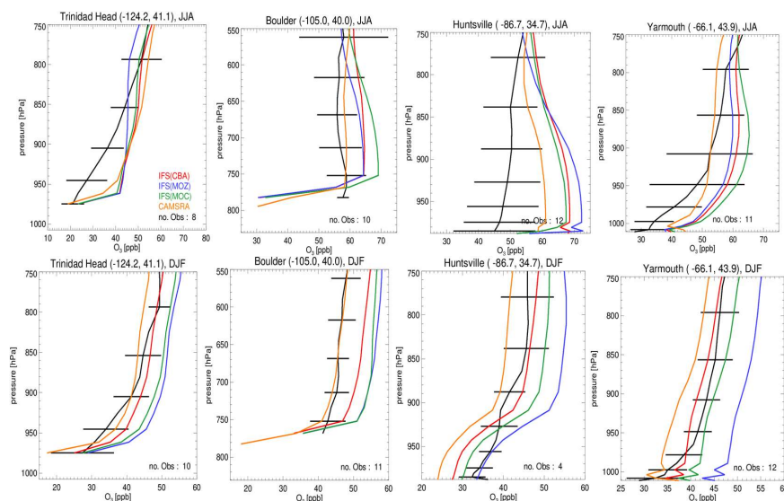
Figure 3: Seasonal O 3 sonde comparisons for seasons JJA (top) and DJF (bottom) for the lower troposphere. Stations shown are Trinidad Head, Boulder, Huntsville and Yarmouth which are situated across the US. The observational composites are shown in black, with the colour key provided in the top left panel. The geolocation of each site is given in the title of each panel and number of observations used bottom right.
