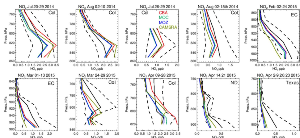
Figure 13. As for Fig. 6 except for tropospheric NO 2 . Campaigns shown (top left to bottom right) are DISCOVER-AQ, FRAPPE, WINTER and SONGNEX.
