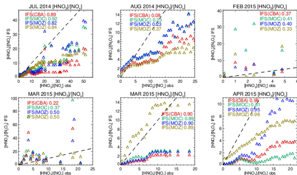
Figure 16. Comparisons of the observed [\text{HNO}_3]/[\text{NO}_x] ratio for selected months against the corresponding values from the ensemble members below 800hPa. The values are binned with respect to the observations using a bin-width of 0.75 with respect to [\text{HNO}_3]/[\text{NO}_x] and the correlation coefficients provided in each panel. Measurements are taken from FRAPPE, WINTER and SONGNEX campaigns to cover seasonality and location.
