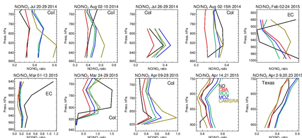
Figure 14. Comparisons of the NO/NO 2 ratio for the lower troposphere from the various aircraft campaigns, with observational values being shown in black. Campaigns shown (top left to bottom right) are DISCOVER-AQ, FRAPPE, WINTER and SONGNEX.
