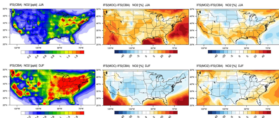
Figure 11. The horizontal mean cross-section of \text{NO}_2 below 1km over the US domain for JJA 2014 (top) and DJF (2014/2015).
