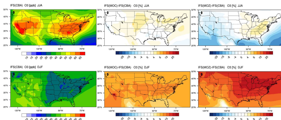
Figure 2: The horizontal seasonal mean for tropospheric O 3 below 1km over the US domain for JJA 2014 (top) and DJF 2014/2015 (bottom).
