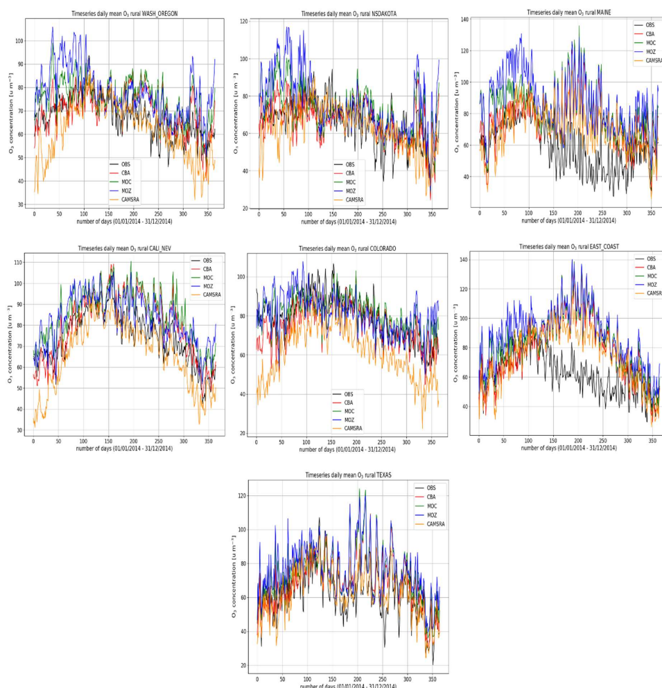
Figure 5: Comparisons of the daily mean variability surface O_3 for 2014 against regional composites assembled from measurement sites for rural locations contributing to the AirNow network. Regions shown (top left to bottom right) are Washington-Oregon, North/South Dakota, Maine, California-Nevada, Colorado, Eastern Coast, and Texas.
