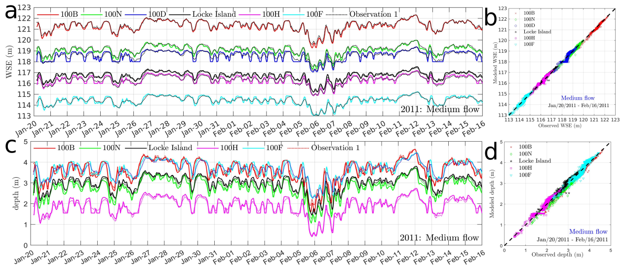
Figure 5. The comparisons of water surface elevation and depth a between the model and observations using the calibrated roughness field (case OF in Table 1) during a medium flow in 2011. a and c represent the hourly recorded WSE and depth, respectively. b and d denote their 1:1 plots. (a) An hourly-recorded WSE and (b) a 1:1 plot. Dashed color liens in (c) denote observation data. f
