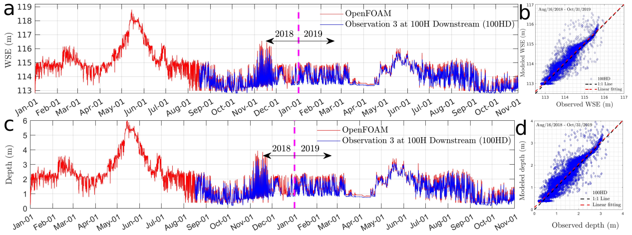
Figure 10. Long-term model validation for water surface elevation and depth a . A comparison of the hourly recorded WSE and depth a from model and observations at 100HD during 2018–2019 (a,c) and their 1:1 plots (b,d).
