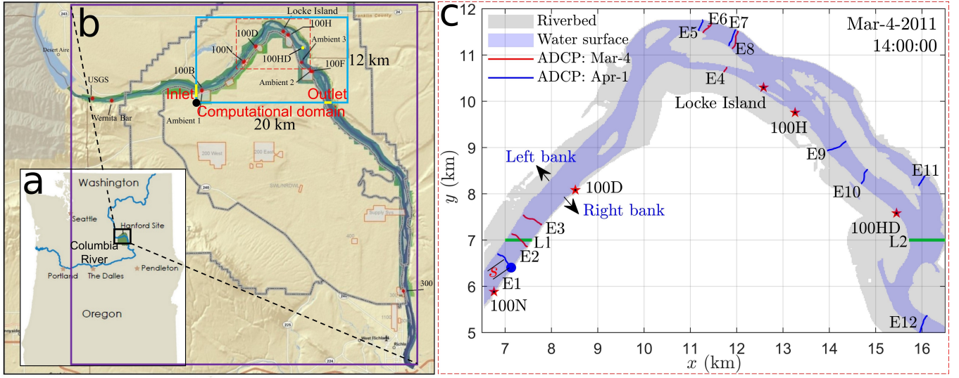
Figure 1. The location of the study site within Washington State and the Columbia River (a), the computational domain with the river bathymetry and water stage survey locations (b), and the exact a locations of velocity and stage a measurements (c). Yellow lines in (b) represent the inlet and outlet locations of the computational domain. Red and yellow dots in (b) denote water stage survey locations. Red and blues lines in (c) denote boat paths measured on two dates. Red stars and green lines in (c) represent the zoom-in of the stage survey locations in (b) and the locations (L1 and L2) selected to evaluate the sensitivity of stage and velocity variations to roughness heights, respectively. a (a) is a reused image of the Oregon Department of Energy ( www.oregon.gov/energy ); (b) is modified from Figure 1 in Niehus et al. (2014) produced by S. Kallio at Pacific Northwest National Laboratory.
