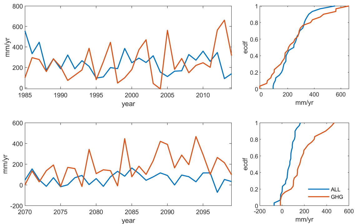
Figure A3. 30-year Mean annual runoff time series and eCDF from all forcing and GHG-only forcing simulations for historical period (upper panel), and SSP5-8.5 period(lower panel) at (9.5 ° S, 40.5 ° W) , where the K-S test was fail to reject (F) in the historical period and rejected (R) in the SSP5-8.5 period.
