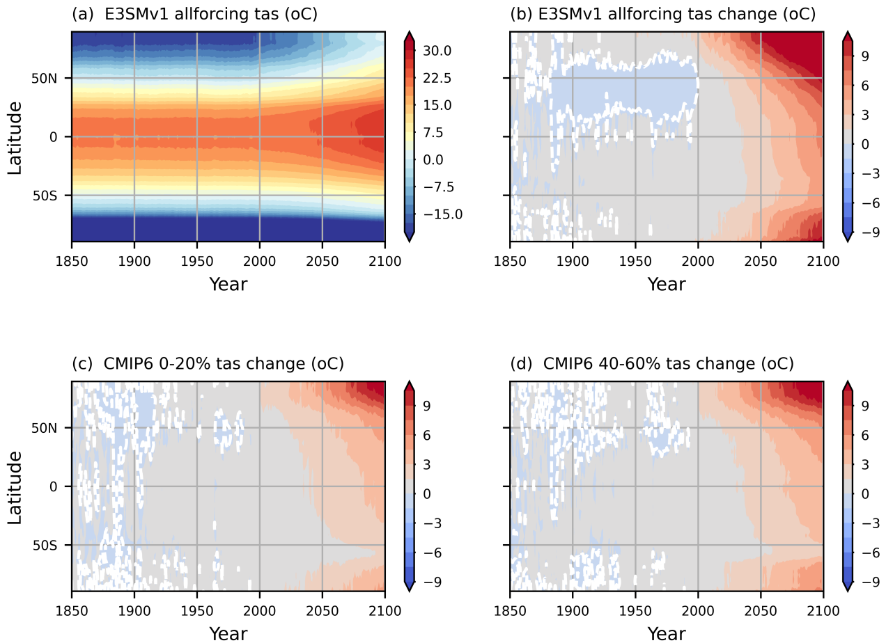
Figure 5. Time evolution of zonal mean (a) E3SMv1.0 annual ( T_{air} ) anomalies. Time evolution of the local changes in zonal mean T_{air} with respect to 1850-1869 from the historical simulations and SSP5-8.5 simulations for (b) E3SMv1.0, (c) CMIP6 models within the 0 – 20th percentile range, and (d) CMIP6 models within the 40 – 60th percentile range based on Fig. 1(c)
