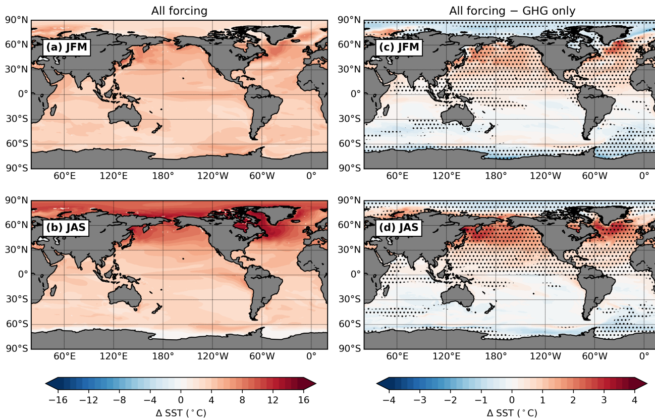
Figure 9. Left panels show the changes of the ensemble averaged SST ( ^\circ\text{C} ) between the period of 2070-2099 and 1985-2014 in (a) Jan., Feb. and Mar. (JFM), and (b) Jul., Aug. and Sep. (JAS) in the E3SMv1.0 all-forcing simulations. Right panels show the differences in the SST change between all-forcing simulations and GHG-only simulations. Dots in panels (c) and (d) highlight the regions where such differences are significant as compared to the variations among ensemble members. See the text for more details on how the significance is quantified.
