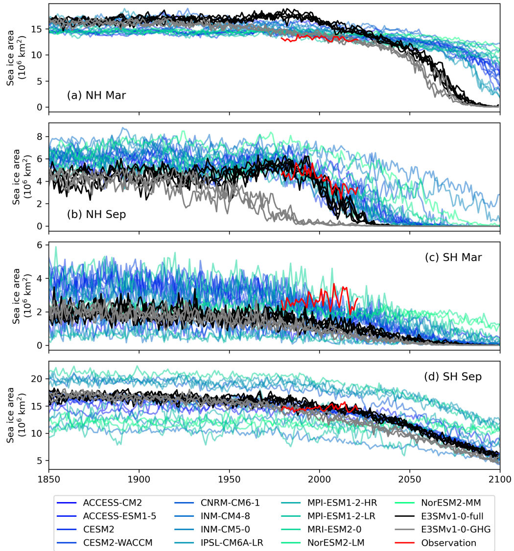
Figure 13. Same as Fig. A, but for (a,b) the Northern Hemisphere and (c,d) Southern Hemisphere sea ice area ( 10^6 \text{ km}^2 ) in (a,c) March and (b,d) September. The observation is from the National Snow and Ice Data Center Sea Ice Index Version 3 (Fetterer et al., 2017). A different set of CMIP6 simulations is used as a reference due to data availability.
