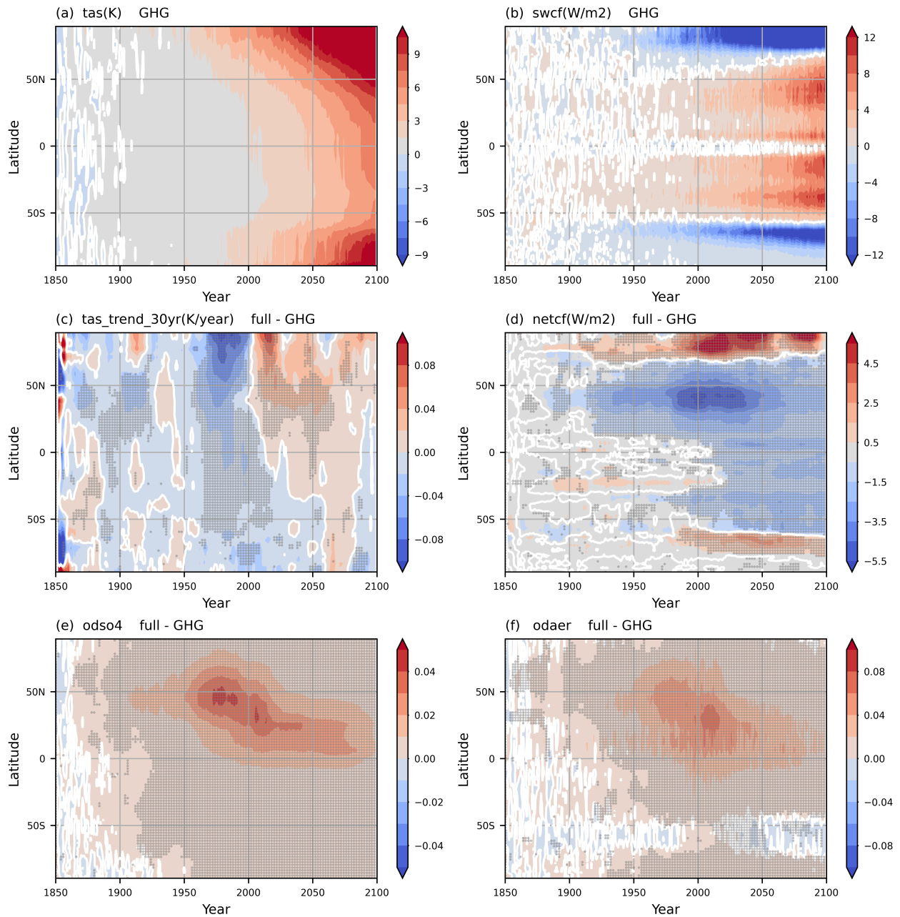
Figure 15. The time evolution of the zonal mean local (a) T_{air} change (K), (b) SW cloud radiative forcing ( W/m^2 ) in E3SMv1.0 GHG-only simulations, and the simulated differences in (c) T_{air} trend ( K/year ), (d) net cloud radiative forcing ( W/m^2 ), (e) Sulfate aerosol optical depth at 550 nm, and (f) total aerosol optical depth at 550 nm between E3SMv1.0 all-forcing simulations and GHG-only simulations. Stippled regions in (c-f) indicate where the difference reaches the 95% confidence level based on a two-tailed Student's t test.
