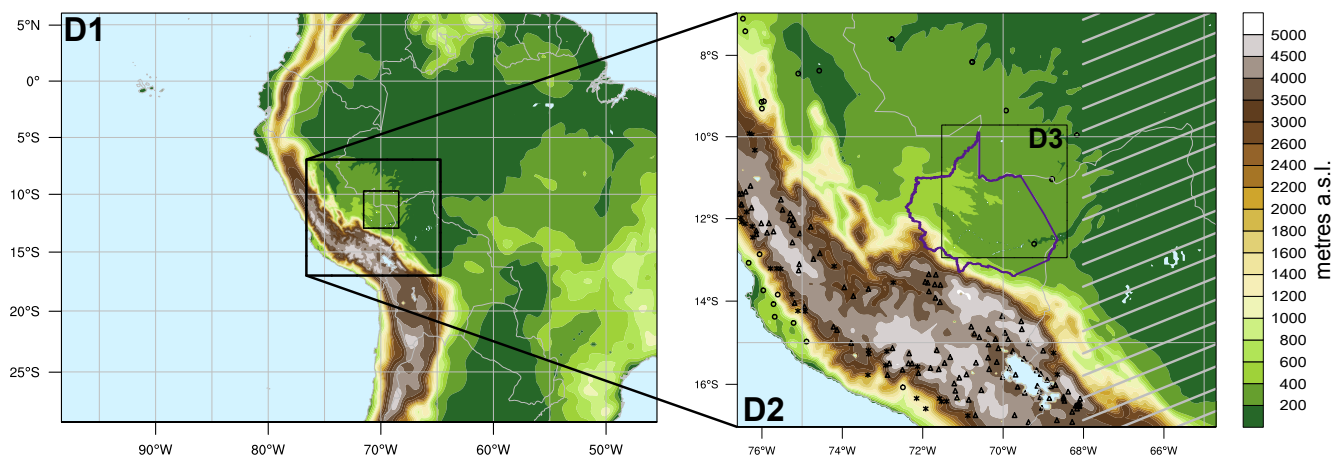
Figure 1. The three nested domain setup employed in all the WRF experiments is depicted on the left. A nesting ratio of 1:5 is used, which means that the spatial resolution of the largest domain is 25 km, followed by another domain with 5 km spatial resolution, and the innermost domain focusing over the region of Madre de Dios with 1 km horizontal resolution. The colour shading indicates elevation in metres above sea level (a.s.l.) using the WRF topography Global Multi-resolution Terrain Elevation Data (GMTED2010) provided by USGS. Domain 2 is presented in detail on the right, where the weather stations for the year 2008 are presented. The stations in the flatlands (< 1000 metres a.s.l.) are depicted with a circle, the ones in the slopes of the Andes (1000–3000 metres a.s.l.) with an asterisks, and finally, stations in the plateau (> 3000 metres a.s.l.) are marked as triangles. The grey striped area highlights the region that is not included in the analysis against PISCO, since this data set is only available over a rectangle around Peru. The purple line borders the department of Madre de Dios.
