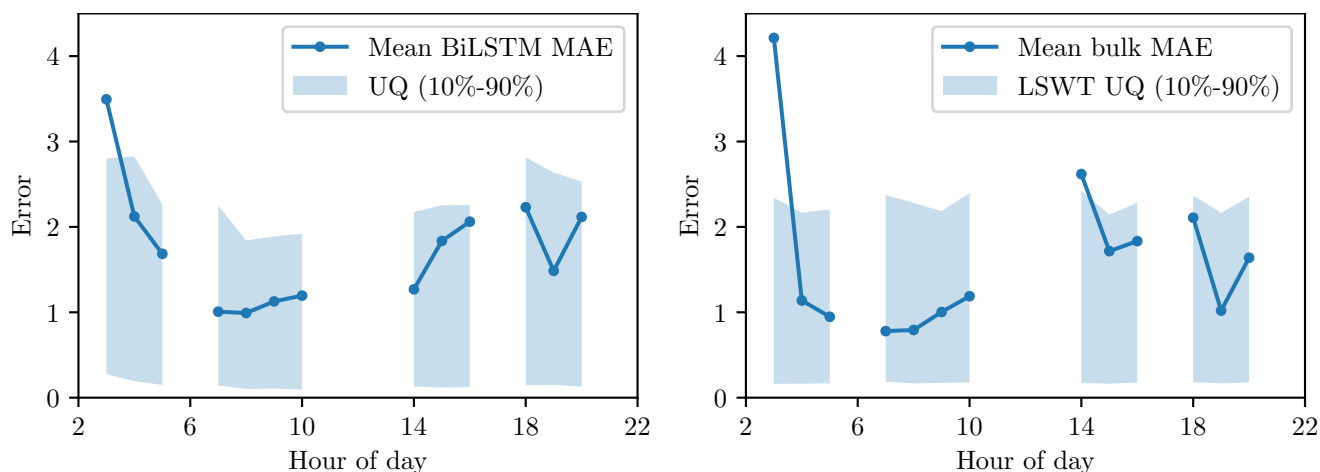
Figure 12. Left: mean BiLSTM prediction error (dark blue line) and the 10%-90% percentiles of the uncertainties predicted by Bi-LSTM (shaded areas) for the different hours of the day. Right: mean bulk temperature prediction error (dark blue line) and the 10%-90% uncertainty estimates based on Lieberherr and Wunderle (2018).
