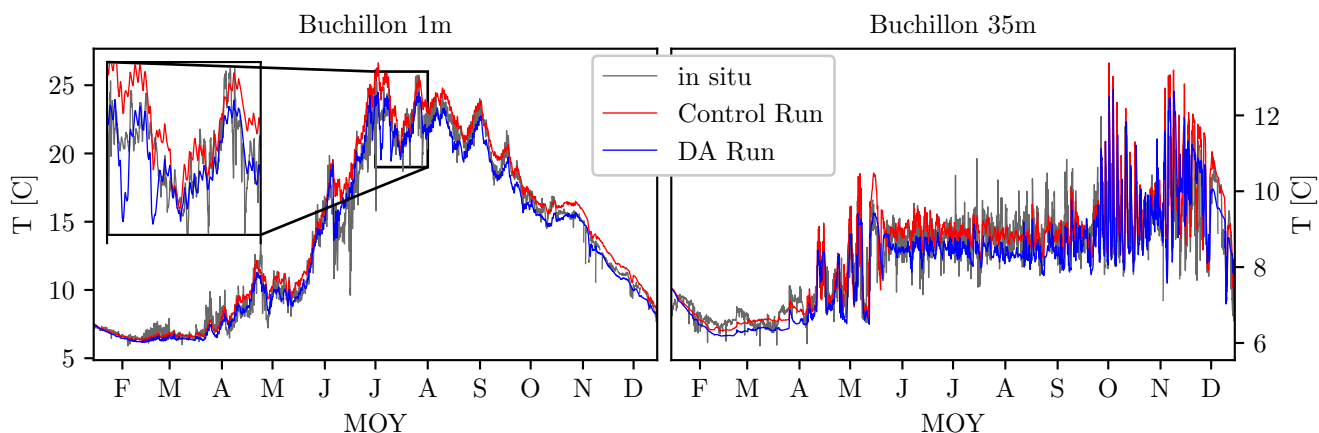
Figure 6. Evolution of temperature at the Buchillon station for the 1m (left) and 35m (right) sensors for the year 2019. The gray line is the in situ measurement, the red line corresponds to the control run, and the blue line is the data assimilated prediction. The small inset on the left shows the improvement from the assimilated run for the 1m sensor in greater detail for July.
