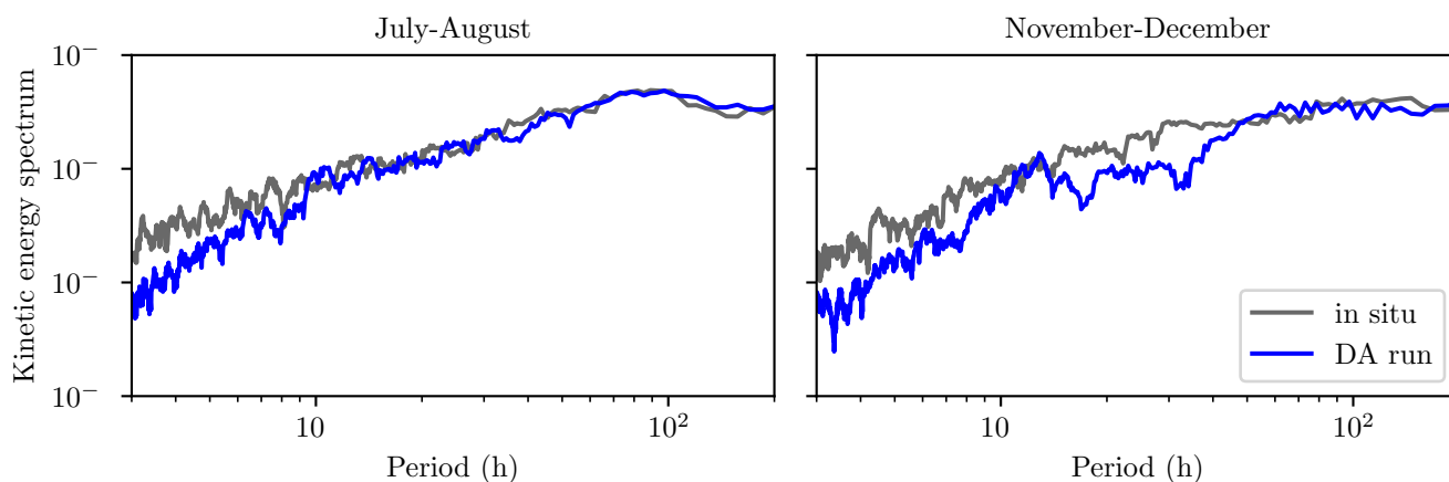
Figure 9. Kinetic energy spectra computed from the ADCP sensors at the LÉXPLORE platform (gray) and from the DA run (blue). Profiles based on 15 meter deep dynamics use July-August data for the left figure and November-December data for the right figure.
