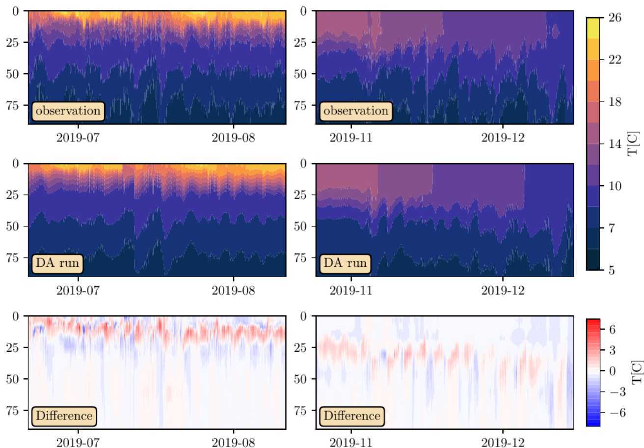
Figure 8. Vertical temperature profiles from the LÉXPLORE sensors for summer months (left) and late autumn (right). The top row shows the dataset, the middle row shows the assimilated predictions. The bottom row shows the difference between the plots, with positive values indicating model over-prediction.
