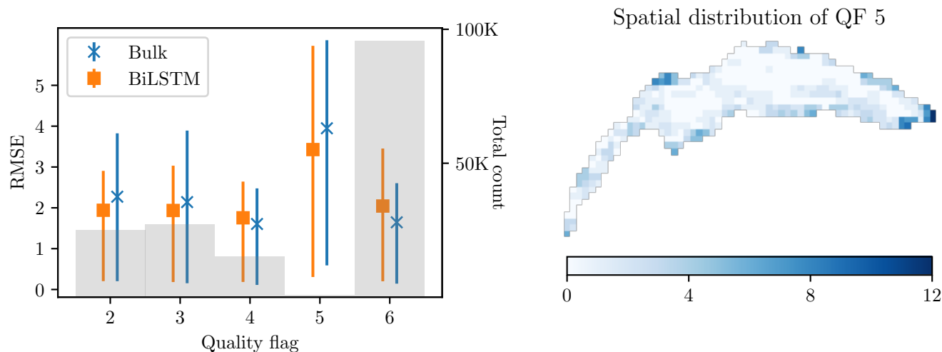
Figure 11. Analysis of Bi-LSTM performance in the DA run with respect to the different quality flags. Left: LSWT difference with respect to bulk temperature (in blue) and BiLSTM predictions (in orange) as a function of QF. The faint gray bars show the total number of LSWT measurements associated with the QF. Right: spatial distribution of LSWT measurement availability for QF 5.
