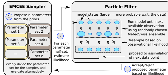
Figure 2. A visualization of the data assimilation framework. The EMCEE sampler proposes n parameters, whose likelihood is then evaluated using the particle filter and used to determine whether to update that particular parameter.
