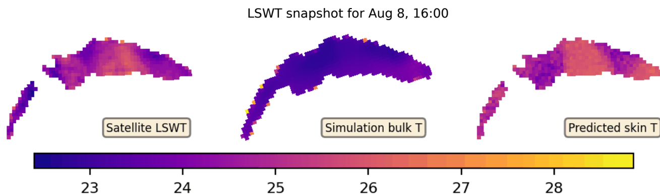
Figure 10. A comparison of LSWT snapshot from August 8, 2019 to the DA bulk and BiLSTM skin temperature predictions.
