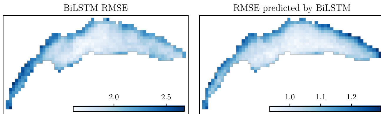
Figure 13. Spatial distribution for the BiLSTM RMSE (left) and the RMSE predicted by the BiLSTM.
