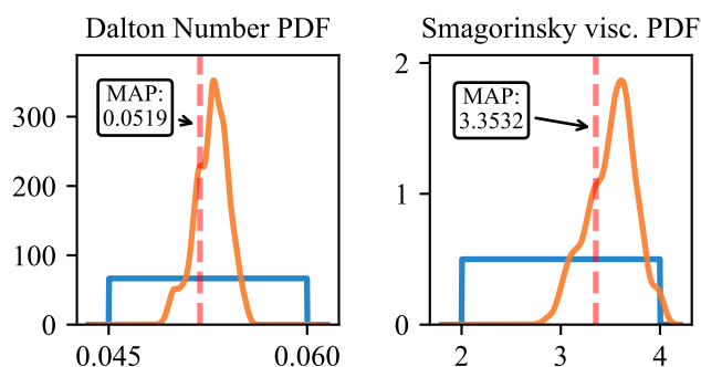
Figure 4. Marginal posterior (orange) and prior (blue) distributions of model parameters. The red dashed line indicates the maximum a posteriori parameter (MAP).
