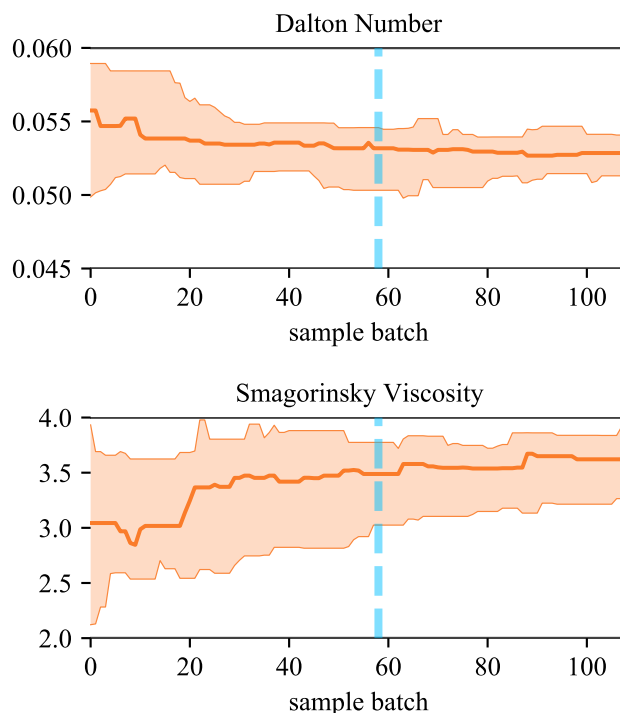
Figure 3. Evolution of the 16 Markov chain parameters. The solid lines indicate the median and the semi-transparent spreads indicate the 5% - 95% percentiles across multiple concurrent chains of the sampler. The vertical dashed blue line indicates the end of the specified burn-in period used to determine the posterior distribution.
