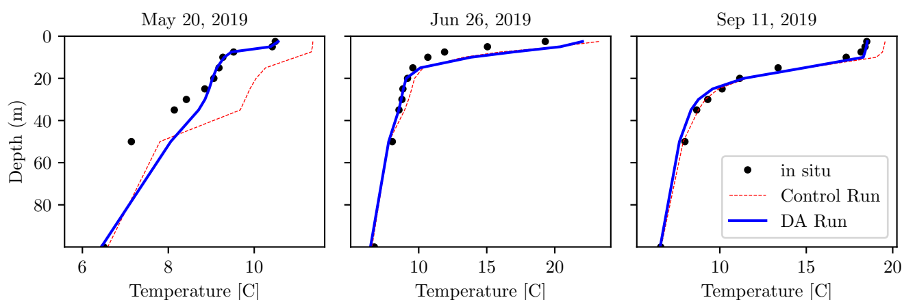
Figure 7. Vertical temperature profiles up to 100 meters deep at the SHL2 location. The black dots represent observations, the dashed red line is the control run, and the blue line shows the data assimilated run.
