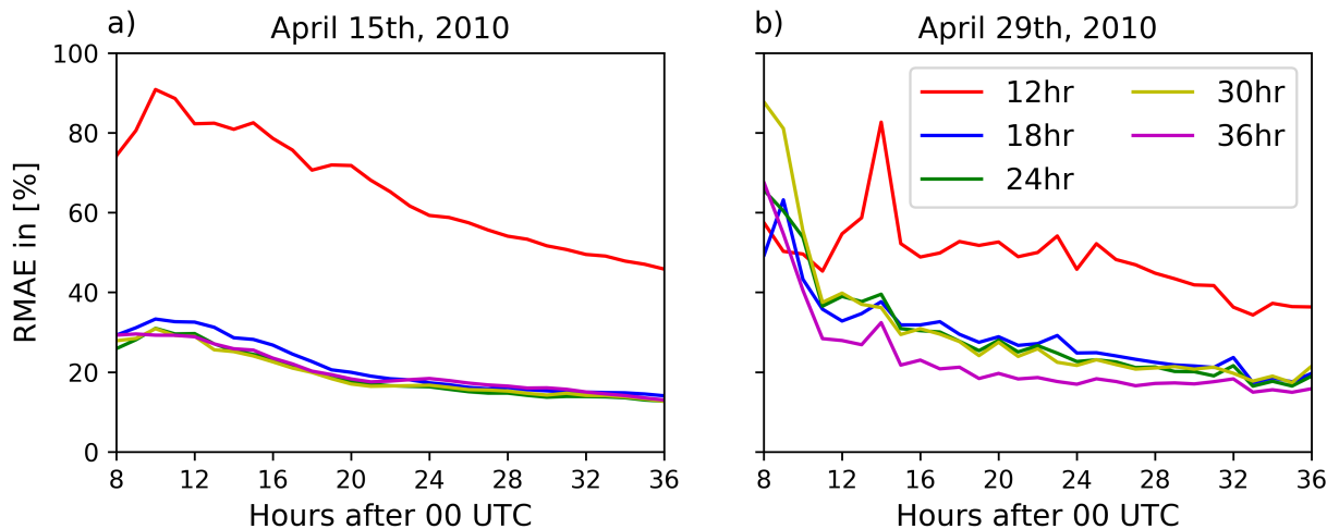
Figure 8. Relative mean absolute error of the volcanic ash concentrations defined by (9) for the eruption on (a) 15 April 2010 and on (b) 29 April 2010. The different lines indicate different assimilation window lengths from 12 hours (red) to 36 hours (magenta) as defined by Fig. 3.
