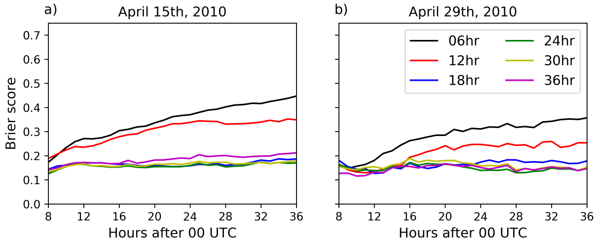
Figure 13. Brier score as calculated by (10) for each hour and all assimilation window lengths for (a) 15 April and (b) 29 April 2010.
