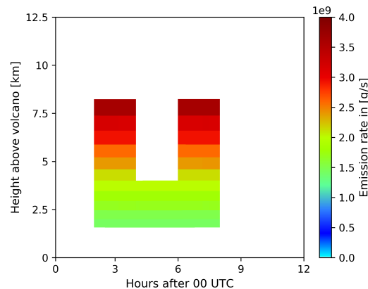
Figure 2. Hovmoeller-like plot of the volcanic ash emission profile used in the nature run to generate the synthetic observations simulating SEVIRI-like column mass loading data for the ESIAS-chem system tests. Shown is the emission rate (colored) for a given time (x-axis) and height above the volcano (y-axis).
