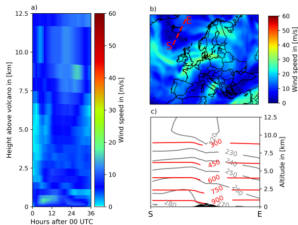
Figure 5. Meteorological conditions on 29 April 2010. (a) Wind speed above the volcano for the whole simulation period. (b) Wind speed at 500 hPa on 29 April 2010, 12 UTC, which corresponds to approx. 5 km above the volcano. (c) Vertical cross-section of isobars in [hPa] (red) and isotherms in [K] (grey) along the red line in b) on 29 April 2010, 12 UTC.
