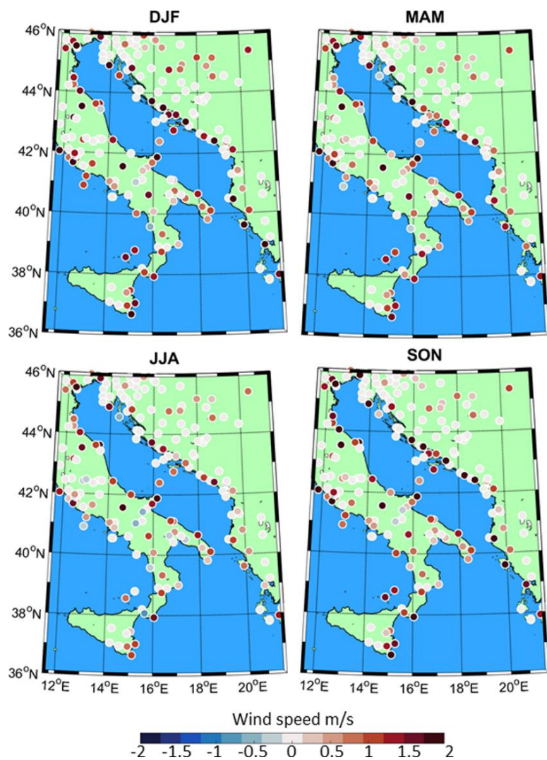
Figure 14. As in Fig. 109 but for the hourly wind speed bias.
