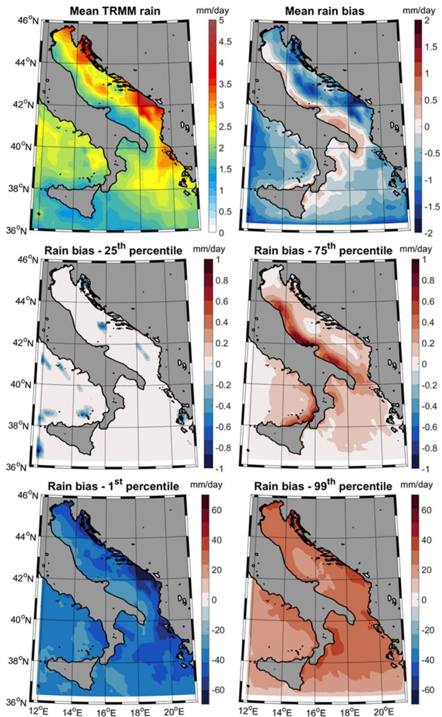
935 Figure 9. As in Fig. 3 but for the daily TRMM rain remote sensing data over the sea during the 1998-2017 period.
