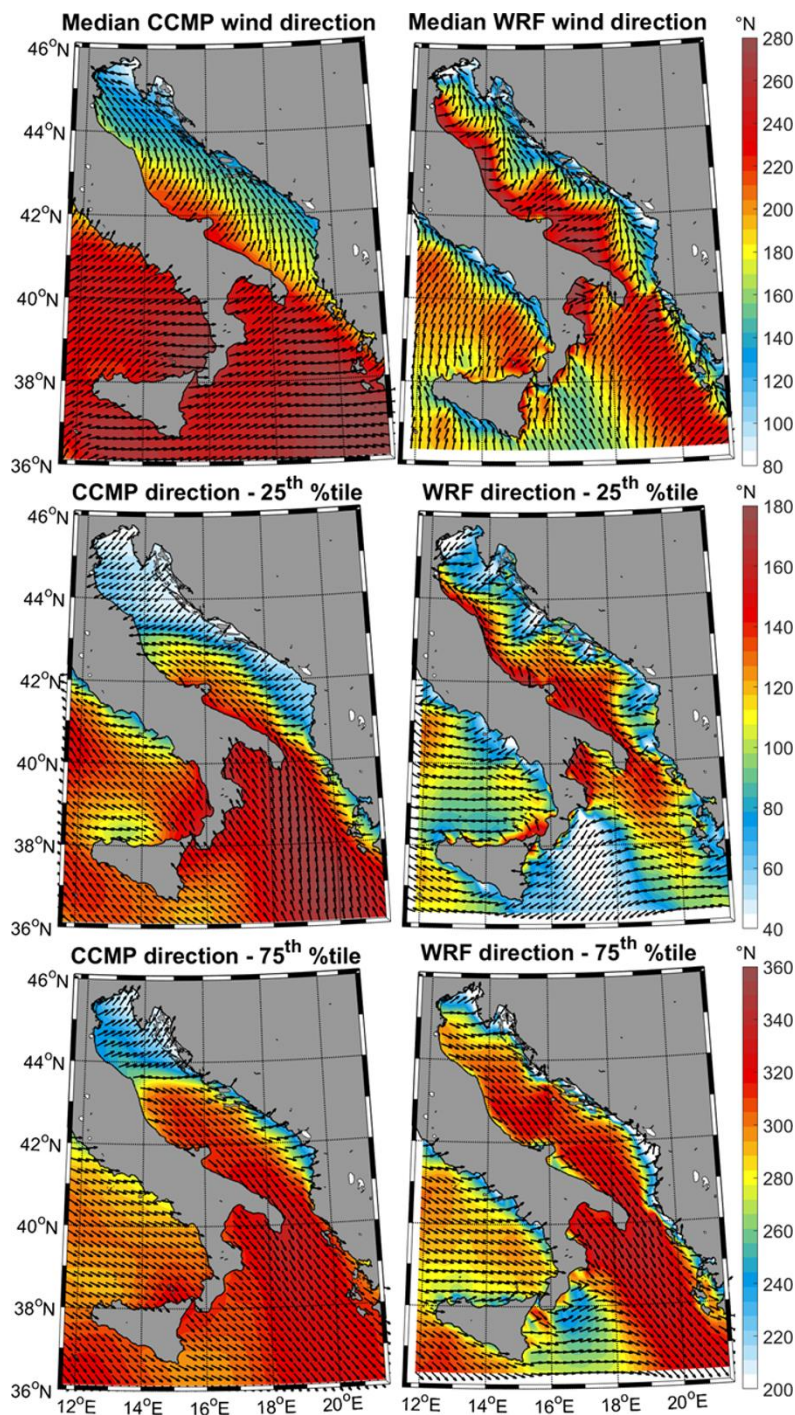
Figure 8. Median as well as the 25 th and 75 th percentilesAs in Fig. 3 but of for the 6-hourly CCMP wind direction (as colour fields and black vectors) over the sea for both CCMP remote sensing data (left panels) and AdriSC WRF 3-km results (right panels) during the 1987-2017 period, over the sea.
