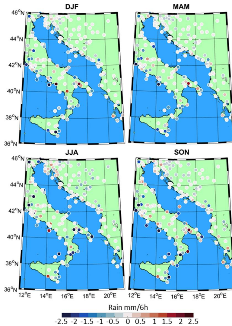
Figure 12. As in Fig. 109 but for the mean 6-hourly rain bias.
