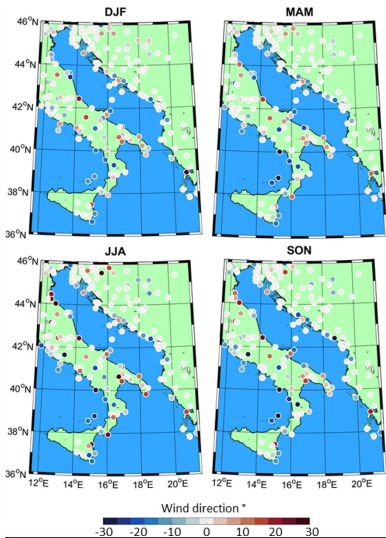
Figure 15. As in Fig. 109 but for the hourly wind direction bias (i.e. shift in direction, positive clockwise).
