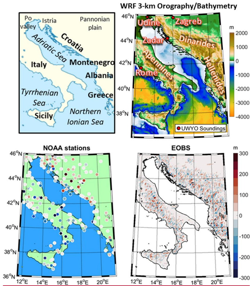
Figure 1. Name of the geographical (top left panel) and orographic topographical /bathymetric (top right panel) features of the AdriSC WRF 3-km model domain, location of the UWYO soundings (top right panel) and biases between the AdriSC WRF 3-km orography and both the NOAA stations (bottom left panel) and the E-OBS dataset (bottom right panel) elevations.
