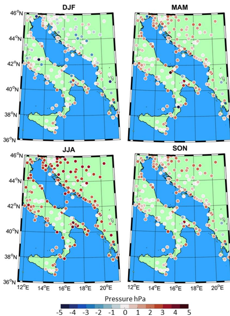
Figure 13. As in Fig. 109 but for the hourly pressure bias.
