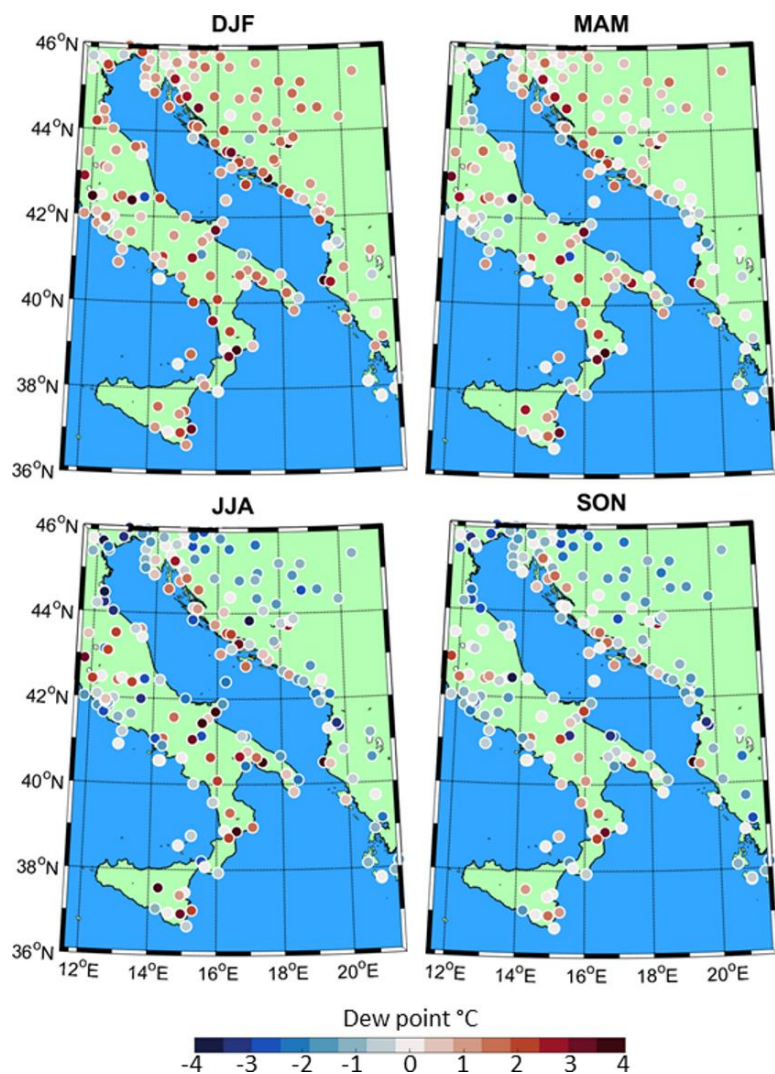
940 Figure 11. As in Fig. 109 but for the hourly dew point bias.
