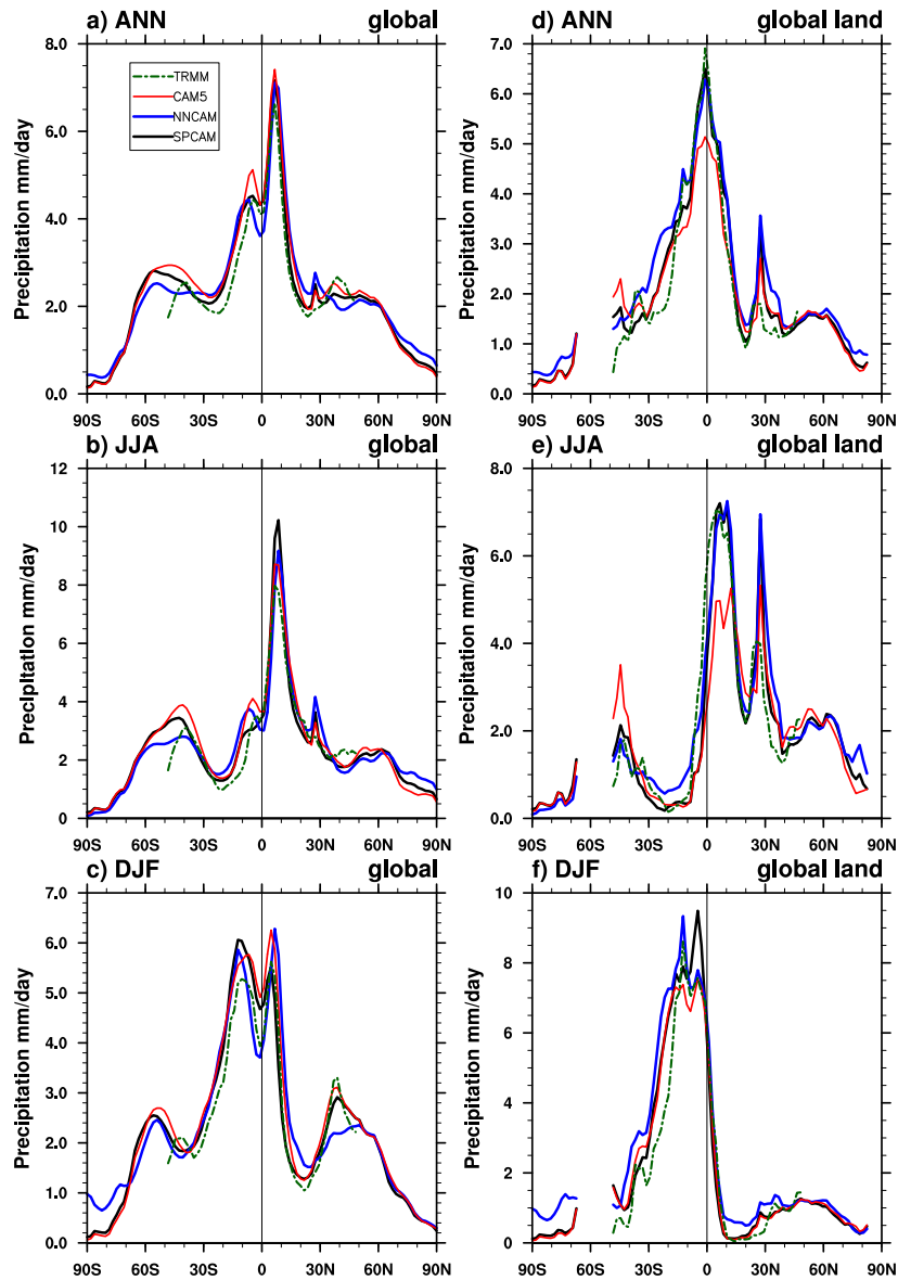
755 Figure 12. The zonal mean precipitation rate (mm/day) averaged from 1999 to 2003 for (a, d) the annual mean, (b, e) June- July-August, and (c, f) December-January-February. The black, blue, and red solid lines denote SPCAM, NNCAM, and CAM5, respectively. The dark green dashed line denotes the averaged results of the TRMM 3B42 daily rainfall product.
