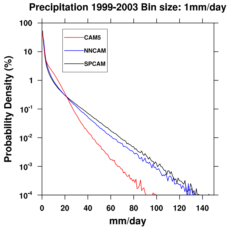
760 Figure 13. Probability densities of the daily mean precipitation in the tropics ( 30^{\circ}\text{S} – 30^{\circ}\text{N} ) obtained from the three model simulations. The black, blue, and red solid lines denote SPCAM, NNCAM, and CAM5, respectively.
