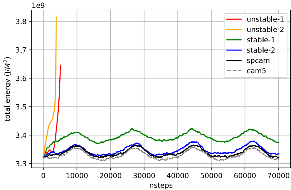
Figure 5. Time evolution of the globally averaged column of the integral total energy of NNCAM with different ResDNN- 715 parameterizations (marked with the same colors as in Figure 4), SPCAM target (black line), and CAM5 control run (grey dashed line). The blue line indicates the stable and accurate ResDNN, the green line indicates the stable but deviating ResDNN, and the orange and red lines indicate unstable ResDNNs.
