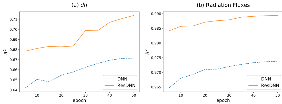
Figure 2. Fitting accuracies ( R^2 ) of both the proposed ResDNN (solid orange lines) and the DNN (dashed blue lines) for different outputs. (a) The R^2 of the moist static energy changing rate ( dh ) versus the training epochs; and (b) the fitting accuracy of the average R^2 for the eight radiation fluxes. Note: the R^2 values are calculated for both space and time in the validation dataset.
