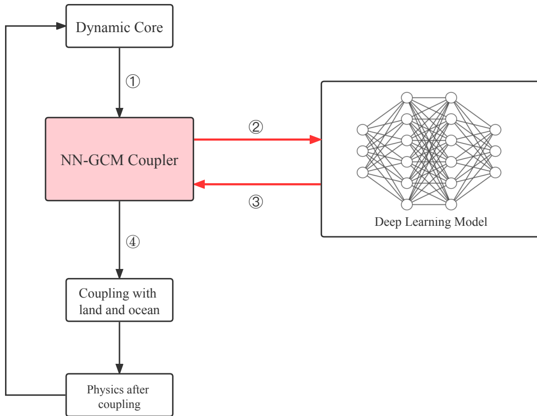
700 Figure 3. A flow chart of NNCAM, including the NN-GCM coupler. NNCAM runs in the direction of the arrow, and each box represents a module. Among them, the NN-GCM coupler is indicated by the pink box. The NN-Parameterization is shown in the box on the right. ① The dynamic core transmits data to the NN-GCM coupler; ② and ③ the data communication between the NN-GCM coupler and the NN-Parameterization; and ④ the host GCM accepts the results from the NN- Parameterization.
