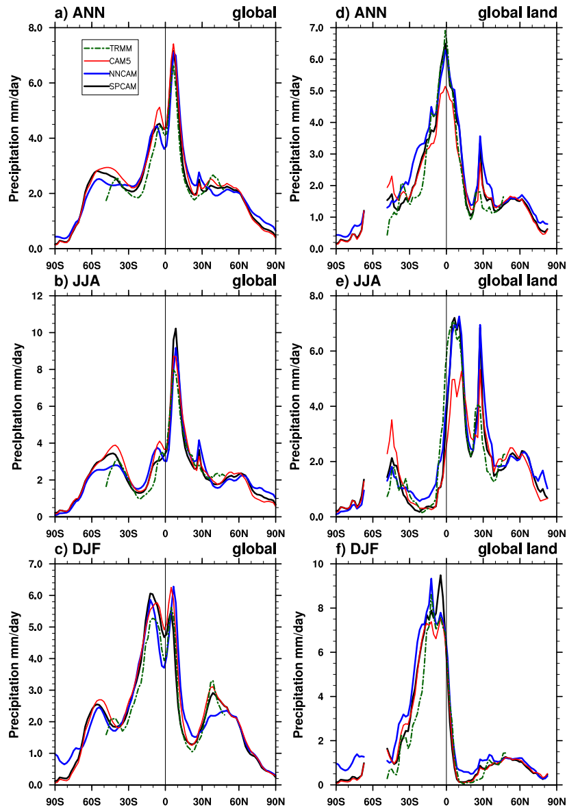
755 Figure 12. The zonal mean precipitation rate (mm/day) averaged from 1999 to 2003 for (a, d) the annual mean, (b, e) June-July-August, and (c, f) December-January-February. The black, blue, and red solid lines denote SPCAM, NNCAM, and CAM5, respectively. The dark green dashed line denotes the averaged results of the TRMM 3B42 daily rainfall product.
