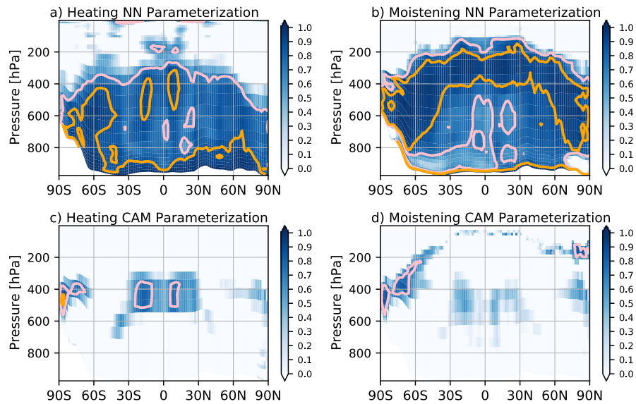
Figure 7. Latitude-pressure cross sections of the coefficient of determination ( R^2 ) for the zonally averaged heating (left panels) and moistening (right panels) predicted using (a & b) the NN-Parameterization in the offline one-year SPCAM run, and (c & d) the offline CAM5 parameterizations. Both were evaluated at a 30-min time step interval. Note: the areas where R^2 is greater than 0.7 are contoured in pink, and the areas where R^2 is greater than 0.9 are contoured in orange.
