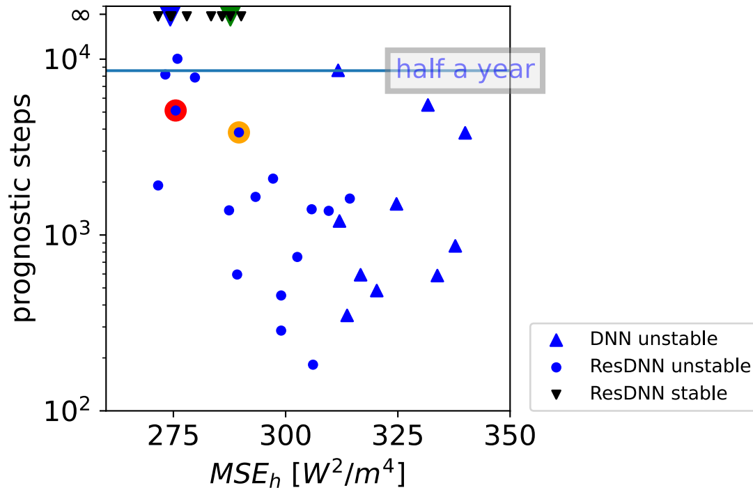
Figure 4. The mean square error of the offline moist static energy vs. the prognostic steps. The black inverted triangles (10 in total but some overlap due to their close MSE_h values) denote stable NN coupled prognostic simulations that last for more than 10 years. The blue dots denote unstable simulations, and the blue triangles denote unstable DNNs. The dots with colored outlines are shown in Figure 5 for the time evolution of the globally averaged energy.
