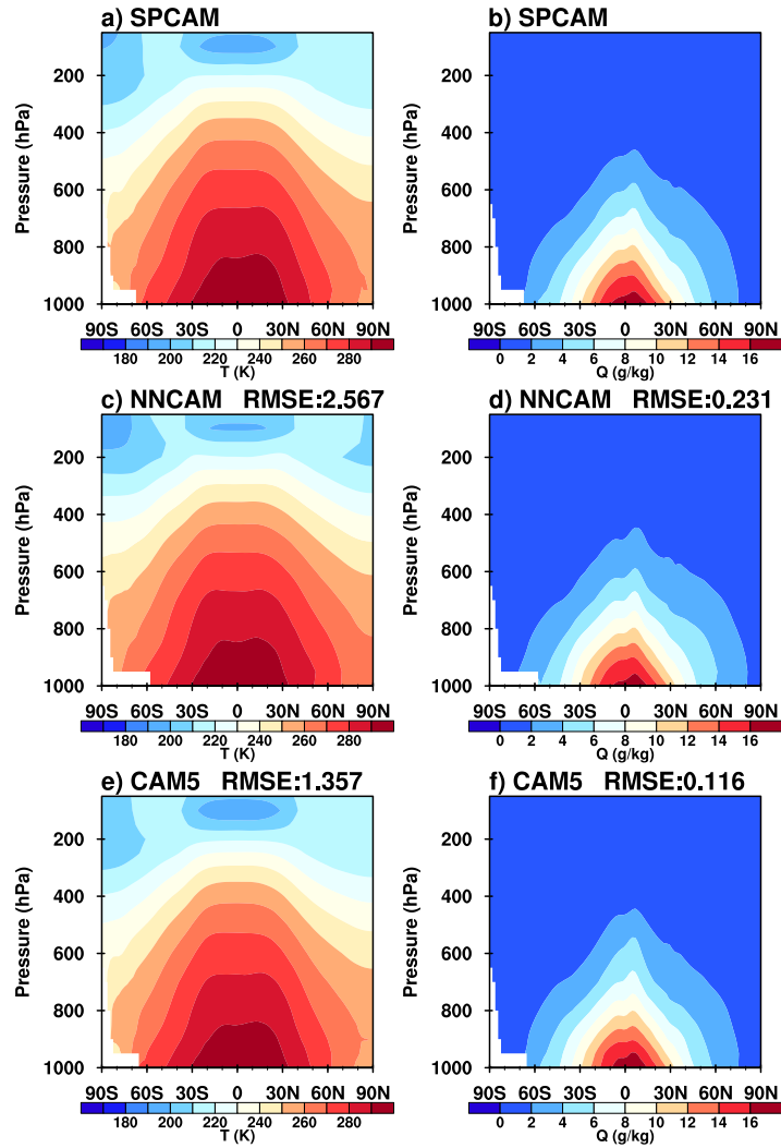
740 Figure 9. Latitude-pressure cross sections of the zonal mean temperature (left panels) and specific humidity (right panels) averaged from 1999 to 2003 predicted using (a, b) SPCAM, (c, d) NNCAM, and (e, f) CAM5.
