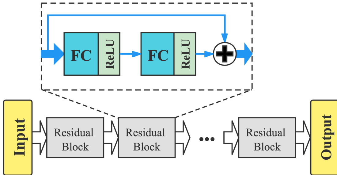
Figure 1. Schematic diagram of the structure of the ResDNN. It consists of seven residual blocks, each of which (dashed box) contains two 512 node-wide dense (fully connected) layers with an ReLU as the activation and a layer jump. The inputs and outputs are discussed in Section 2.2.2.
