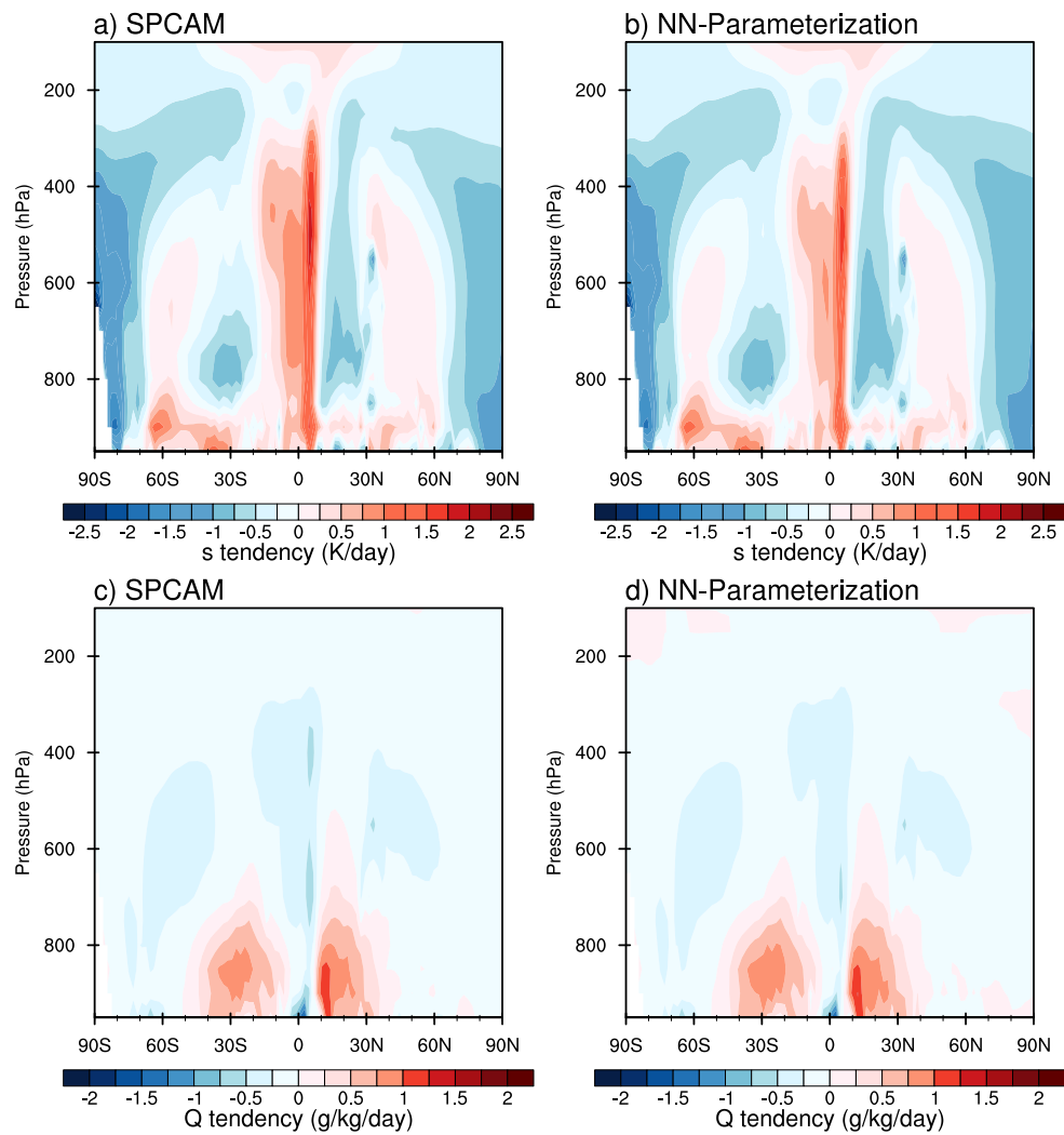
Figure 6. Latitude-pressure cross sections of the annual and zonal mean heating (top) and moistening (bottom) due to moist physics during the year 2000 for (a, c) SPCAM simulations, and (b, d) the offline test using the NN-Parameterizations.
