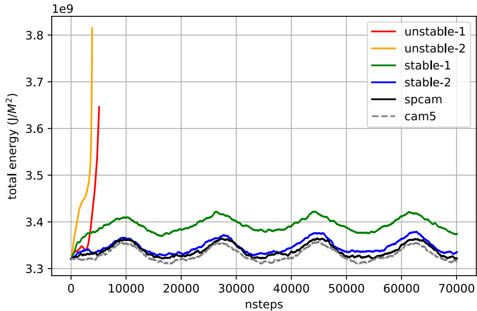
715 Figure 5. Time evolution of the globally averaged column of the integral total energy of NNCAM with different ResDNN-parameterizations (marked with the same colors as in Figure 4), SPCAM target (black line), and CAM5 control run (grey dashed line). The blue line indicates the stable and accurate ResDNN, the green line indicates the stable but deviating ResDNN, and the orange and red lines indicate unstable ResDNNs.
