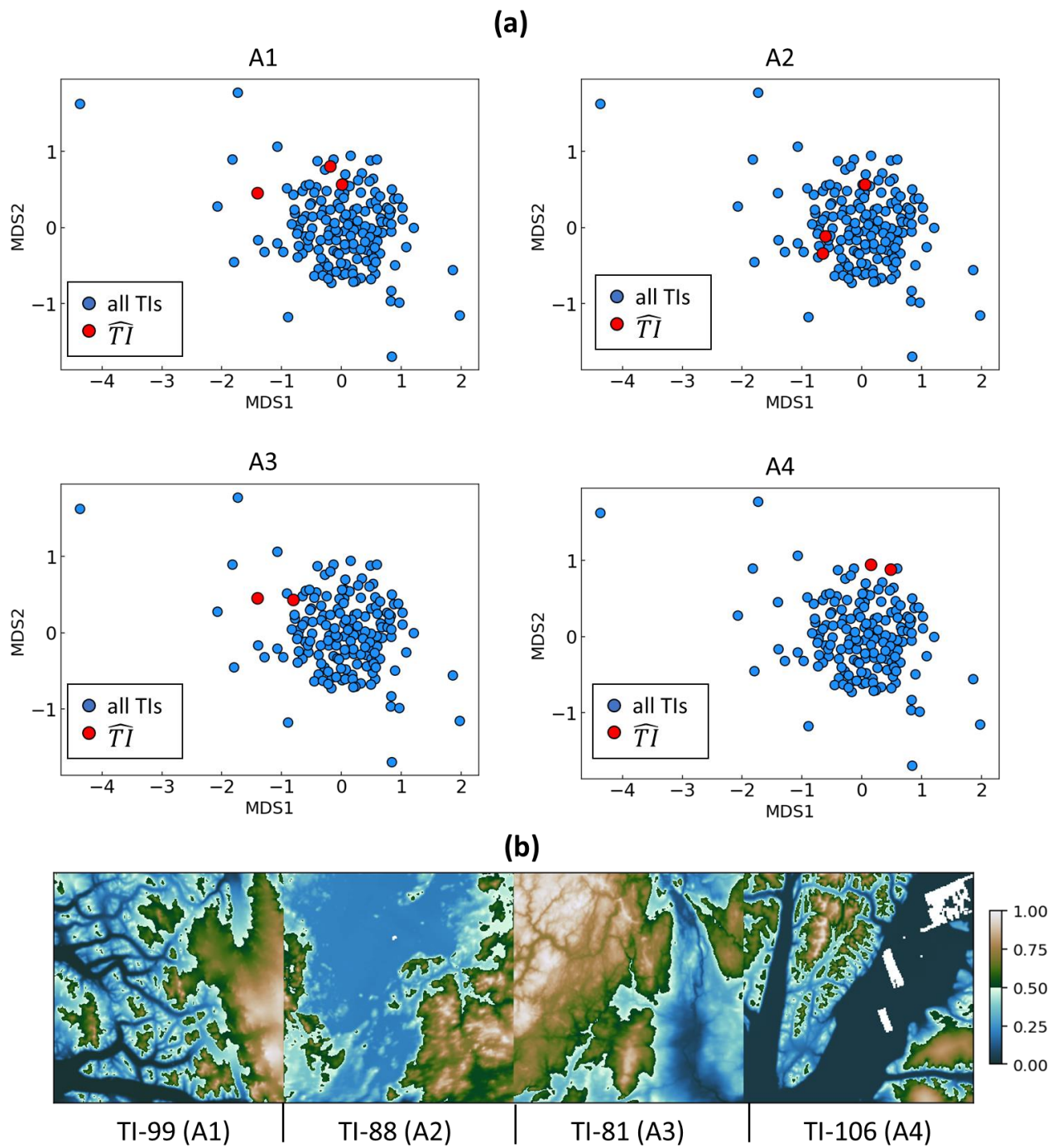
315 Figure 8. (a) The estimated set of most probable training images \hat{T}I on MDS plots for for each subarea (A1, A2, A3, A4). The red dots highlight the estimated \hat{T}I . (b) Examples of \hat{T}I displayed in the topographic modeling space.
