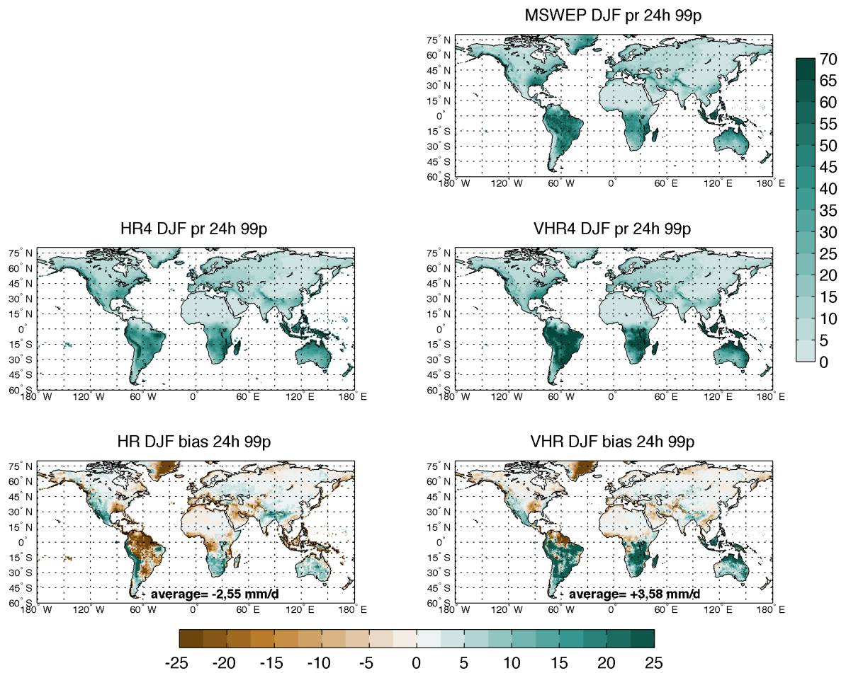
455 Figure 5: Winter (DJF) Extreme Precipitation (99th percentile, 99p) computed at the daily frequency. Upper panel shows MSWEP observational results. Central panels show model results (HR on the left and VHR on the right) and lower panels show the relative model bias. Units are [mm/d]. Vertical colorbar refers to the three upper panels, while the horizontal colorbar refers to the two bottom panels.
