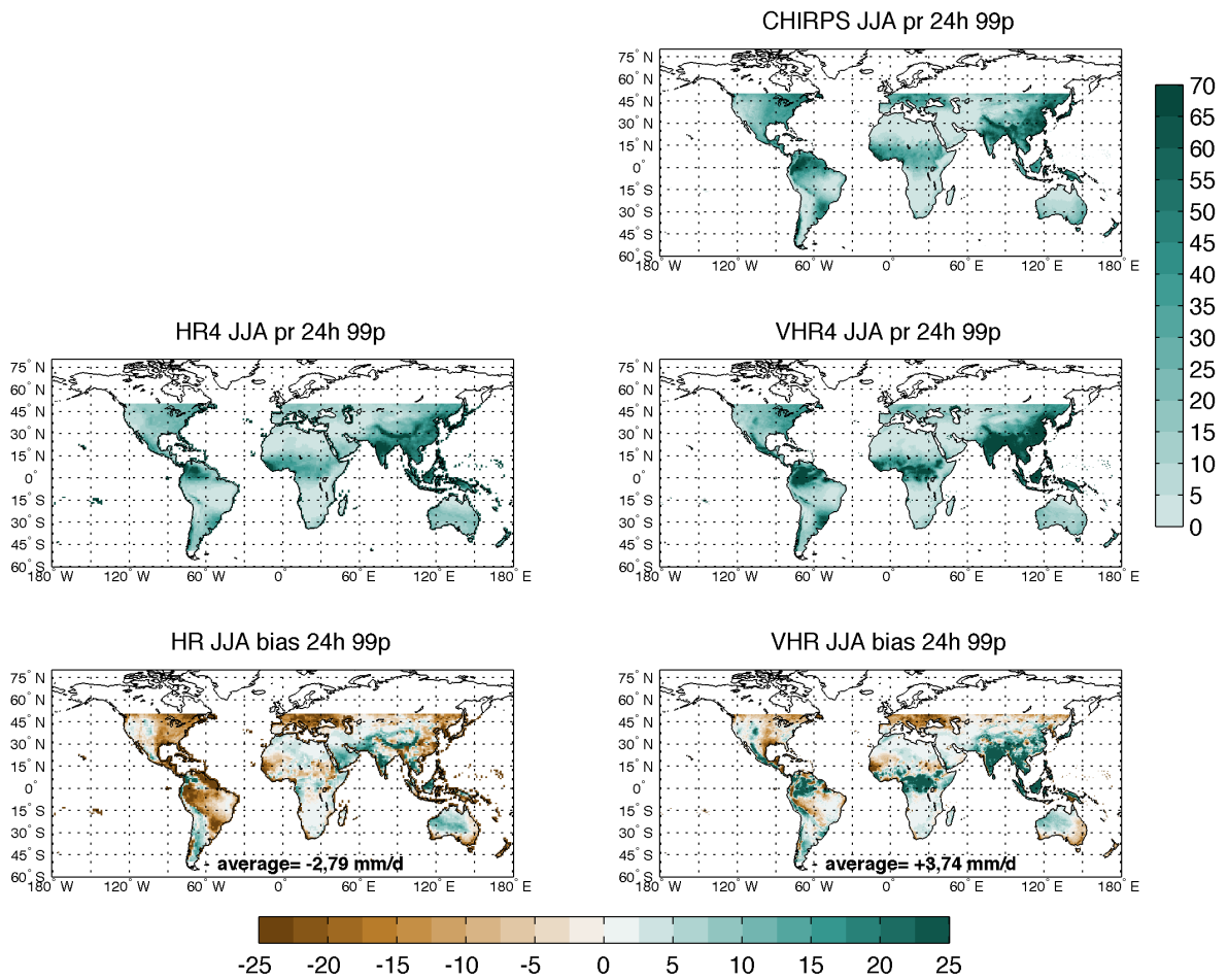
Figure 10: Same as figure 6 but based on CHIRPS observation. Summer (JJA) Extreme Precipitation (99th percentile, 99p) computed at the daily frequency. Upper panel shows CHIRPS observational results. Central panels show model results (HR on the left and VHR on the right) and lower panels show the relative model bias. Units are [mm/d]. Vertical colorbar refers to the three upper panels, while the horizontal colorbar refers to the two bottom panels.
