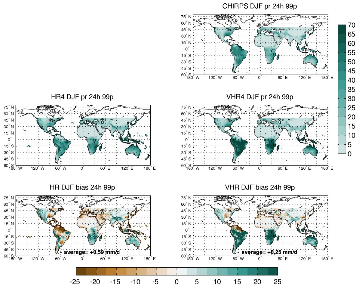
480 Figure 9: Same as figure 5 but based on CHIRPS observations. Winter (DJF) Extreme Precipitation (99th percentile, 99p) computed at the daily frequency. Upper panel shows CHIRPS observational results. Central panels show model results (HR on the left and VHR on the right) and lower panels show the relative model bias. Units are [mm/d]. Vertical colorbar refers to the three upper panels, while the horizontal colorbar refers to the two bottom panels.
