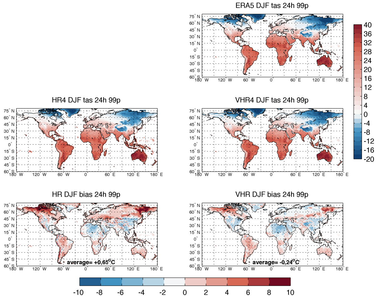
Figure 1: Winter (DJF) Extreme Temperature (99th percentile, 99p) computed at the daily frequency. Upper panel shows ERA5 results. Central panels show model results (HR on the left and VHR on the right) and lower panels show the relative model bias. Units are [°C]. Vertical colorbar refers to the three upper panels, while the horizontal colorbar refers to the two bottom panels.
