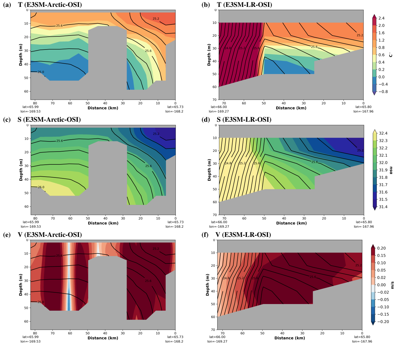
Figure 13. Similar to Fig. 10, but for Bering Strait.
