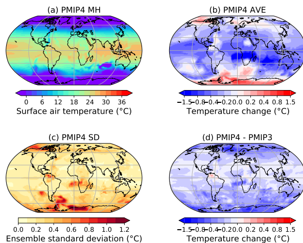
Figure 4. Annual mean surface temperature in the midHolocene simulations ( ^{\circ}\text{C} ). (a) The multi-model mean, mid-Holocene annual mean surface temperature simulated by PMIP4-CMIP6 midHolocene simulations. (b) The multi-model mean, annual mean temperature changes in PMIP4- CMIP6 ( midHolocene – piControl ) and (c) the inter-model spread, defined as the across-ensemble standard deviation. (d) The difference in the multi-model mean, annual mean temperature changes between the PMIP4-CMIP6 and the PMIP3-CMIP5. Panels (a), (b) and (c) are replotted from panels a, b and e in Fig.1 of Brierley et al. (2020) respectively.
