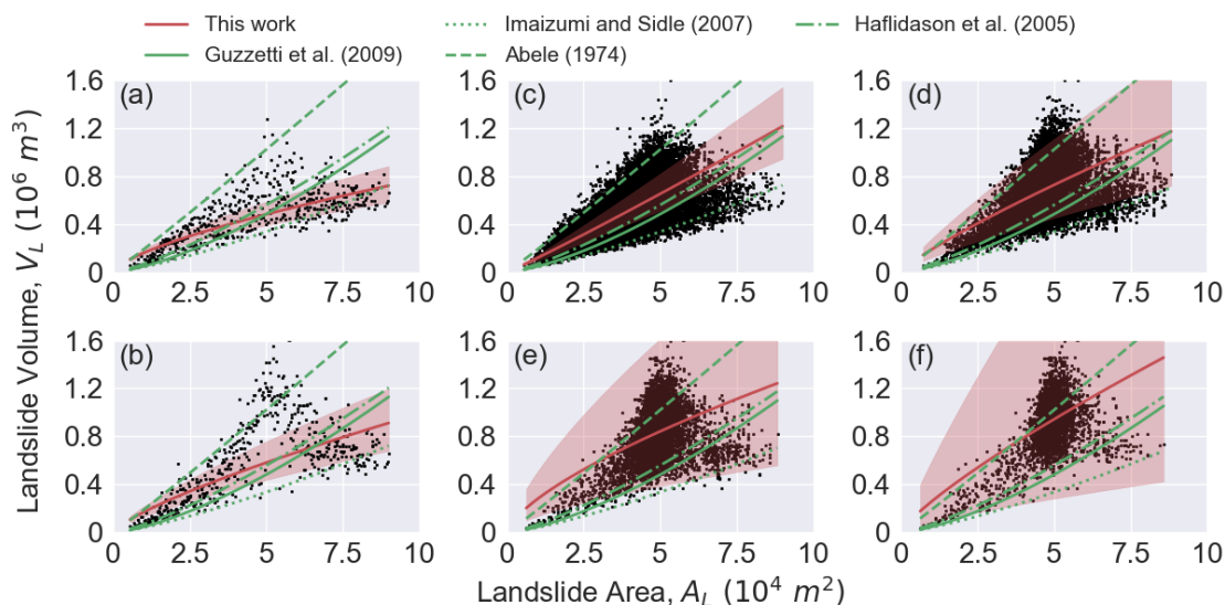
Figure 14: Six sets of source data (ID 1 to 6 in Table 6) are plotted and fitted in this work. All available equations (ID 7 to 10 in Table 6) are plotted by substituting the A_L values in this work. Red zone shows 95% confidence intervals.
