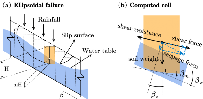
170 Figure 2: Typical longitudinal section of an ellipsoid used as slip surface in iHydroSlide3D v1.0: (a) overall features involved in a potential failure, and (b) forces acting at each column considering the groundwater effect.
