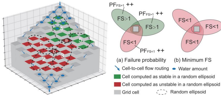
290 Figure 4: Cell-to-cell routing scheme and potential landslides generated across the grid in the iHydroSlide3D v1.0 model: (a) and (b) illustrate the definitions of PF and FS within the framework, respectively.
