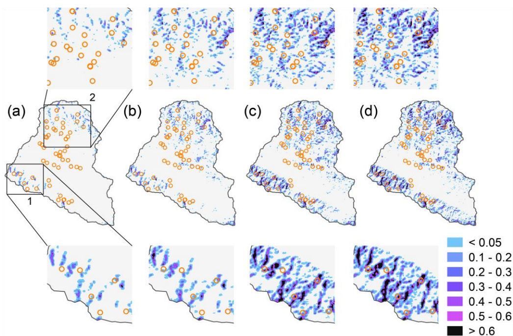
505 Figure 10: Spatiotemporal evolutions of the landslide occurrence probability. (a)–(d) are four moments that span the complete rainfall event.
