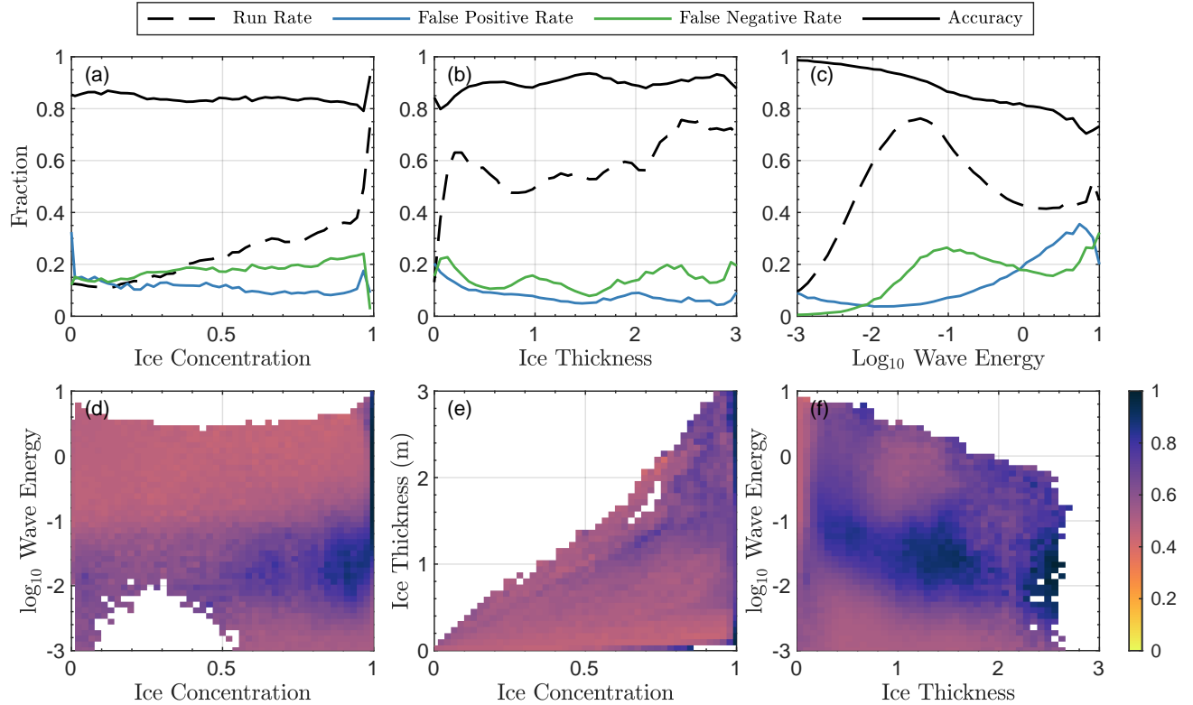
Figure 1. Performance of Input Classification for NN-WIFF (a) Percentage of times the classifier runs (run rate, dashed black), calls the histogram network incorrectly (false positive rate, blue), or fails to call the histogram network (false negative rate, green), and overall accuracy (black) for input classifier as a function of sea ice concentration. (b,c) Same as (a) for (b) sea ice thickness and (c), \log_{10} wave energy. (d-f) Heat map of average classifier accuracy as a function of (d) ice concentration and \log_{10} wave energy, (e) ice concentration and ice thickness, and (f) ice thickness and \log_{10} wave energy. Regions of phase space with fewer than 75 input vectors (less than 0.005% of input data) are uncolored/empty.
