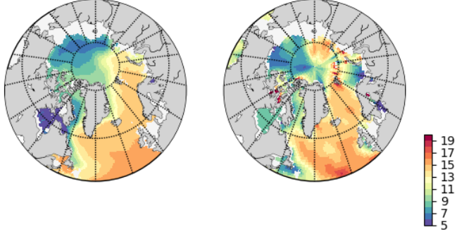
Fig. A4: Simulated and WOA2013 inorganic nutrients annual averages \text{NO}_3/\text{PO}_4 molar ratios, a) model, b) WOA2013 for 5 and 100 meters isodepth.
