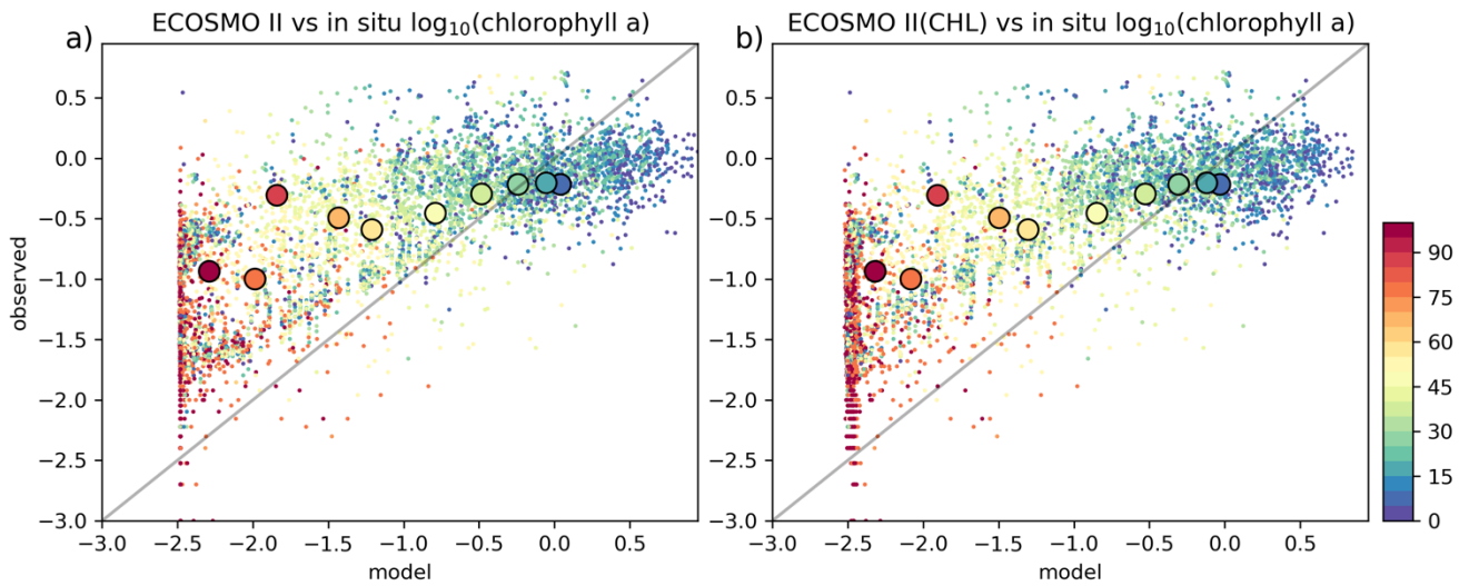
615 Fig. A2: (a) ECOSMO II and (b) ECOSMO II(CHL) 1D model chlorophyll a ( \log_{10}(\text{mg m}^{-3}) ) is evaluated against in situ data at Station-M. Model data was interpolated to co-locate with the in situ data. Small markers depict the individual points and the large markers depict 10 meter interval averages. The observation depth is given in color coding.
