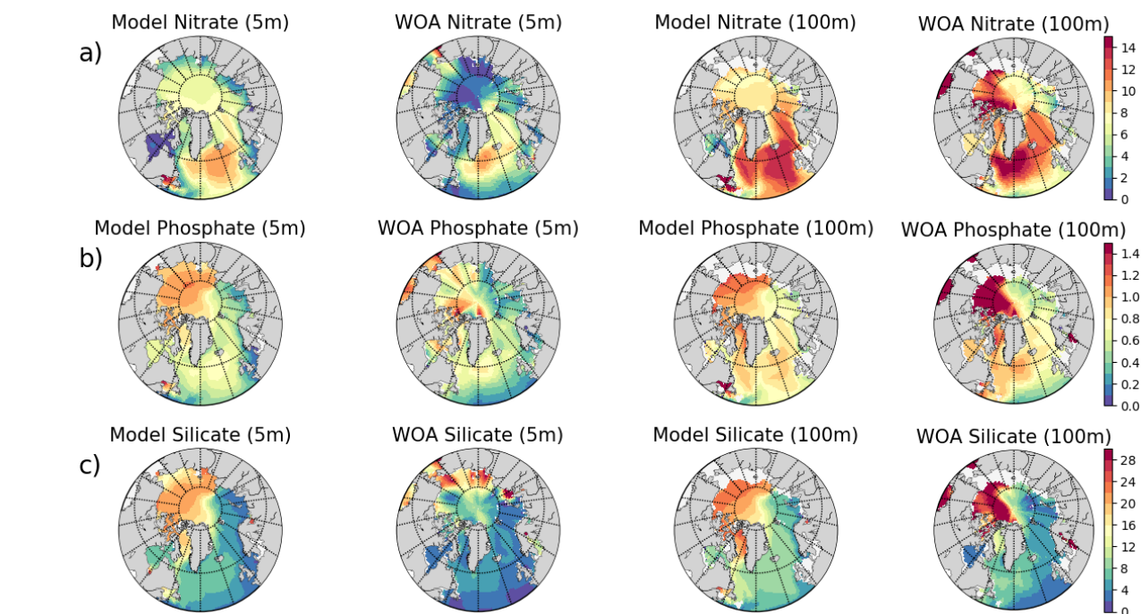
Fig. 8: Simulation averaged (EXP1; \text{mmol m}^{-3} ) (a) nitrate, (b) phosphate and (c) silicate for 5 and 100 meters depth and corresponding WOA2013 annual climatologies.
