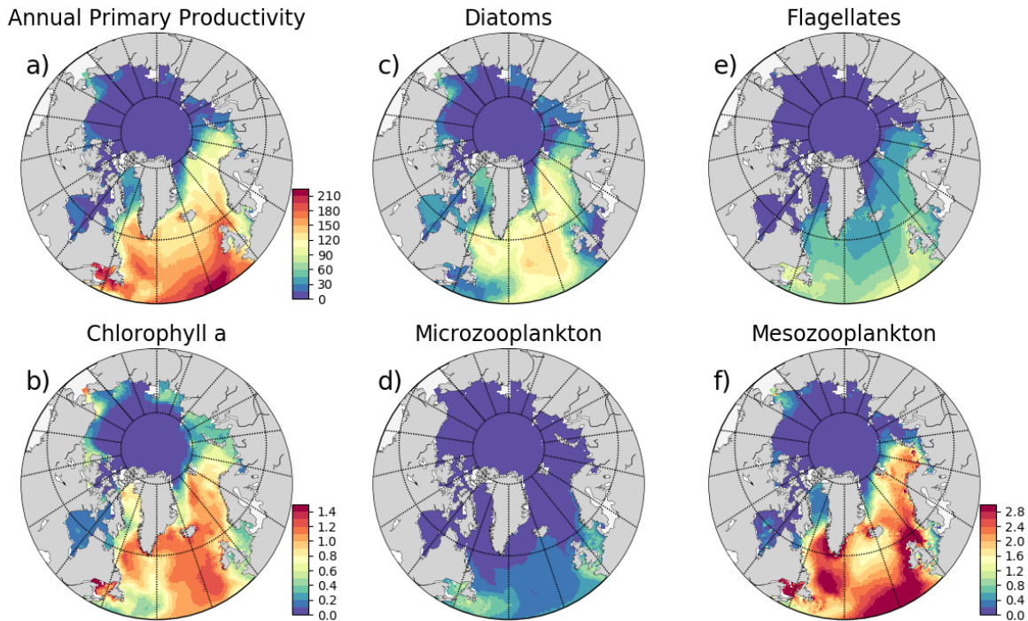
445 Fig. 5: Simulation averaged (EXP1) model results; (a) vertically integrated (0–200 m) annual primary production ( \text{gC m}^{-2} \text{y}^{-1} ), (b) annually averaged surface chlorophyll a ( \text{mg m}^{-3} ), and simulation averaged vertically integrated (0–200 m) plankton functional type biomass ( \text{gC m}^{-2} ) (c) diatoms, (d) microzooplankton, (e) flagellates, (f) mesozooplankton. The colorbar to Figure f applies to Figures c, d, e and f.
