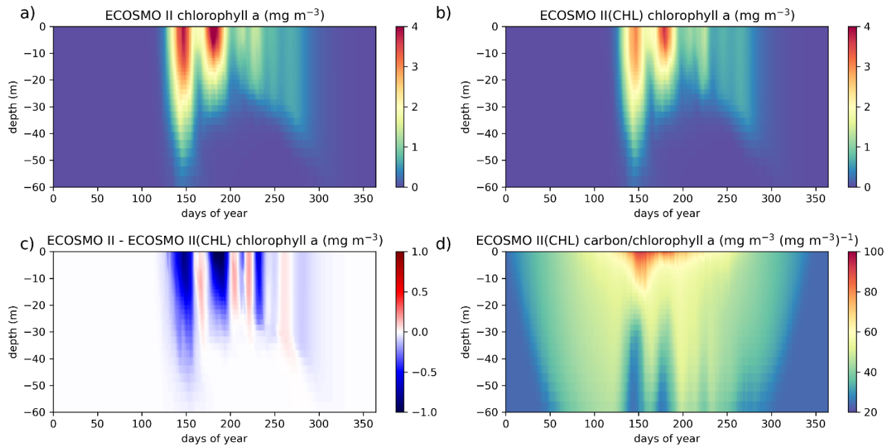
605 Fig. A1: ECOSMO II chlorophyll a seasonal evolution is compared to ECOSMO II(CHL) using a 27-year (1990 – 2016) 1D simulation at Station-M (66°N 2°E) in the Norwegian Sea. Results provided here are the averages of the last 22 years (1995 – 2016) of the simulations given as annual climatologies. Figures a and b depict chlorophyll a concentrations of ECOSMO II and ECOSMO II(CHL) respectively, c depicts the chlorophyll a difference of the 2 simulations, and d depict the diatom and flagellate averages of carbon:chlorophyll a ratios.
