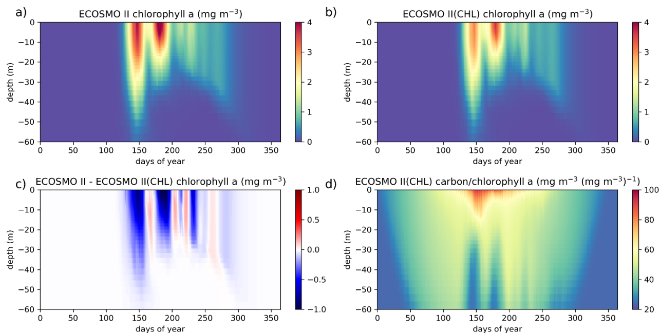
620 Fig. A1: ECOSMO II chlorophyll a seasonal evolution is compared to ECOSMO II(CHL) using a 27-year (1990 – 2016) 1D simulation at Station-M (66°N 2°E) in the Norwegian Sea. Results provided here are the averages of the last 22 years (1995 – 2016) of the simulations given as annual climatologies. Figures a and b depict chlorophyll a concentrations of ECOSMO II and ECOSMO II(CHL) respectively, c depicts the chlorophyll a difference of the 2 simulations, and d depict the diatom and flagellate averages of carbon:chlorophyll a ratios.
