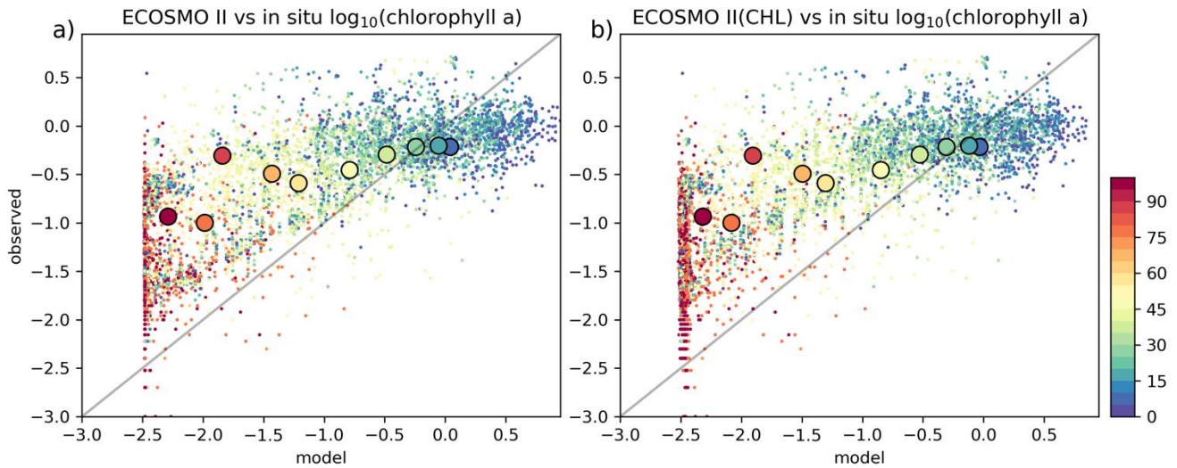
630 Fig. A2: (a) ECOSMO II and (b) ECOSMO II(CHL) 1D model chlorophyll a ( \log_{10}(\text{mg m}^{-3}) ) is evaluated against in situ data at Station-M. Model data was interpolated to co-locate with the in situ data. Small markers depict the individual points and the large markers depict 10 meter interval averages. The observation depth is given in color coding.
