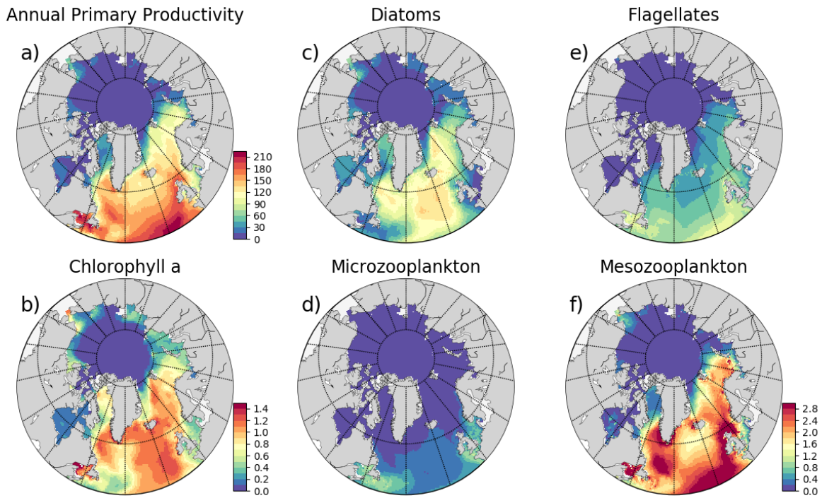
460 Fig. 5: Simulation averaged (EXP1) model results; (a) vertically integrated (0–200 m) annual primary production ( \text{gC m}^{-2} \text{y}^{-1} ), (b) annually averaged surface chlorophyll a ( \text{mg m}^{-3} ), and simulation averaged vertically integrated (0–200 m) plankton functional type biomass ( \text{gC m}^{-2} ) (c) diatoms, (d) microzooplankton, (e) flagellates, (f) mesozooplankton. The colorbar to Figure f applies to Figures c, d, e and f.
