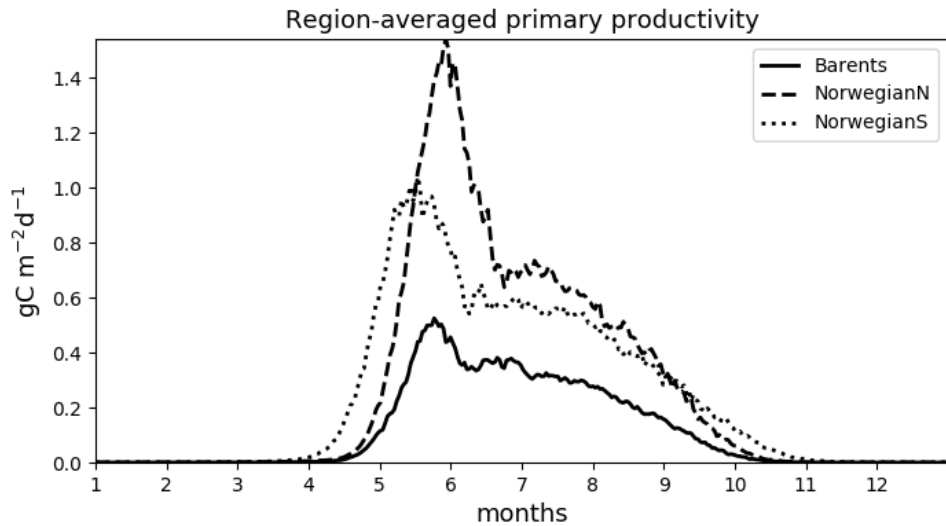
465 Fig. 6: Simulated (EXP1) time-series of 0-200 m integrated primary productivity ( \text{gC m}^{-2} \text{d}^{-1} ) for different regions: (a) Barents, (b) NorwegianN and (c) NorwegianS. See Table 3 for annually averaged primary productivities.
