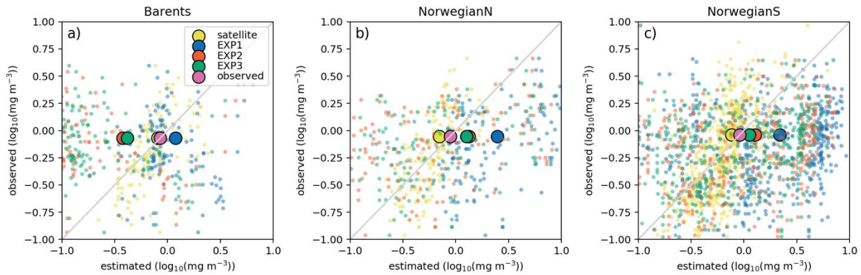
565 Fig. 9: Estimated surface chlorophyll a data against in situ observations ( \log_{10}(\text{mg m}^{-3}) ). Region-wide averages are depicted with the large markers representative of the individual points depicted with the same colors in the background with smaller-sized markers.
