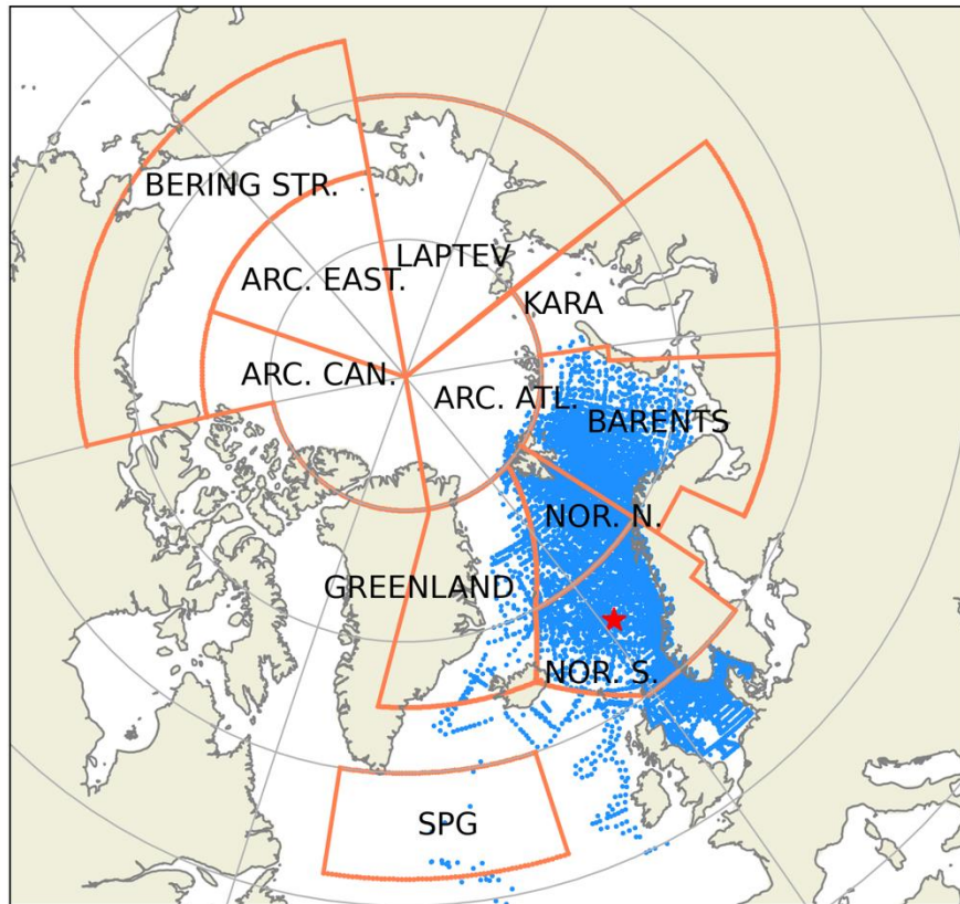
645 Fig. A5: Subdivision of model domain in prescribed geographical subdomains used for model quality assessments. The subdomains are as follows: Norwegian Sea South (NOR. S.), Norwegian Sea North (NOR. N.), Barents Sea (BARENTS), Kara Sea (KARA), Laptev Sea (LAPTEV), Bering Strait (BERING STR.), Arctic-Canada (ARC. CAN.), Arctic-East (ARC. EAST), Arctic-Atlantic (ARC. ATL.), Greenland Sea (GREENLAND) and the Subpolar Gyre (SPG). The points in the oceanic regions denote the profile 650 locations for the observed biogeochemical variables that were used for the statistical analyses. The star depicts the coordinates of the Station-M time-series location. While the model domain extends down to the equatorial regions, the figure focuses on the area of interest. Note that the BERING STR. subdomain is within the effective area of the open boundary conditions thus is relaxed to climatology.
