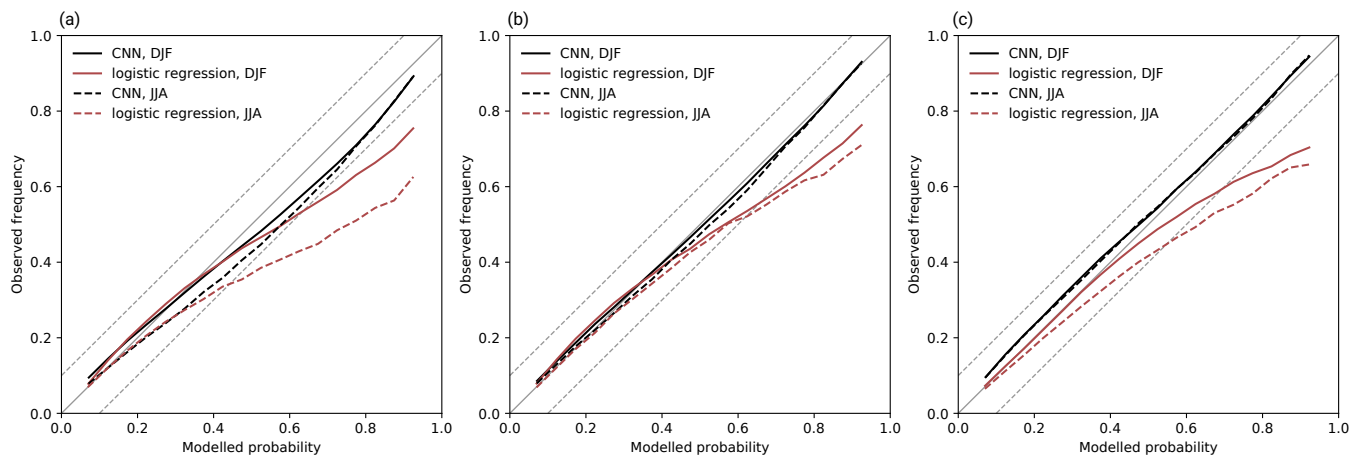
Figure 3. Reliability diagrams for (a) inflow, (b) ascent, and (c) outflow during DJF (solid lines) and JJA (dashed lines). The black curves represent the reliability of the CNN models and the red curves represent the reliability of the logistic regression models (Quinting and Grams, 2021). Modelled probabilities (x-axis) and observed frequencies (y-axis) are binned into 19 bins based on the modelled probabilities. The perfect modelled probability and a \pm 10\% interval about the perfect model is shown by the solid and dashed gray diagonals, respectively.
