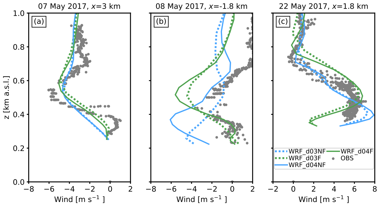
Figure 7. Vertical profiles of the wind speed parallel to the cross sections (see Figs. 6, 8, 9) during the low-level-Jet (LLJ) events for both simulations (colour lines) and Lidar observations (grey dots). Panel a) presents the first LLJ event (07 May 2017 04:00:00 ) on the leeward side of the topography ( x = 3\text{km} ). Panel b) presents the second LLJ event (08 May 2017 05:30:00 ) on the lee side of the topography ( x = -1.8\text{km} ). Panel c) presents the third LLJ event (22 May 2017 04:00:00 ) on the leeward side of the topography ( x = 1.8\text{km} ).
