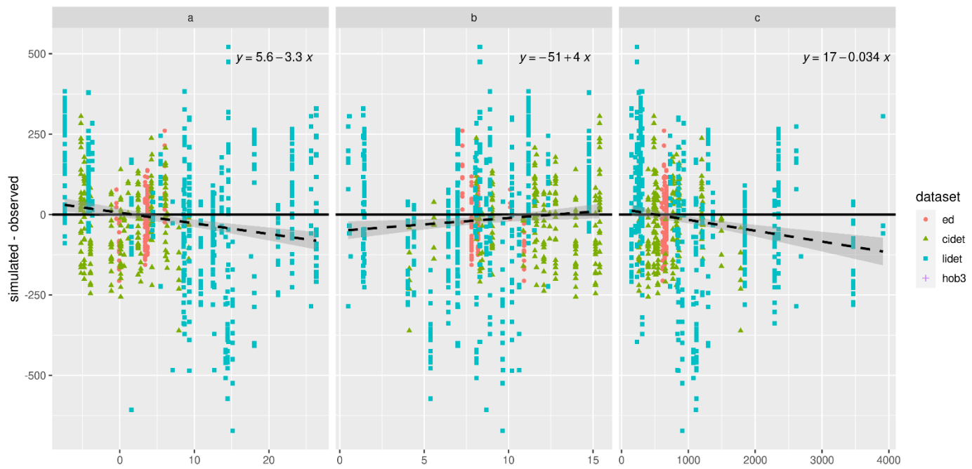
925 Figure 7: Residual analysis between simulated and observed carbon remnant on a) mean temperature (C), b) temperature variation (C) and c) total precipitation ( \text{mm y}^{-1} ) at the validation site.
