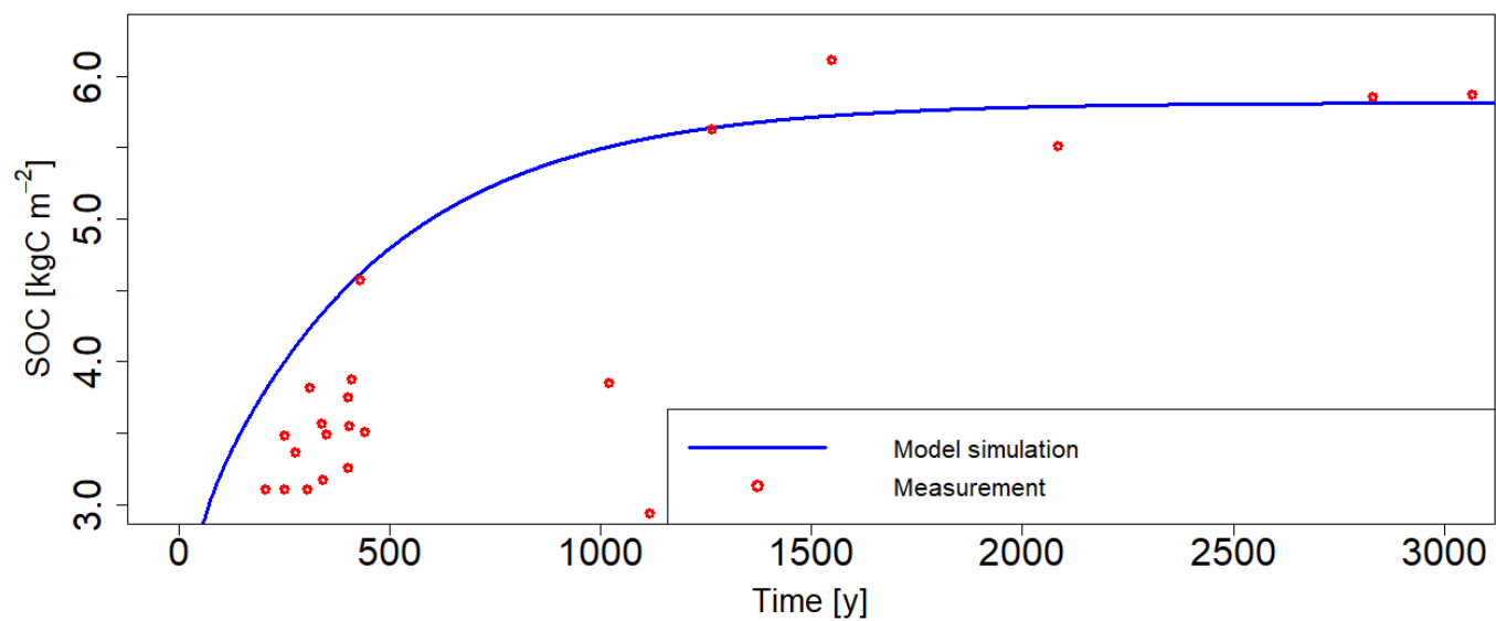
Figure 5: Measurement (Red dots) and model (Blue line) based projections of SOC accumulation on the Finnish coast after the end of ice age.
