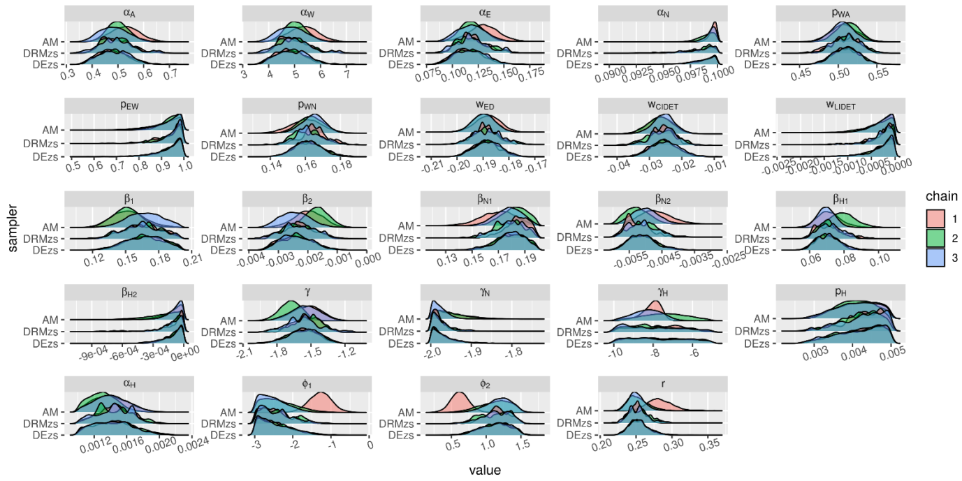
895 Figure 1: The global calibration results with the different calibration methods.
