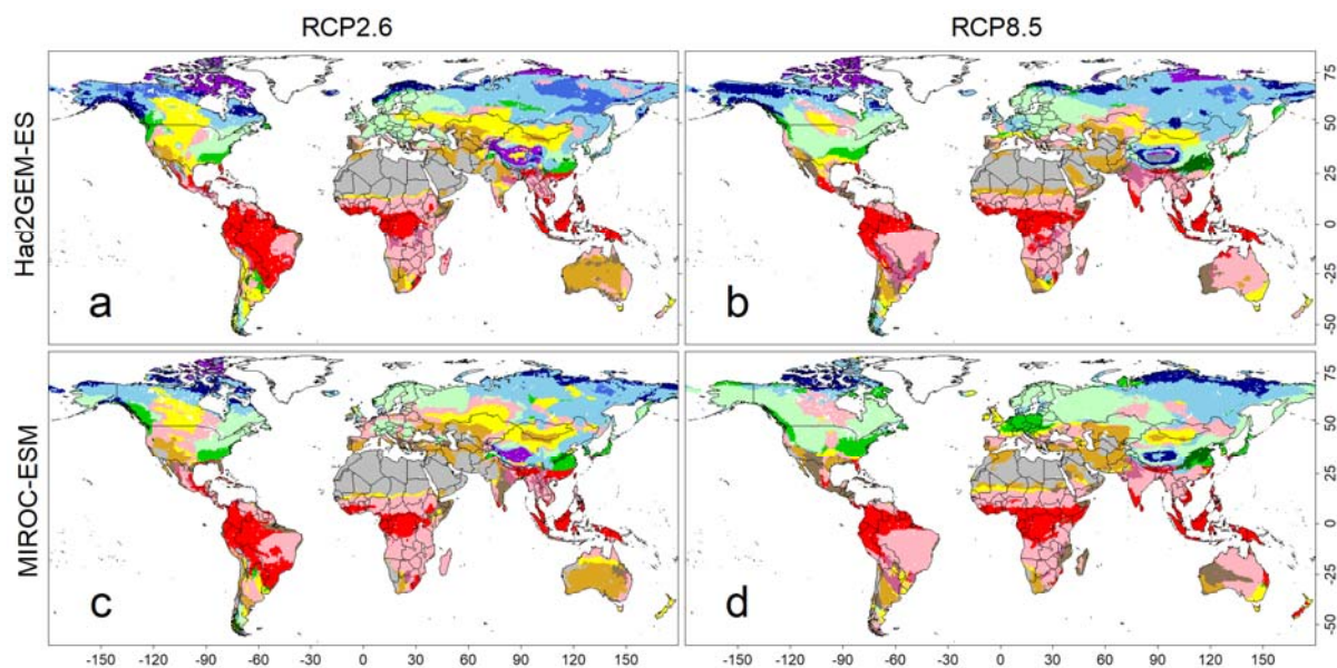
Figure 5: Predicted biome maps under climatic scenarios from 2091 to 2100. Monthly means of four sets of forecasted climatic conditions derived from combinations of two climate models (i.e., Had2GEM-ES and MIROC-ESM) and two RCP scenarios (i.e., RCP2.6 and RCP8.5). These means were applied to the CNN model that was trained by the current biome distribution map, as well as the present climatic condition derived from the CRU dataset. Colour definitions are available in Figure 1.
