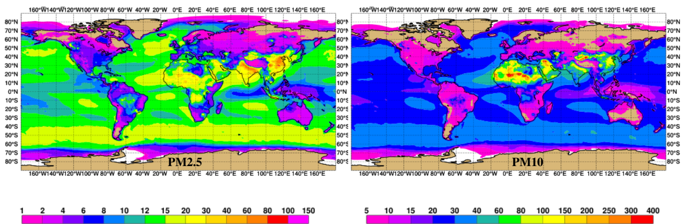
Figure 3. Global mean 2017 PM 2.5 (left) and PM 10 (right) in \mu\text{g}/\text{m}^3 simulated by the CY47R1_NEWDEP experiment in cycling forecast mode. Please note the different scale for PM 2.5 and PM 10 .
