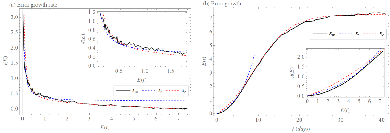
530 Figure 3. (a) Error growth rate \lambda_{tot}(E) of the L05-3 system (black). Quadratic model \lambda_r(E) (Eq. (22)) with \alpha = 0.25 (day -1 ) and \beta = 0.13 (units/day) ( \lambda_{tot,p}(E) , blue, dashed) and extended quadratic model \lambda_q(E) (Eq. (20)) with \alpha = 0.2 (day -1 ), the coefficient \beta = 0.19 (units/day), and E_\infty = 7.3 (units) ( \lambda_{q,w}(E) , red, dashed) that approximate \lambda_{tot}(E) . (b) Error growth E_{tot}(t) (Eq. (17)) (black), solution E_{tot,r}(t) (blue, dashed) of \lambda_{tot,r}(E) (Eq. (22)), and solution E_{tot,q}(t) (red, dashed) of \lambda_{tot,q}(E) (Eq. (21)) (red, dashed).
