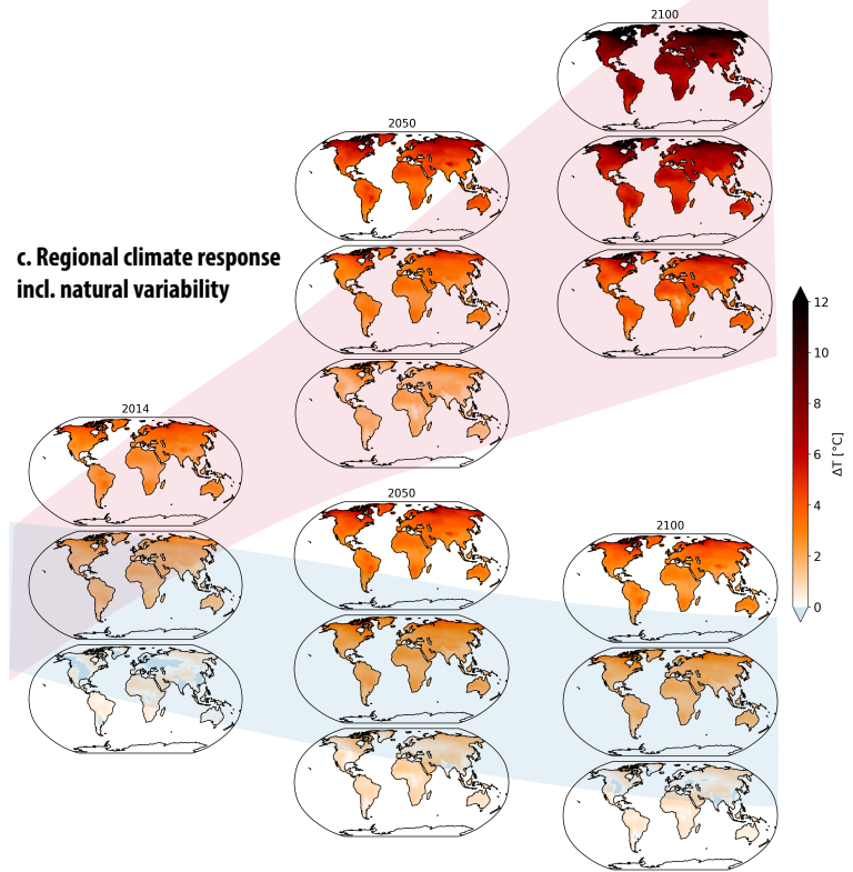
Figure 1. Illustration of the MAGICC-MESMER emulator chain. (a) The sequence of the analysis starts from either an emission or a concentration scenario, as highlighted here for the CO 2 concentration time series of the historical time period and two Shared Socioeconomic Pathway (SSP) scenarios (O’Neill et al., 2017), namely SSP1-1.9 and SSP3-7.0. (b) The probabilistic global mean temperature change distributions – whose medians and 90 % ranges (5th–95th percentile) are shown – consist of realizations which are a combination of the scenario-specific forced global warming from MAGICC and emulated global natural variability from MESMER. (c) Based on this information, MESMER can derive the associated spatially resolved temperature change distributions, with the maps shown here representing the 5th percentile, the median, and the 95th percentile (each map trio from bottom to top) for 2014 (first column of maps), for 2050 for both SSP scenarios (second column of maps), for and 2100 for both SSP scenarios (third column of maps).
