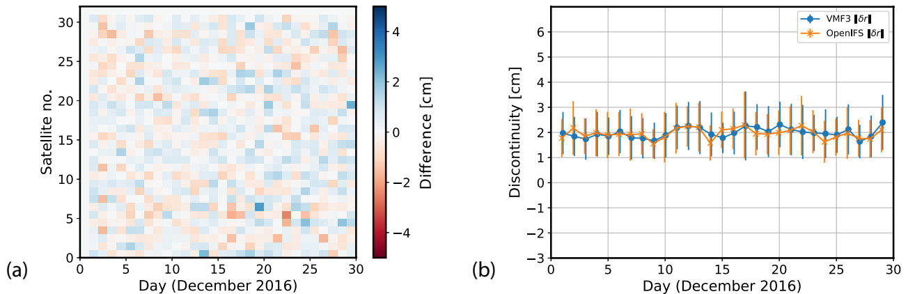
Figure 1. Norm of the midnight discontinuity ( \|\delta\mathbf{r}\| ) for December 2016. (a) A color map representing the difference between the default and experimental system for the satellites used in the experiment; (b) The mean (solid lines) and standard deviation (vertical whiskers) over all satellites for each day of the experiment with blue (default system) and orange (experimental system).
