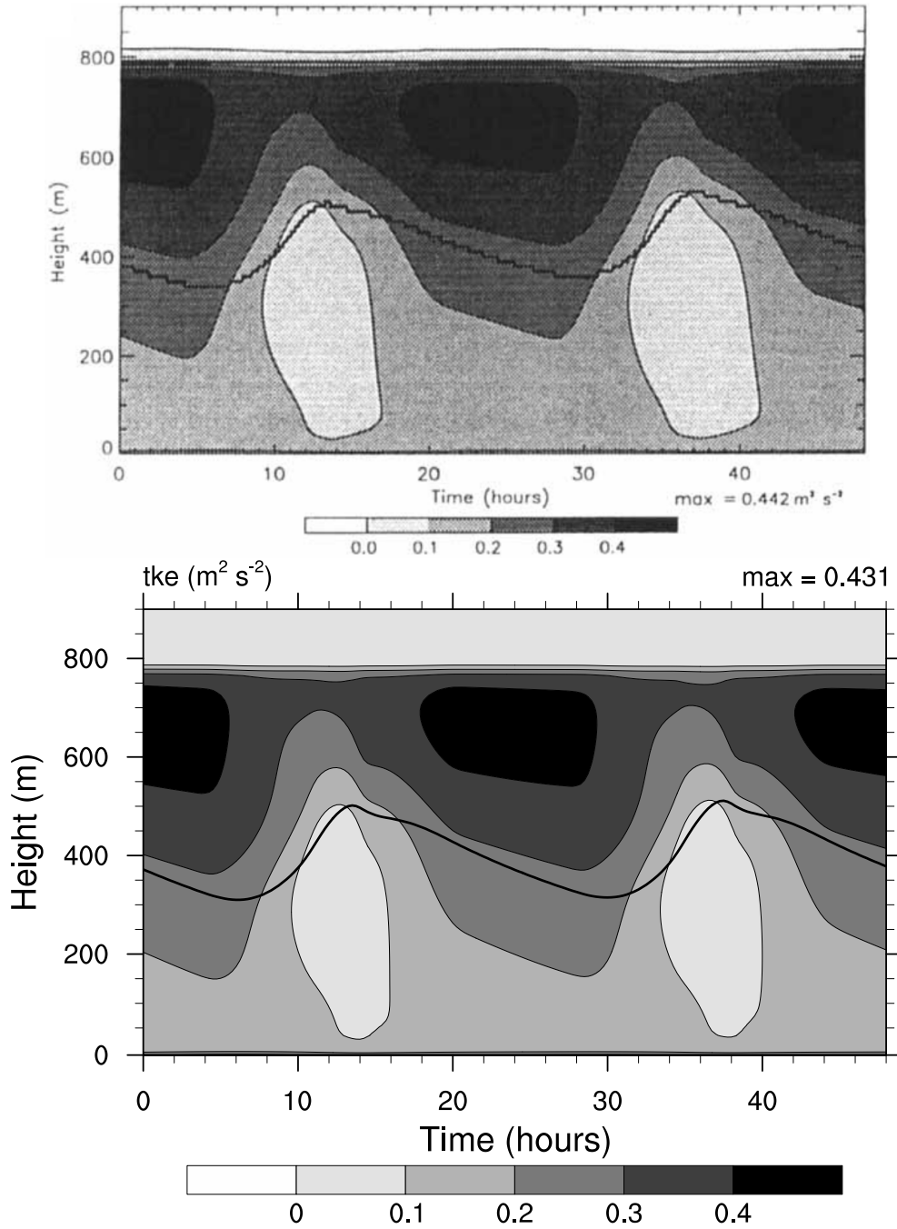
Figure 4. Contour plot of turbulent kinetic energy (in \text{m}^2 \text{s}^{-2} ) as a function of height and simulation time. The thick line shows the bottom of cloud, defined as LWC dropping below 0.01 \text{ g kg}^{-1} . Top: study from Loughlin et al. (1997, Fig. 4a). Bottom: MISTRA-v9.0. For both, the simulation settings are identical to those in Bott et al. (1996). Top panel reproduced with permission from Loughlin et al. (1997, Fig. 4a). Copyright (1997) by John Wiley and Sons.
